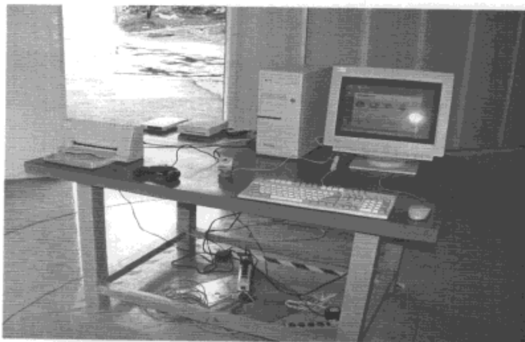
BACK VIEW OF RADIATED TEST ( Worst Case Test Setup)
