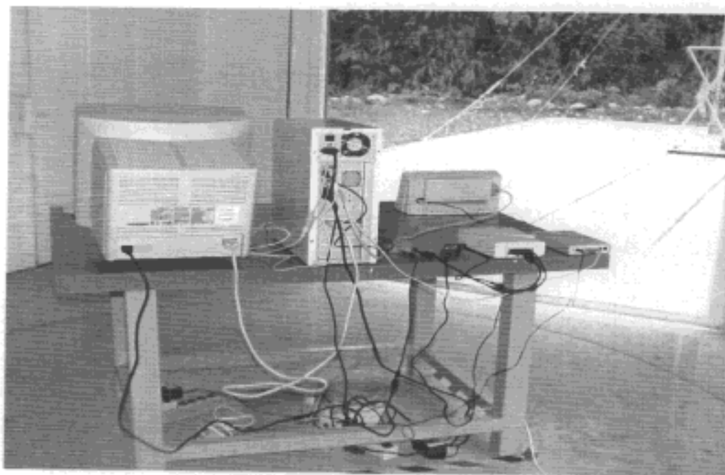
BACK VIEW OF RADIATED TEST ( Worst Case Test Setup)
