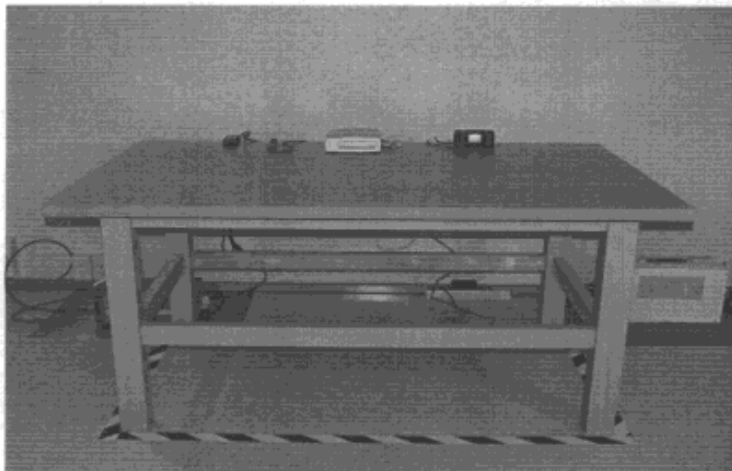
BACK VIEW OF CONDUCTED TEST ( Worst Case Test Setup)
