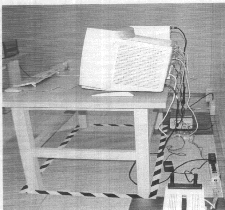
BACK VIEW OF CONDUCTED TEST ( Worst Case Test Setup, mode 1)
