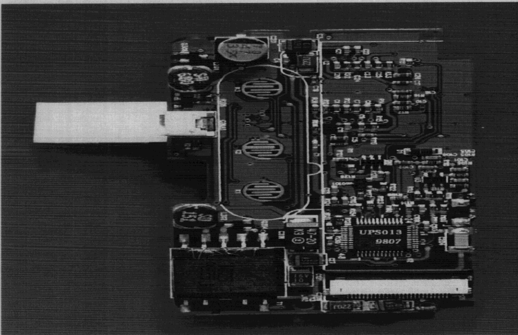
Solder Side of EUT
