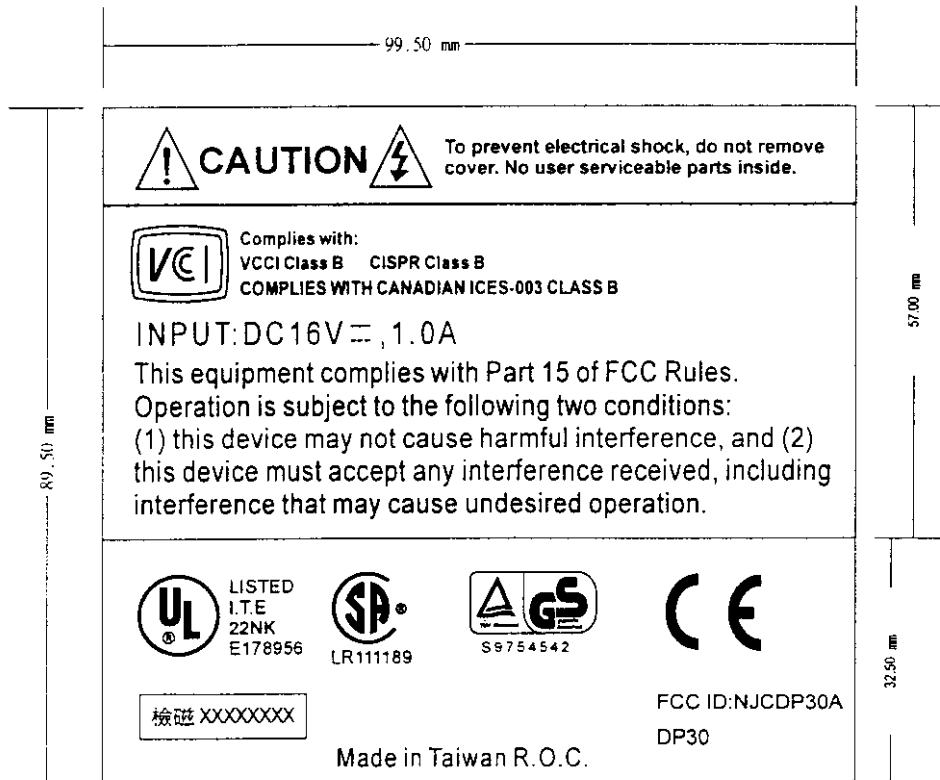
( The Proposed FCC ID Label )
