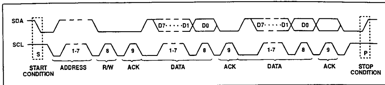
Fig.19 I 2 C Data transfer
