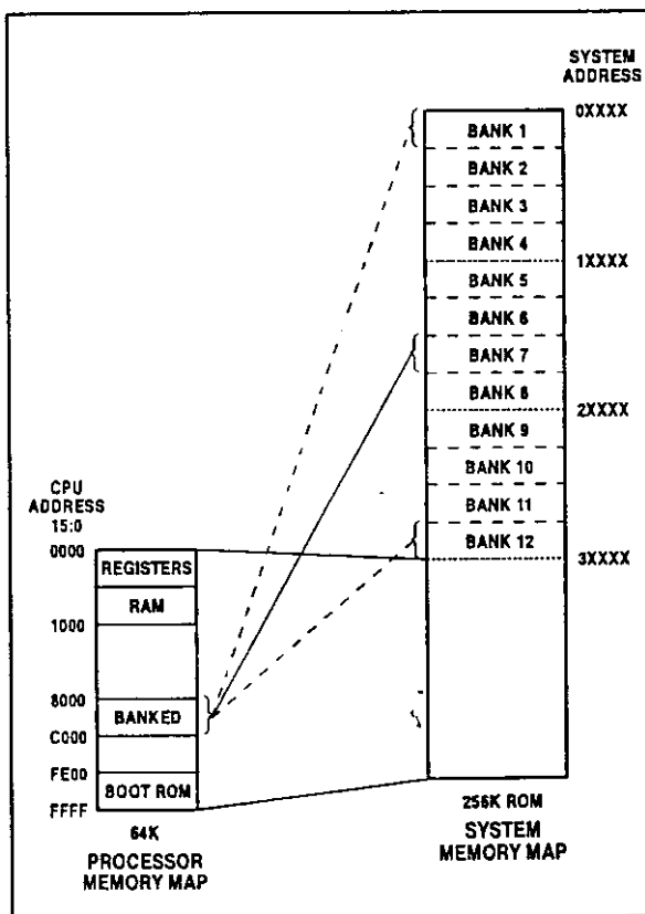
Fig. 15 Memory Map and Banked Addressing
