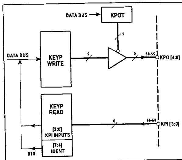
Fig. 25 Keypoint configuration
