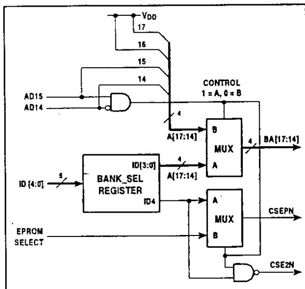
Fig. 14 Banked Addressing block diagram
