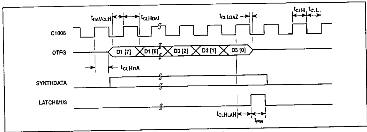
Fig.9 ACEBus Transmit timing diagram
