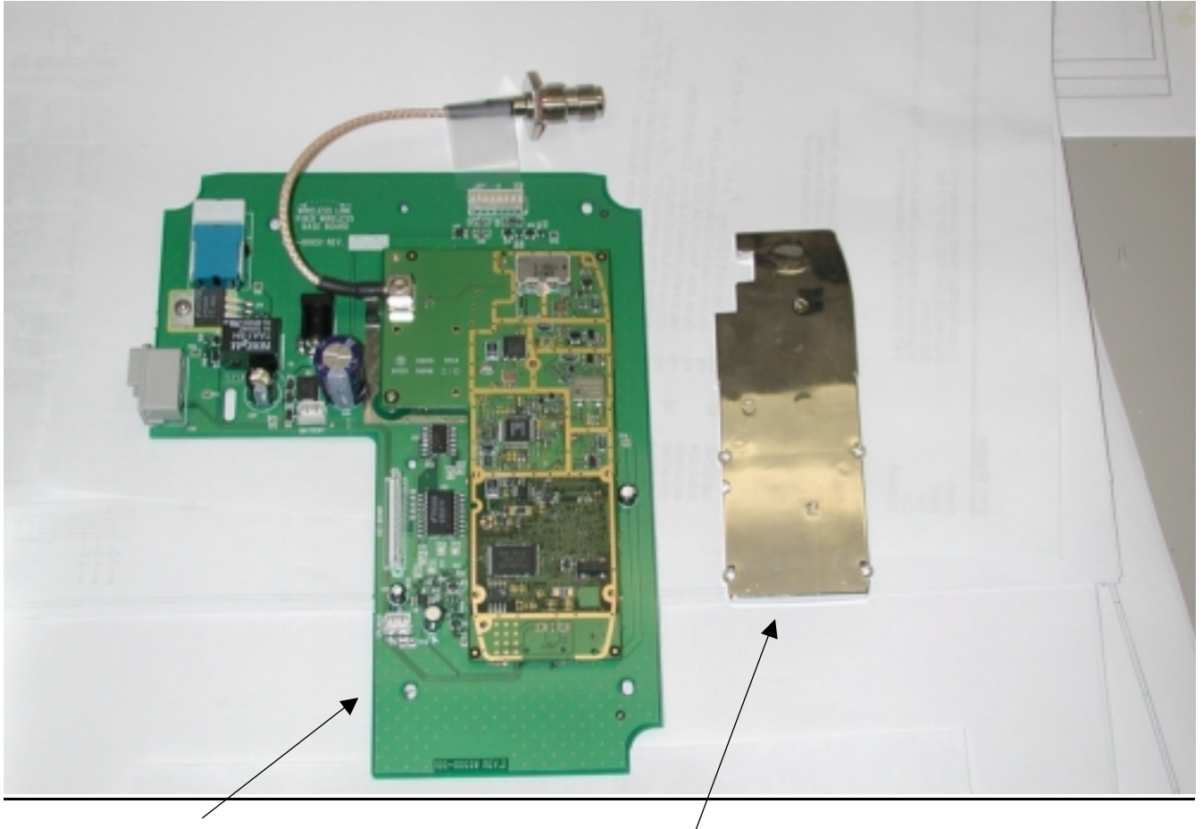
Base and RF / Baseband PCB Assemblies
