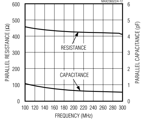
IF/IN DIFFERENTIAL PORT INPUT IMPEDANCE
