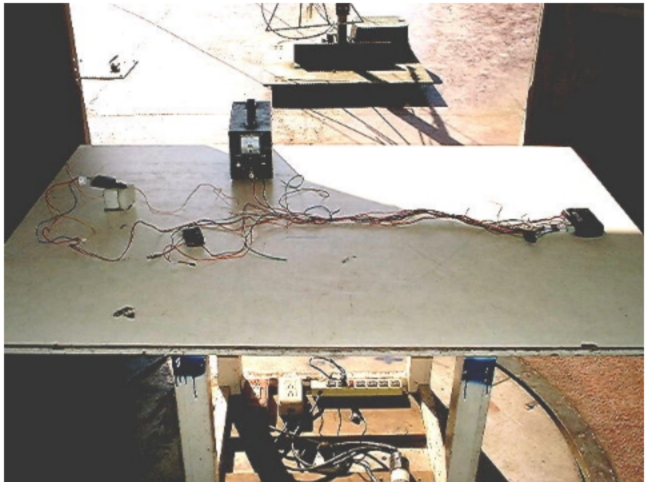
01E9251 Setup Photos ( RX-Front ) 4 of 5
