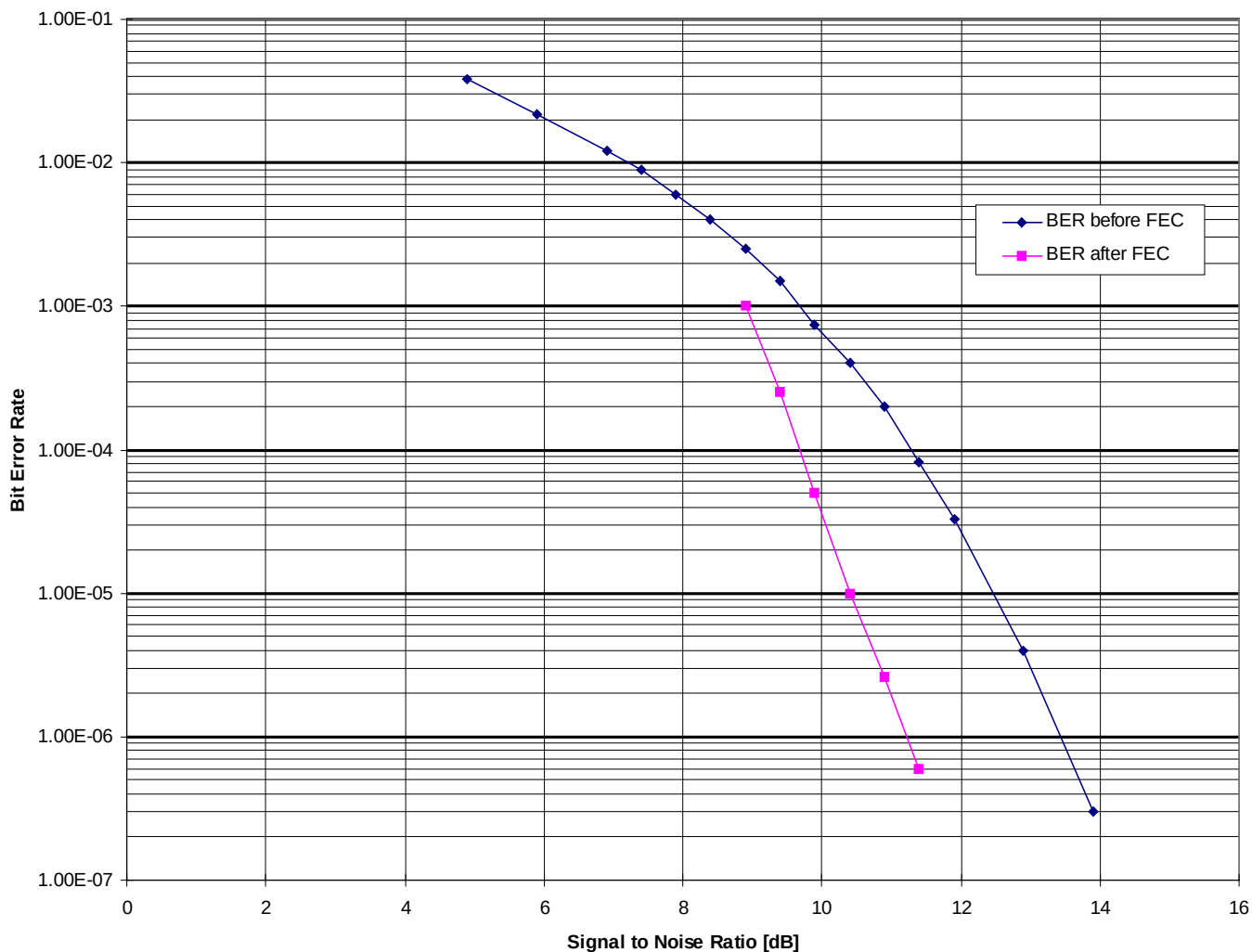
Figure 2-7. Forward Error Correction (FEC) Improvement of Bit Error Rate (BER) for Differential Quadrature Phase Shift Keying (DQPSK)
