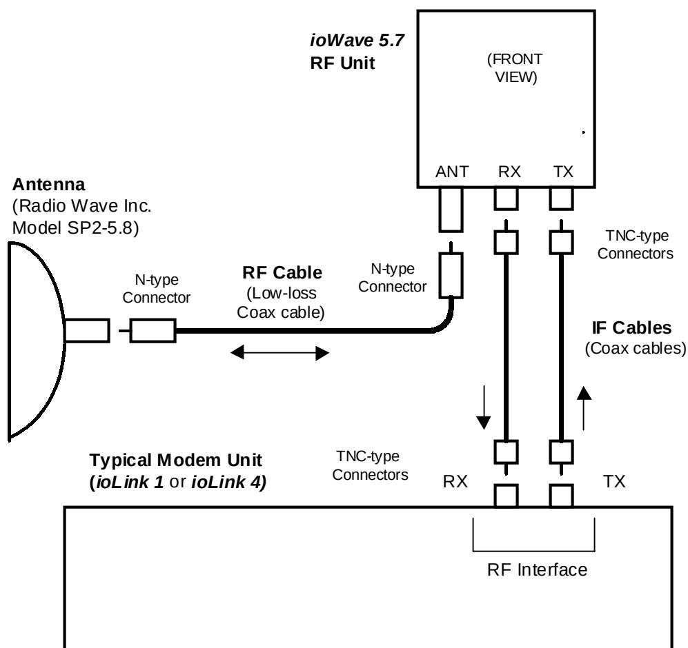
Figure 1-3. ioWave 5.7 RF Unit System Overview
