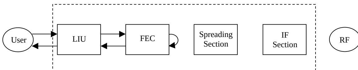
Figure 3-5. FEC Loopback
