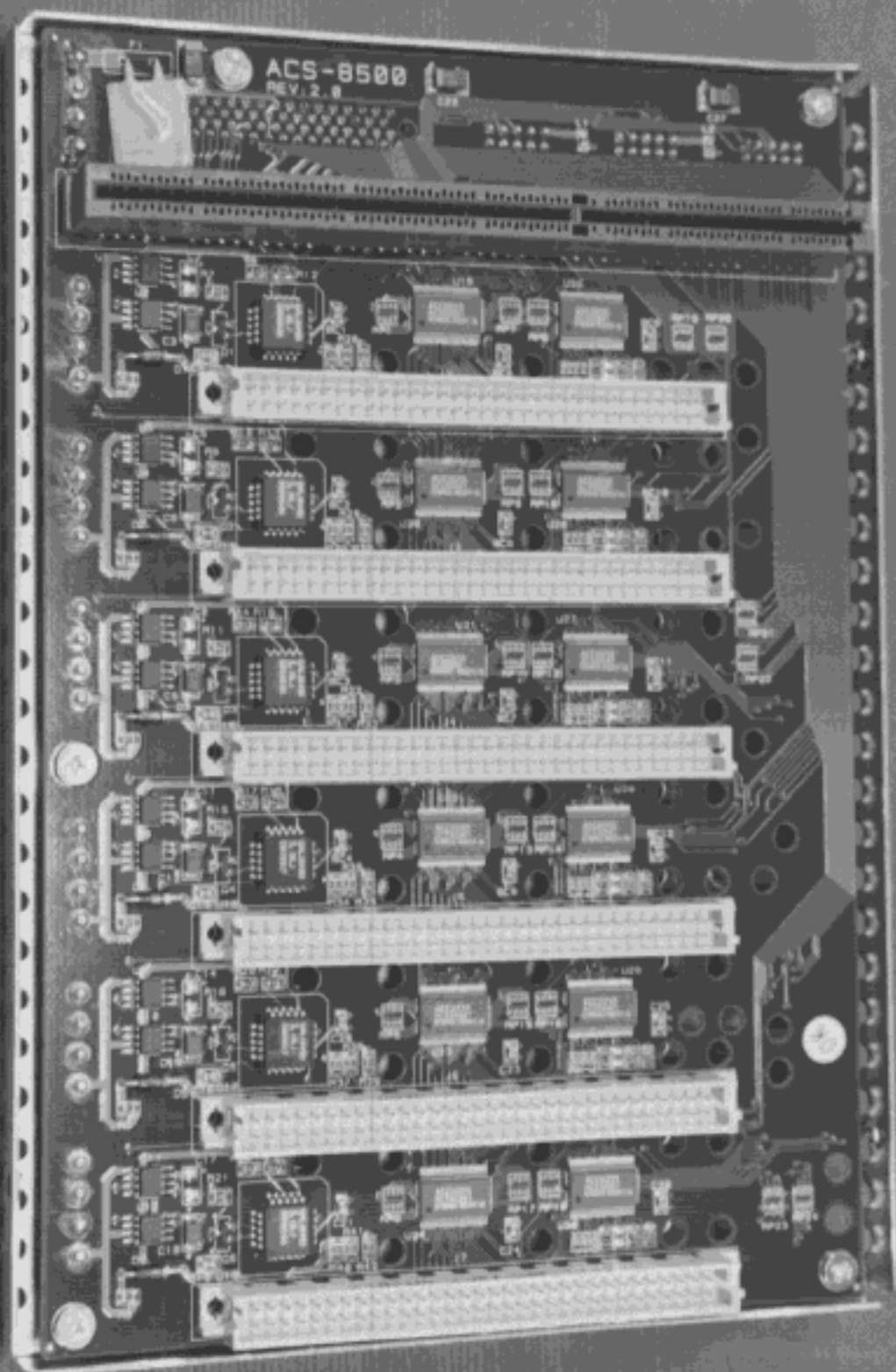
PHOTO 6. EUT COMPONENT SIDE VIEW
