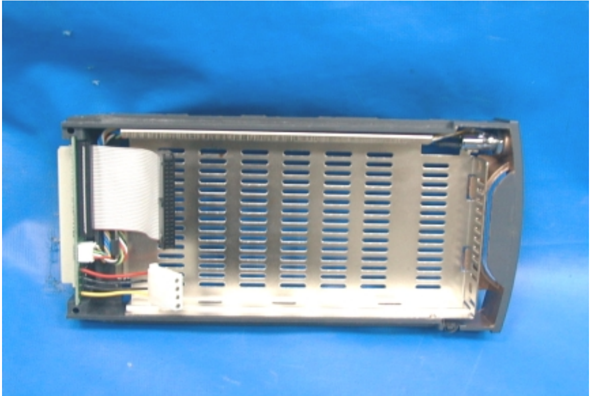
PHOTO. 9. HARD DISK CHASSIS FRONT VIEW
