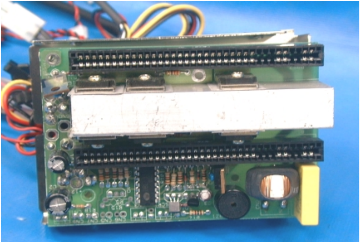
PHOTO. 22. POWER SUPPLY COMPONENT SIDE VIEW
