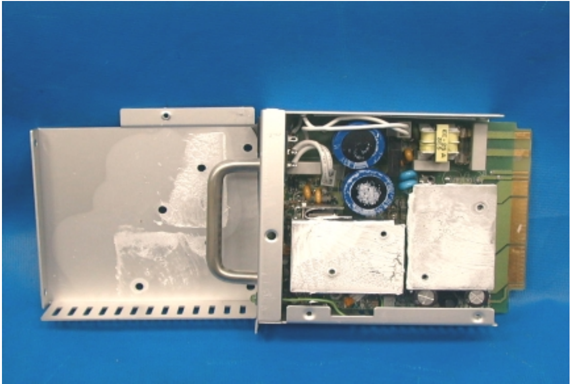
PHOTO. 28. POWER SUPPLY COMPONENT SIDE VIEW
