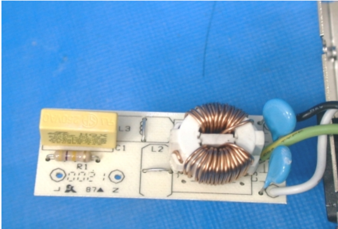
PHOTO. 29. POWER SUPPLY COMPONENT SIDE VIEW
