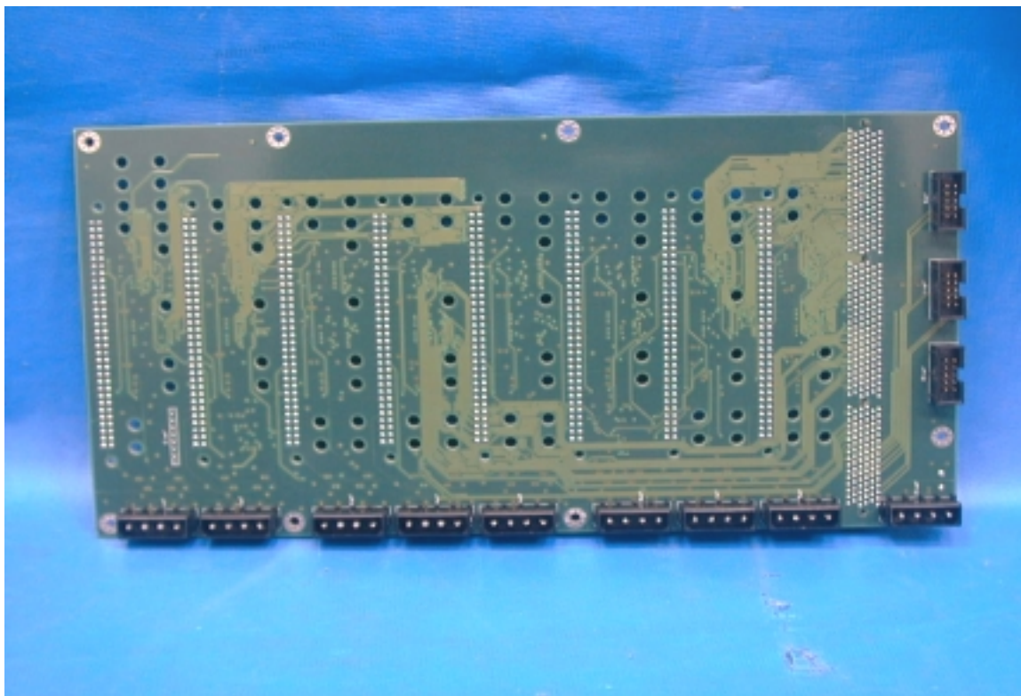
PHOTO. 18. EUT COMPONENT SIDE VIEW
