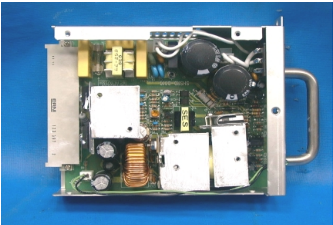
PHOTO. 26. POWER SUPPLY INSIDE VIEW
