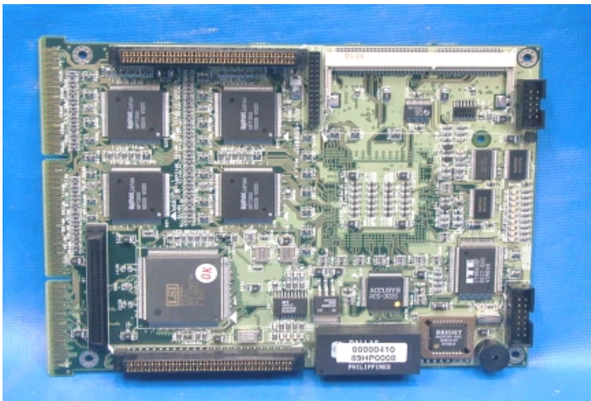
PHOTO. 12. ENU COMPONENT SIDE VIEW
