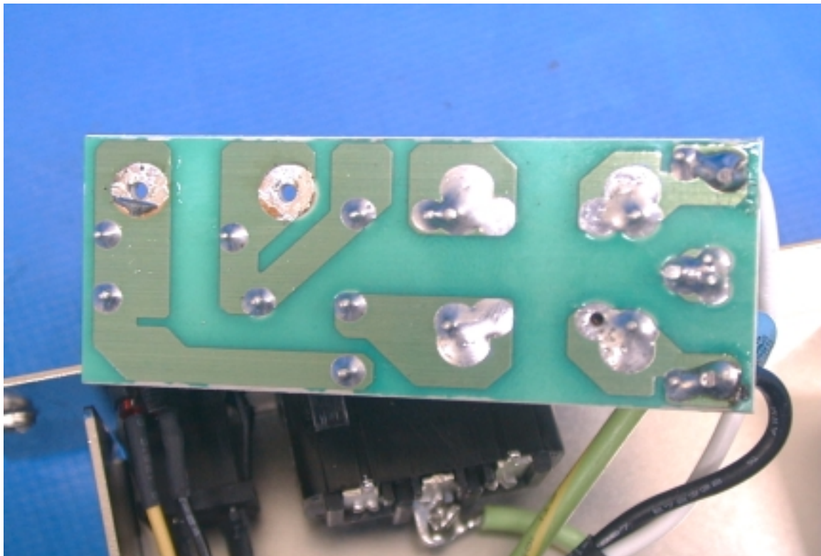
PHOTO. 30. POWER SUPPLY SOLDERING SIDE VIEW
