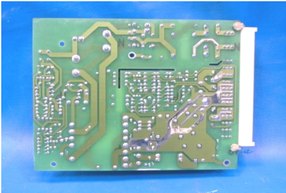
PHOTO. 28. POWER SUPPLY SOLDERING SIDE VIEW
