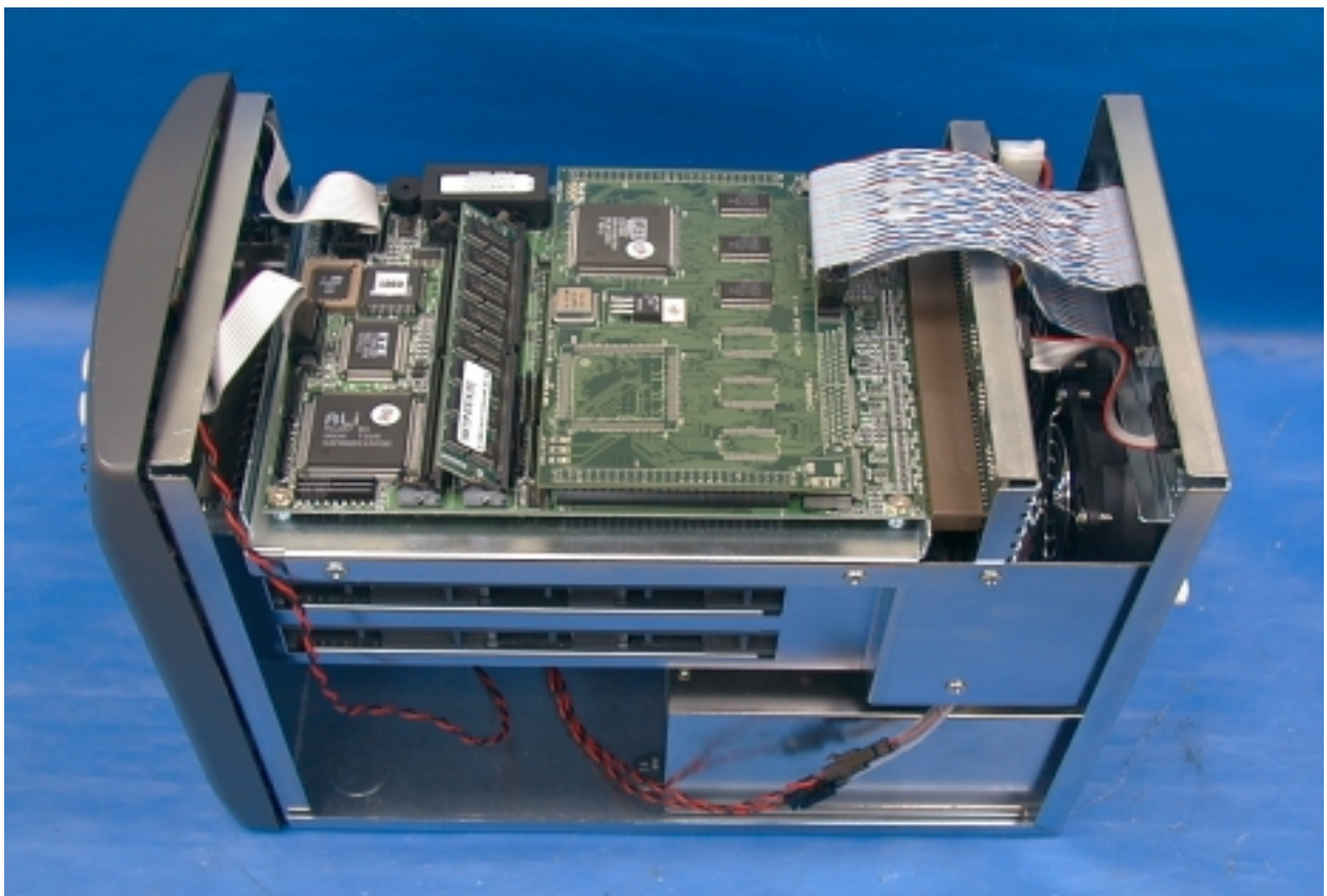
PHOTO. 4. EUT INSIDE VIEW
