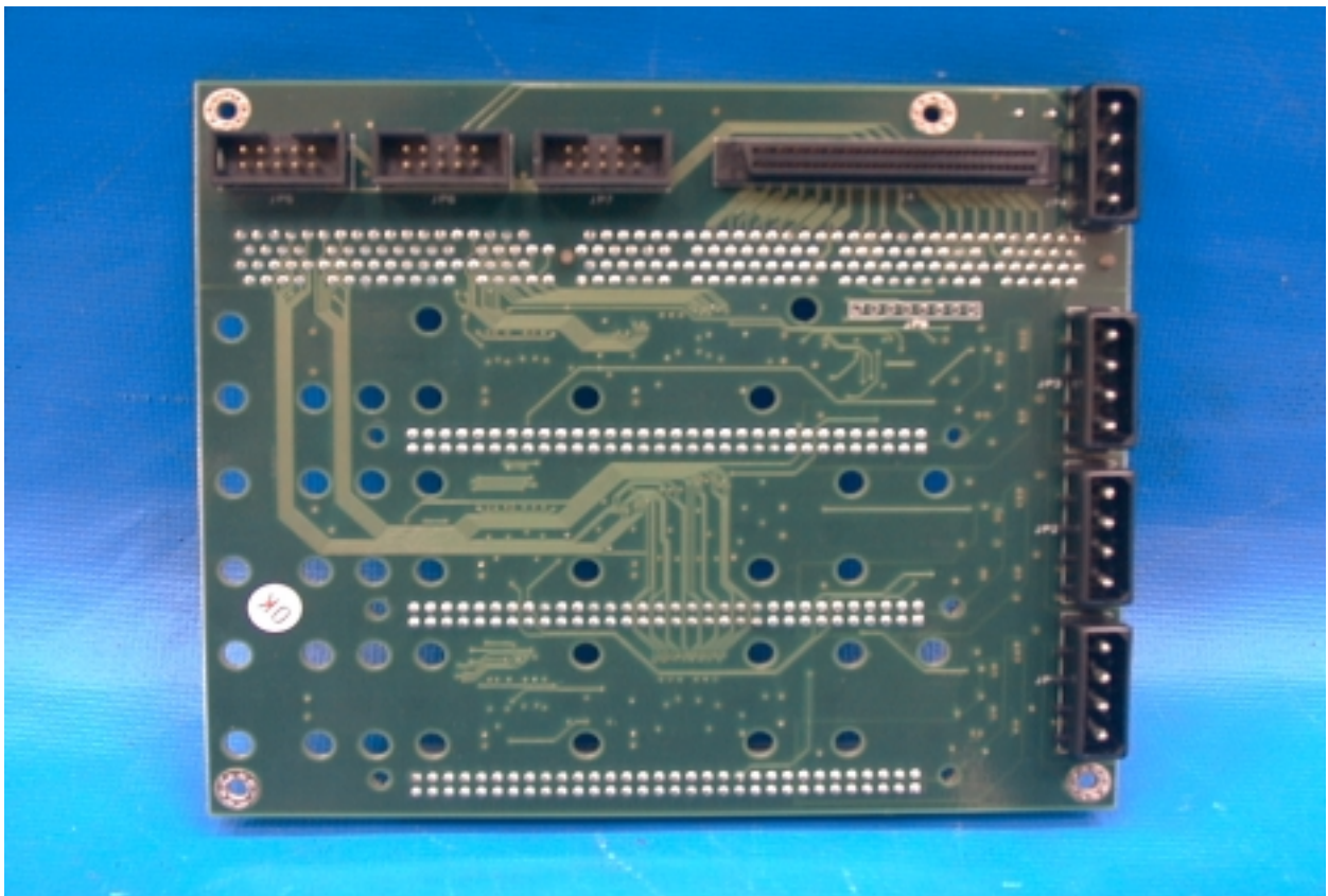
PHOTO. 12. EUT SOLDERING SIDE VIEW
