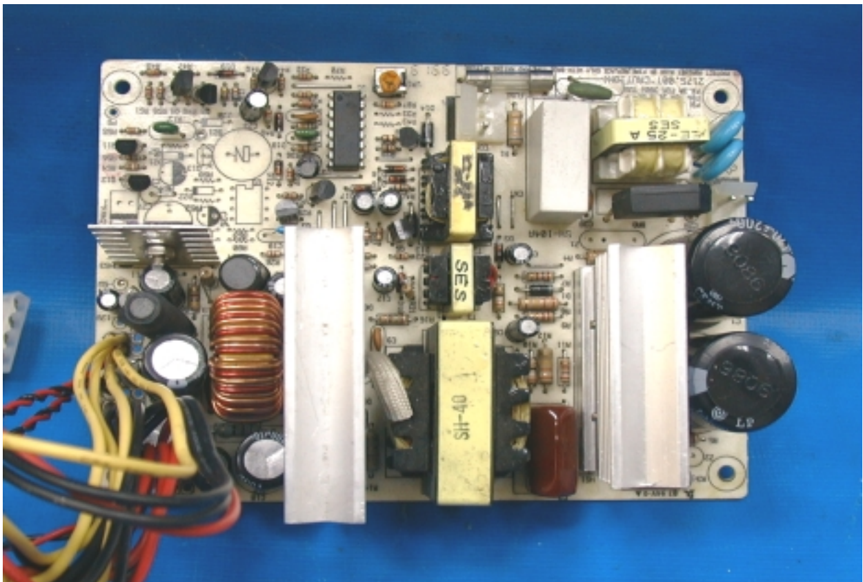
PHOTO. 20. EUT COMPONENT SIDE VIEW
