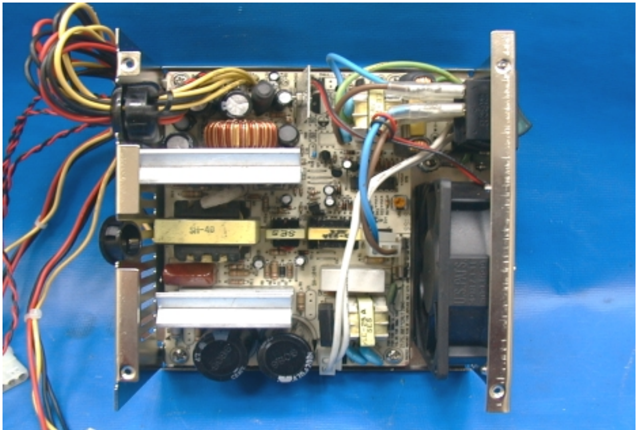
PHOTO. 19. EUT COMPONENT SIDE VIEW
