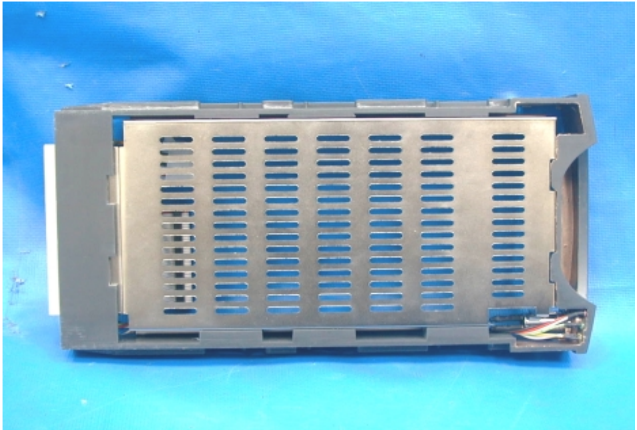
PHOTO. 19. HARD DISK CHASSIS REAR VIEW
