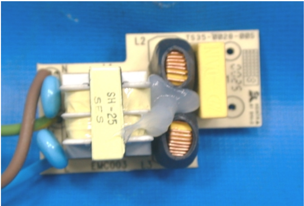
PHOTO. 13. POWER SUPPLY COMPONENT SIDE VIEW
