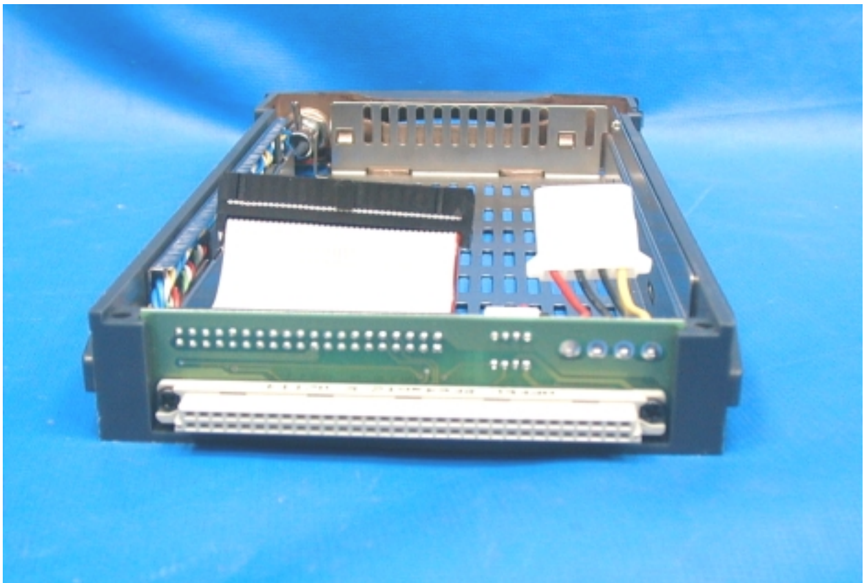
PHOTO. 20. HARD DISK CHASSIS INSIDE VIEW
