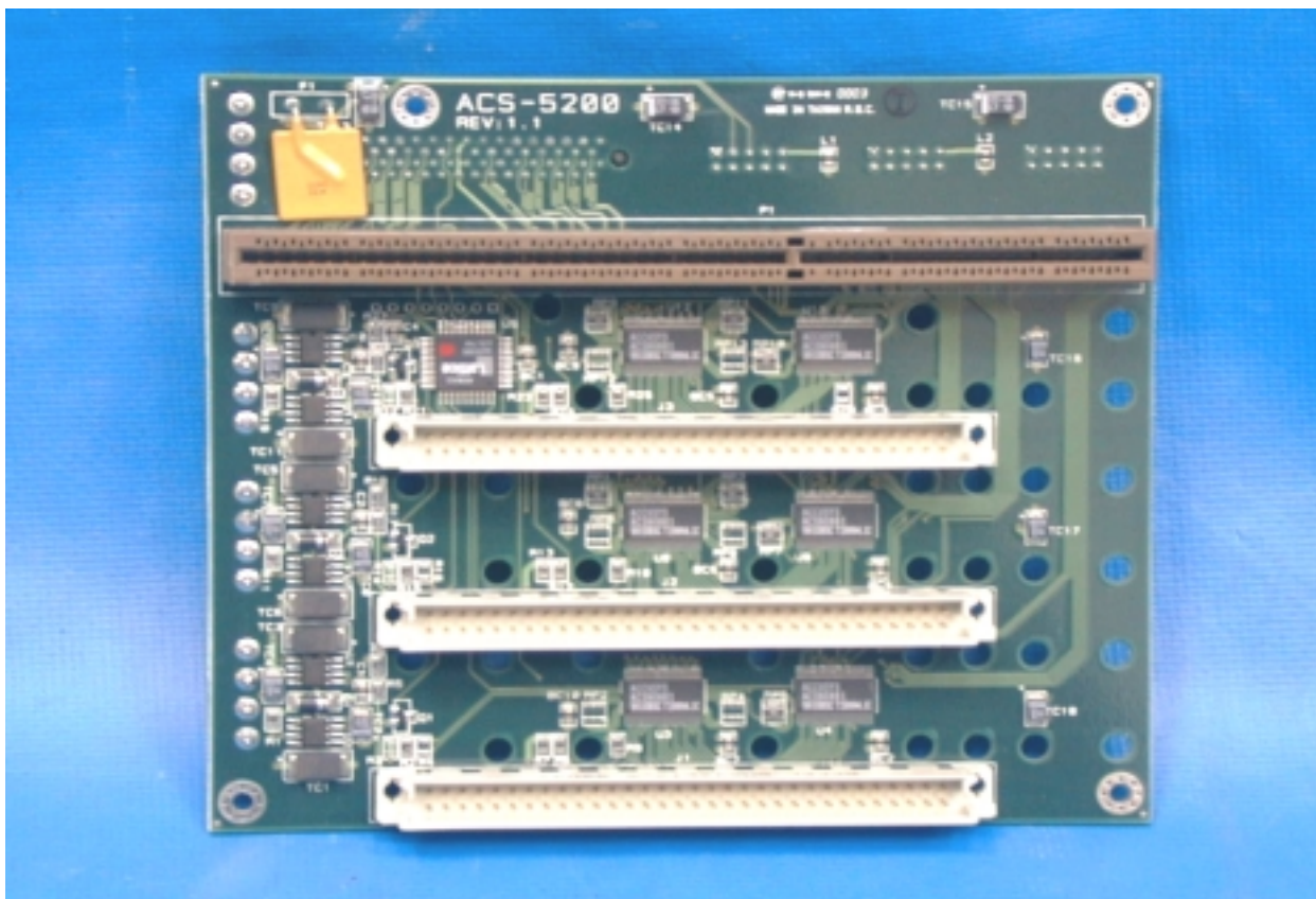
PHOTO. 5. EUT COMPONENT SIDE VIEW
