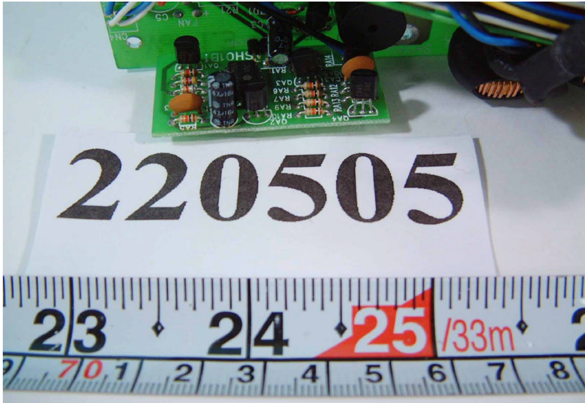
Front SIDE Module board of power
