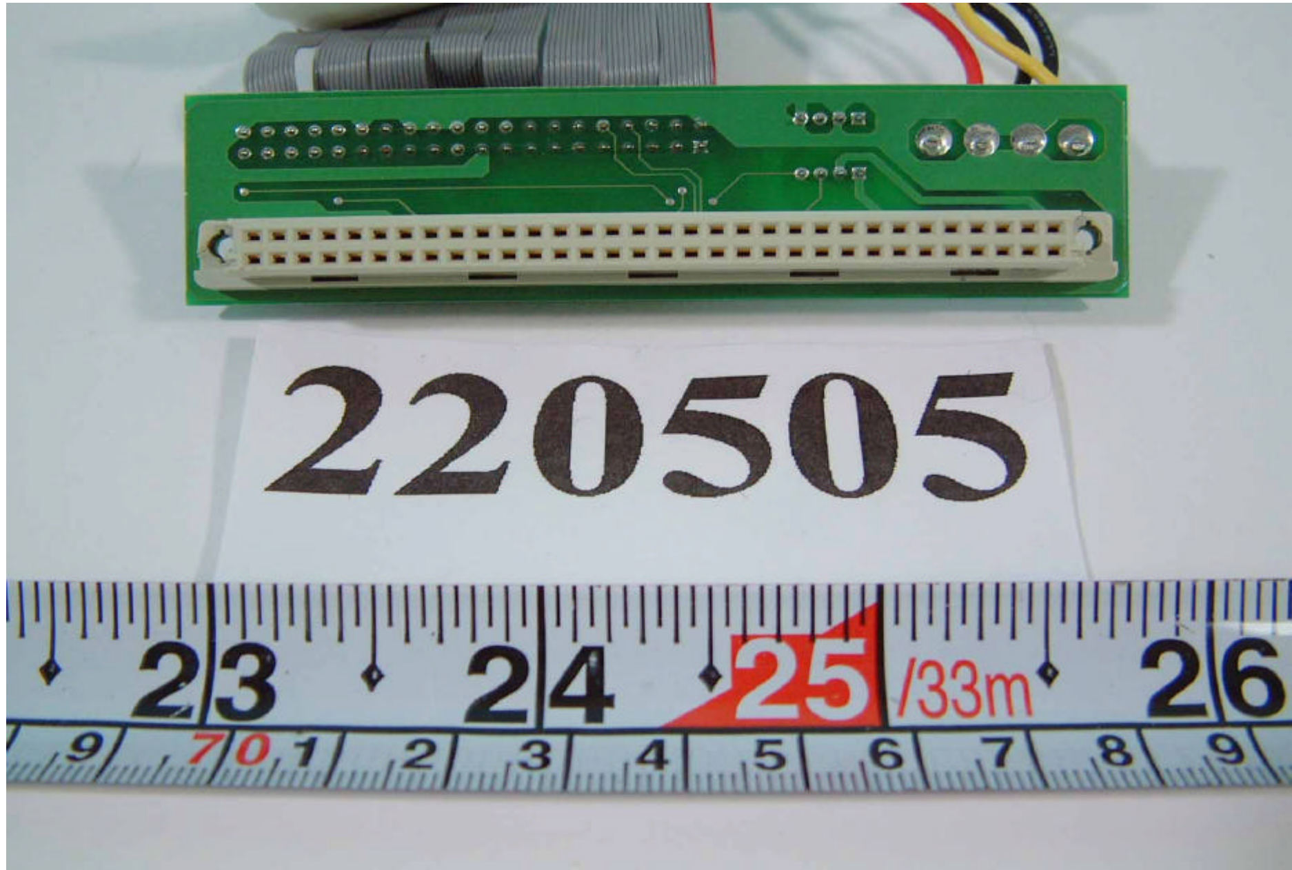
REAR SIDE OF Module board
