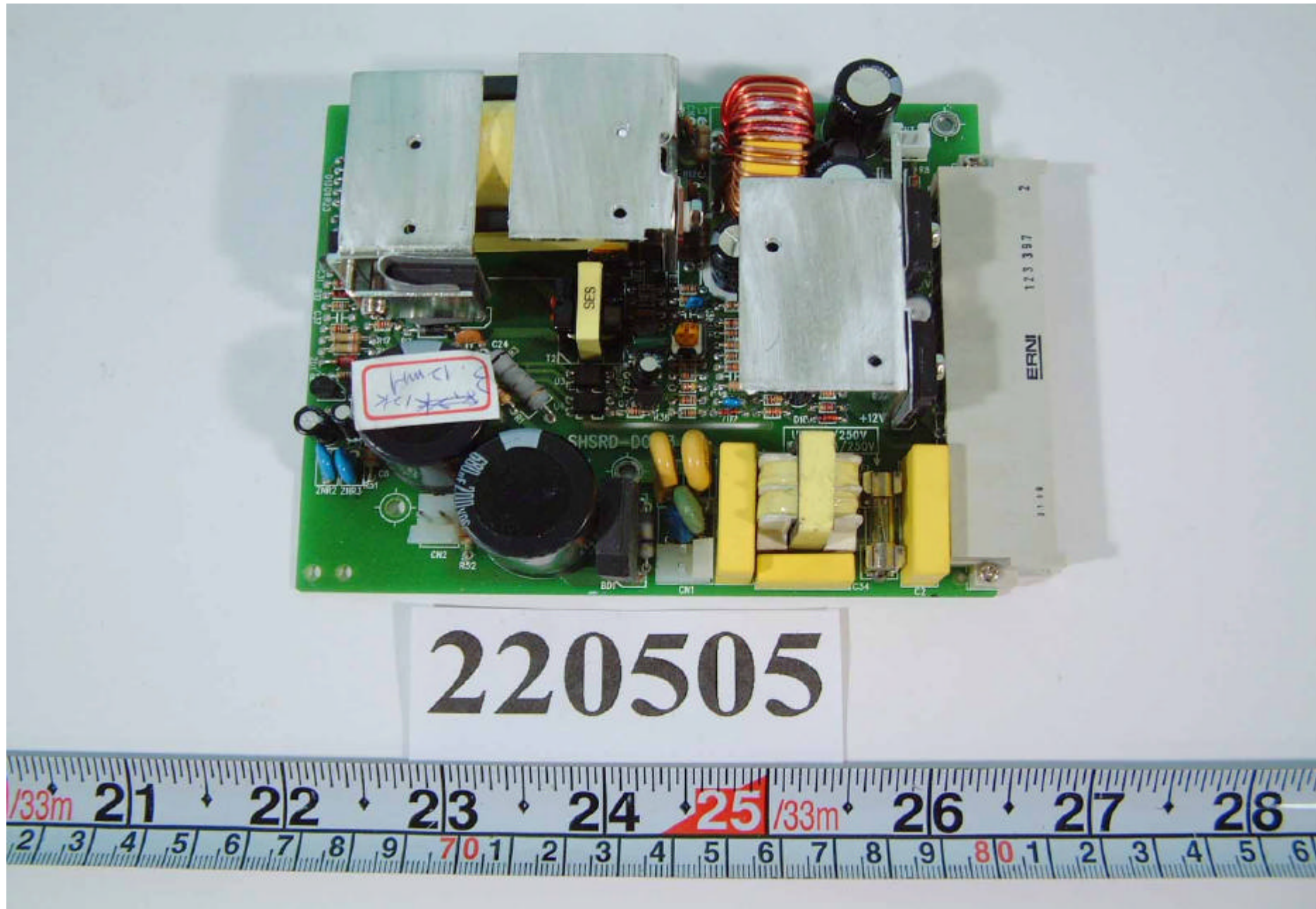
Front SIDE OF main board of module power
