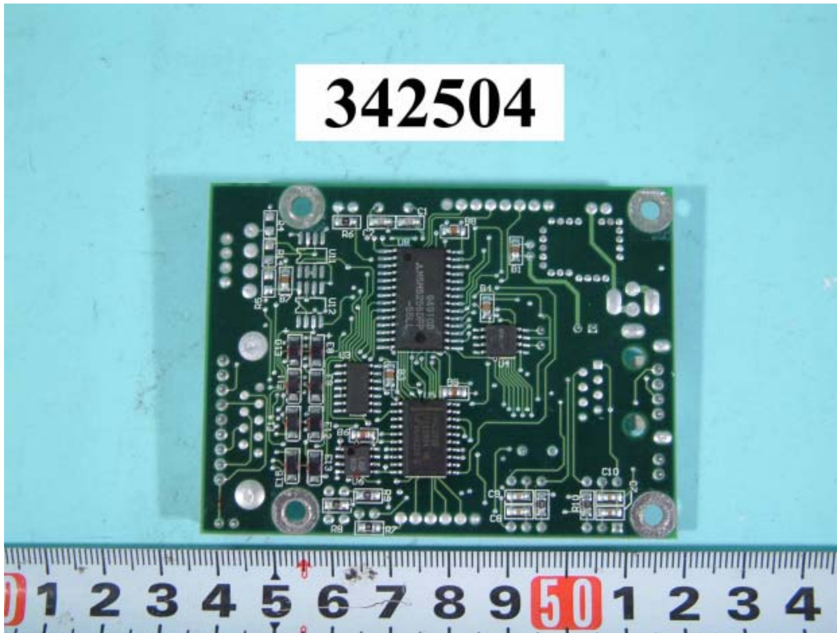
Rear side of RS-232 to RJ-45 connector board
