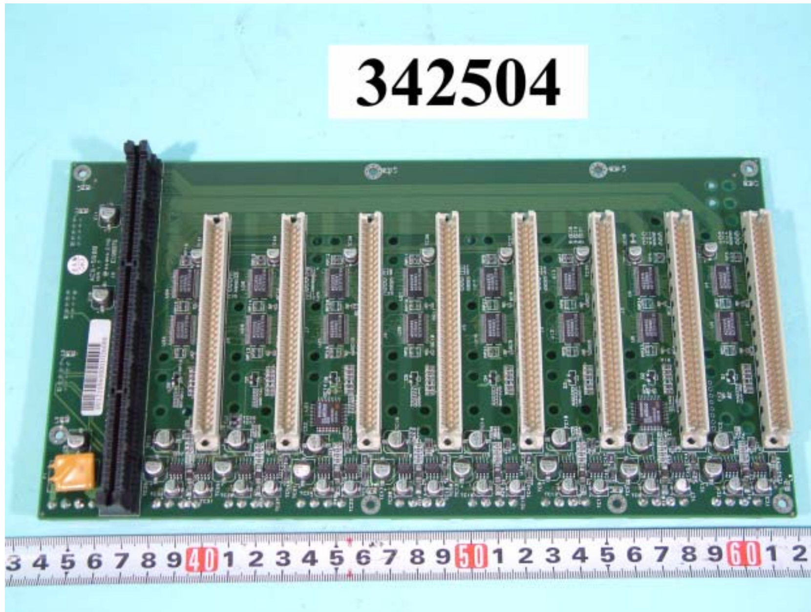
Front side of back plane
