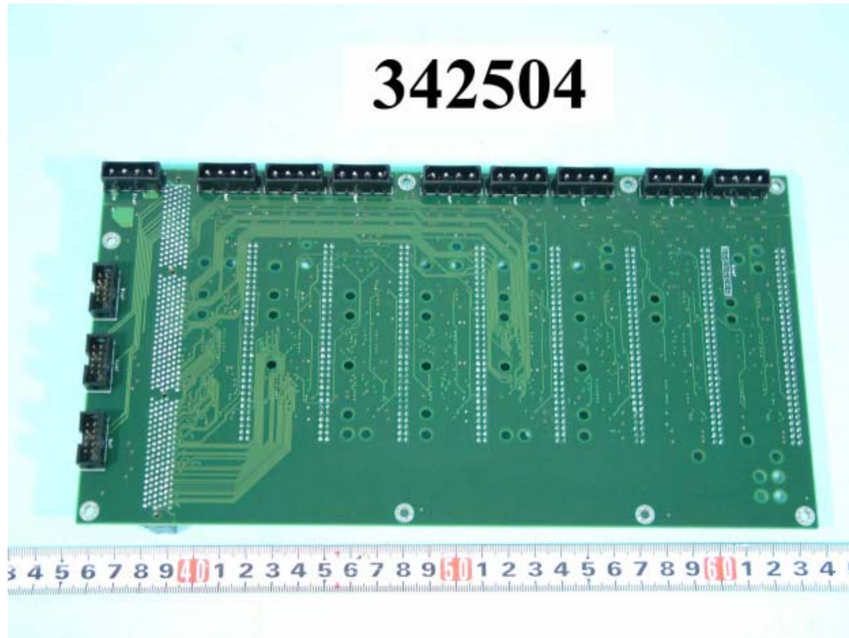
Rear side of back plane
