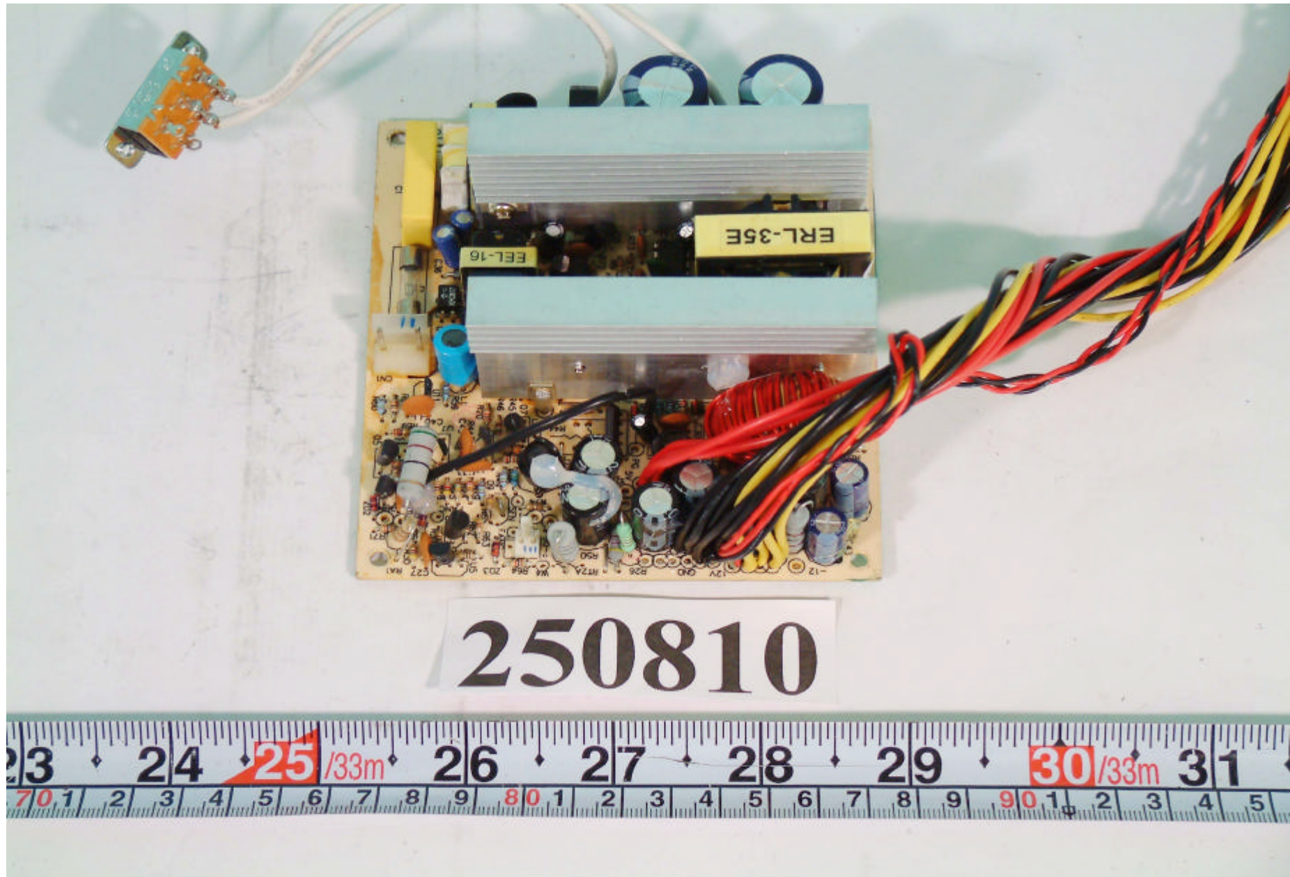
REAR SIDE of main board of power
