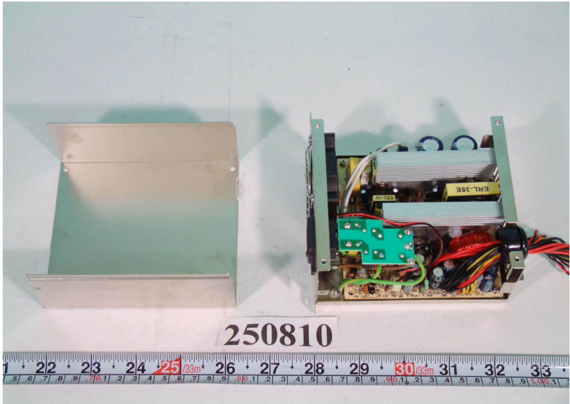
Mechanical Construction of power
