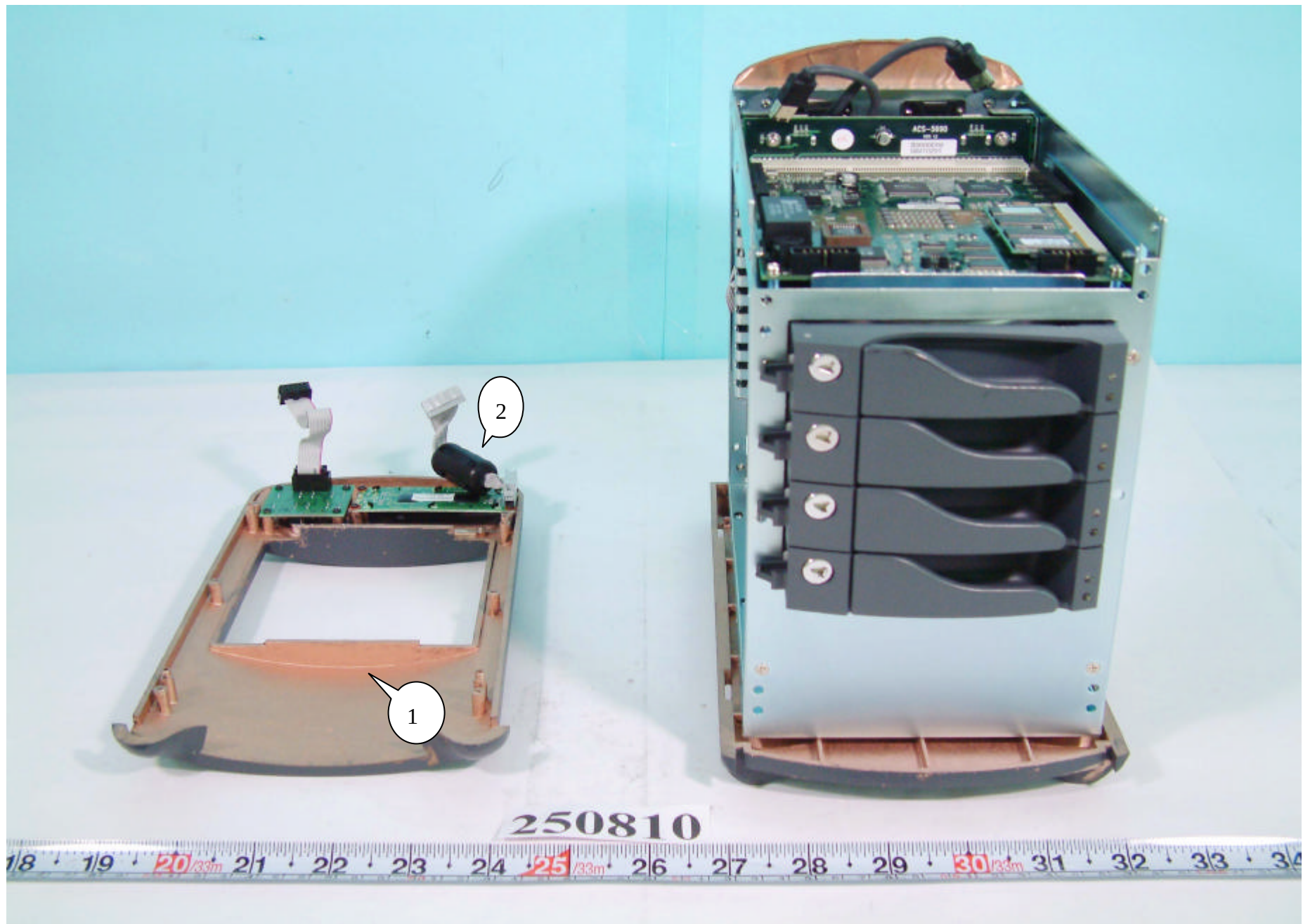
Mechanical Construction
