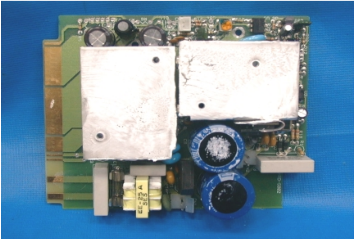
PHOTO. 23. POWER SUPPLY COMPONENT SIDE VIEW
