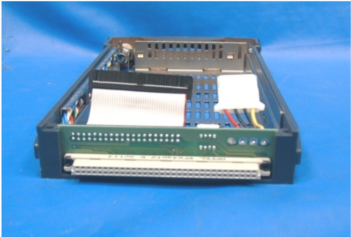
PHOTO. 11. HARD DISK CHASSIS INSIDE VIEW
