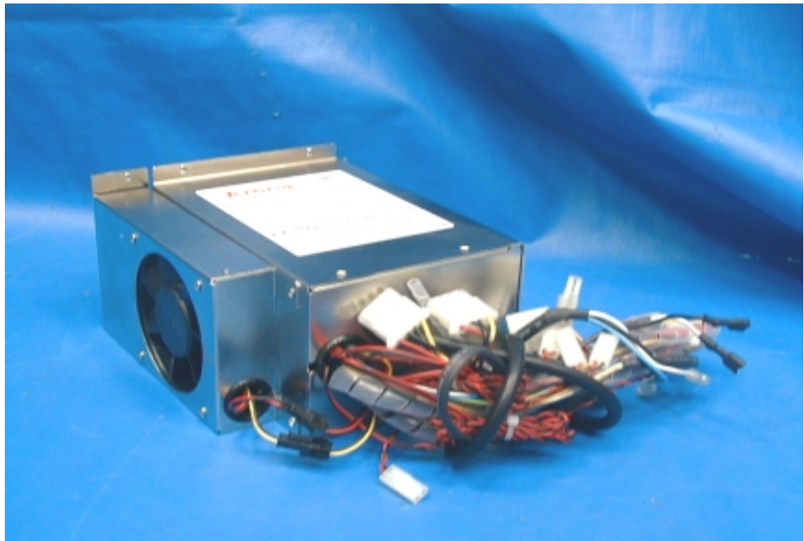
PHOTO. 16. POWER SUPPLY FRONT VIEW
