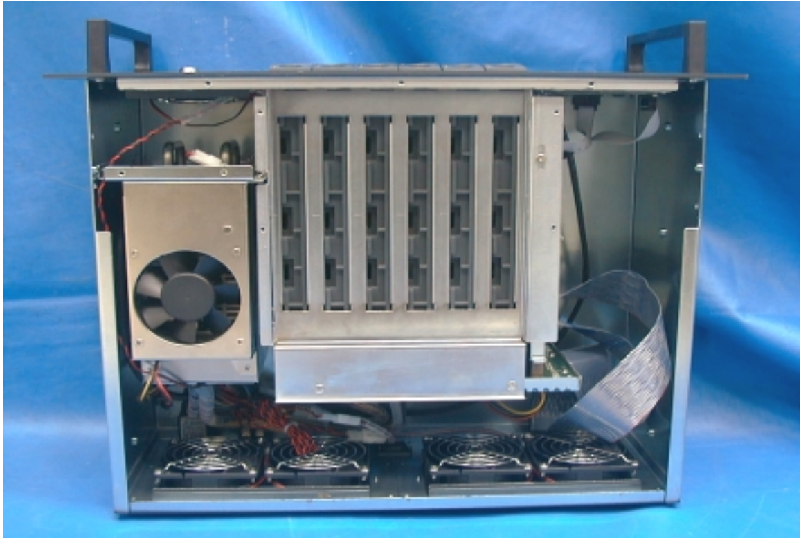
PHOTO. 5. EUT INSIDE VIEW
