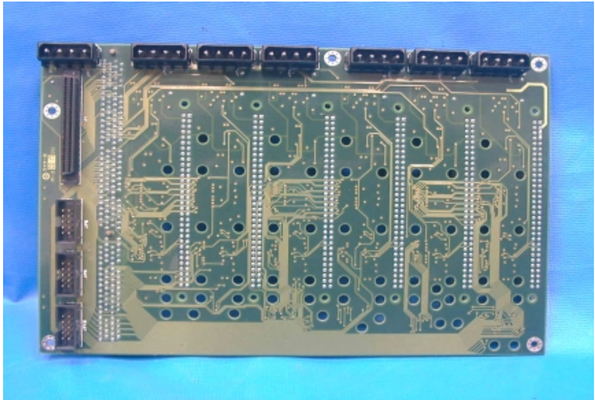
PHOTO. 13. EUT SOLDERING SIDE VIEW
