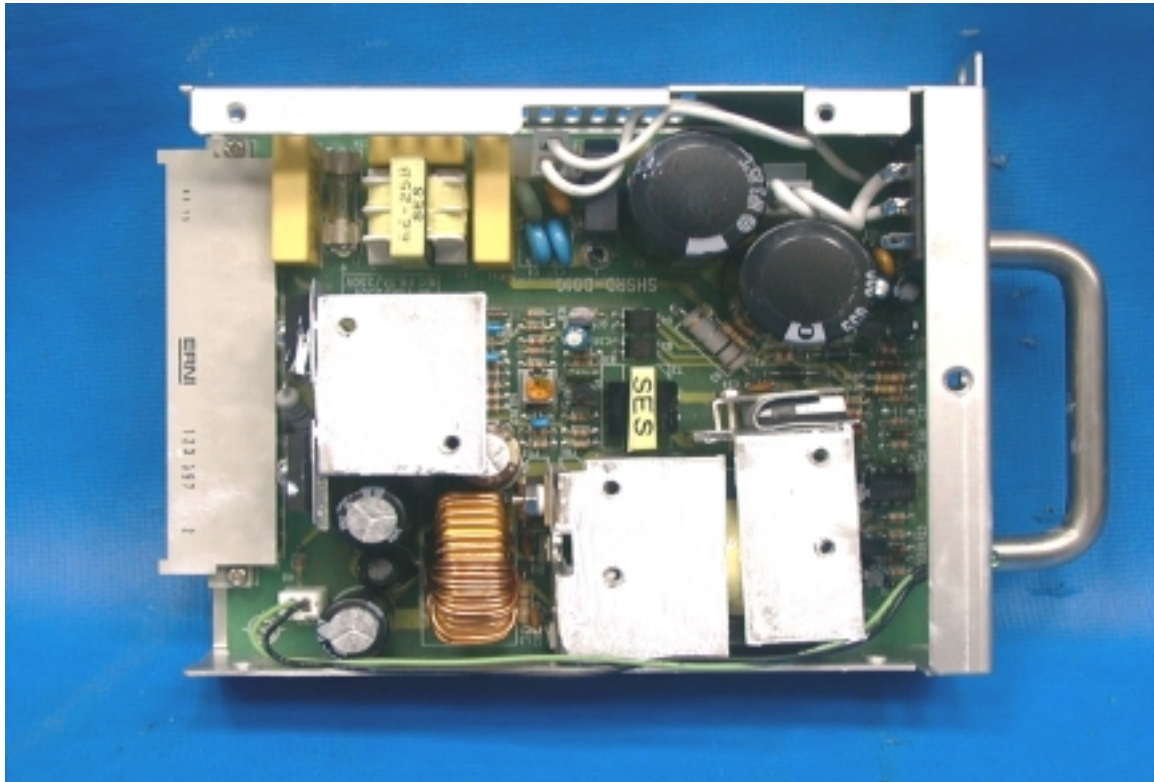
PHOTO. 24. POWER SUPPLY COMPONENT SIDE VIEW
