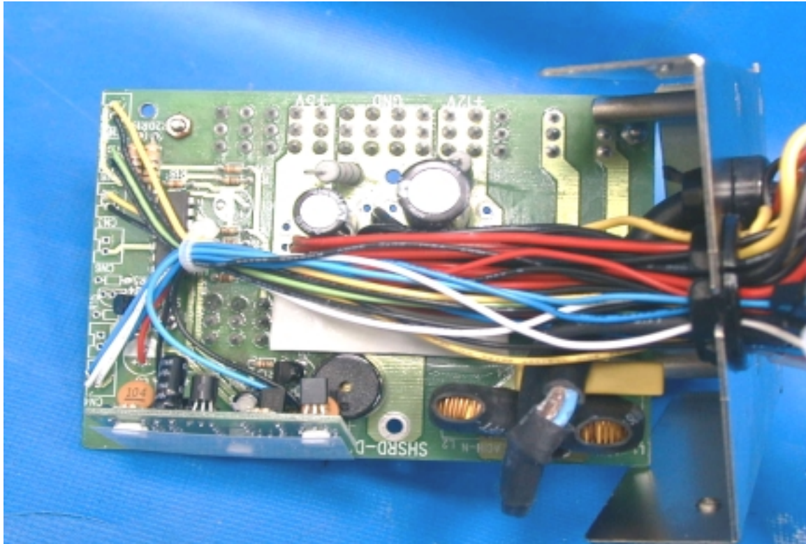
PHOTO. 28. EUT CABLE VIEW
