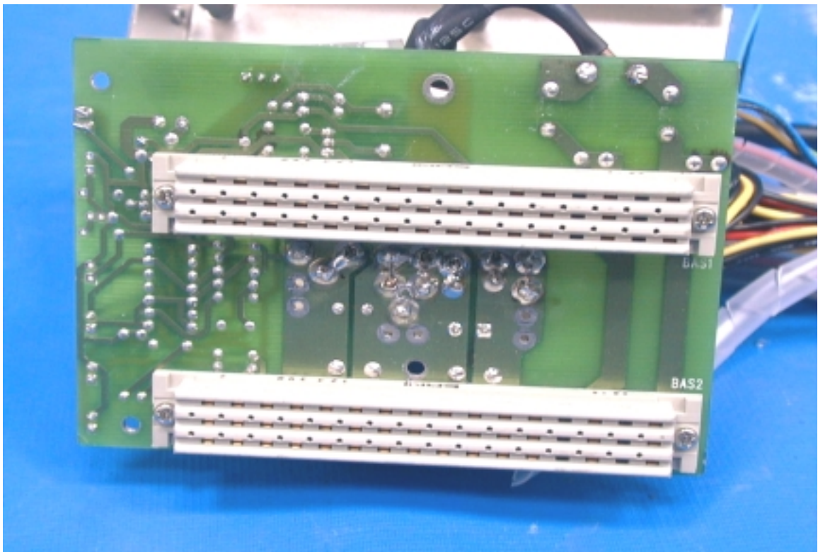
PHOTO. 26. POWER SUPPLY COMPONENT SIDE VIEW
