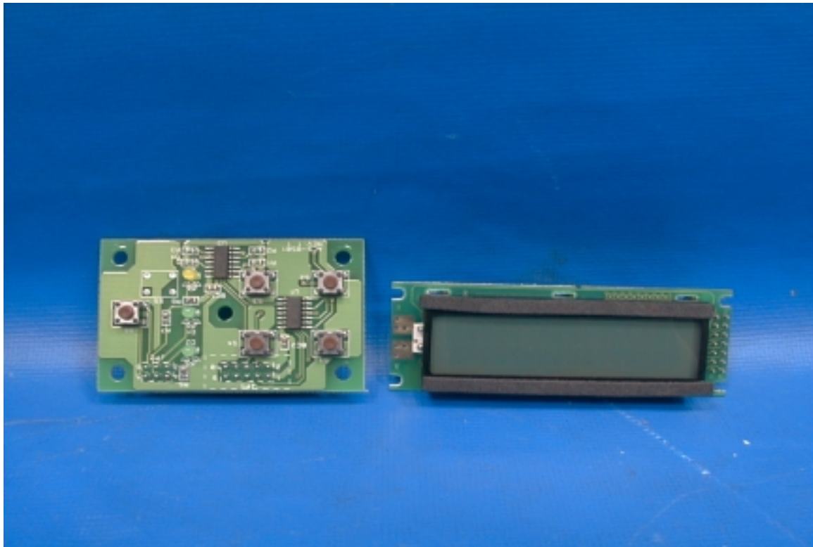
PHOTO. 16. EUT SOLDERING SIDE VIEW
