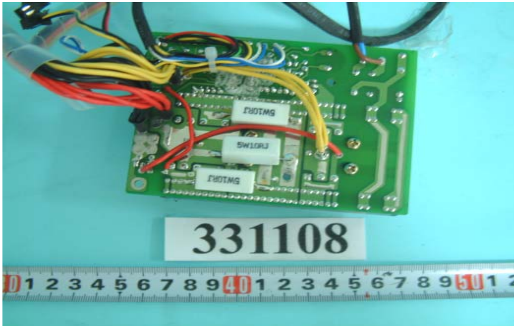
Rear side of power main board
