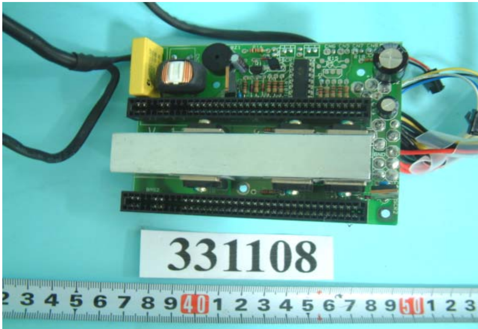
Front side of power main board
