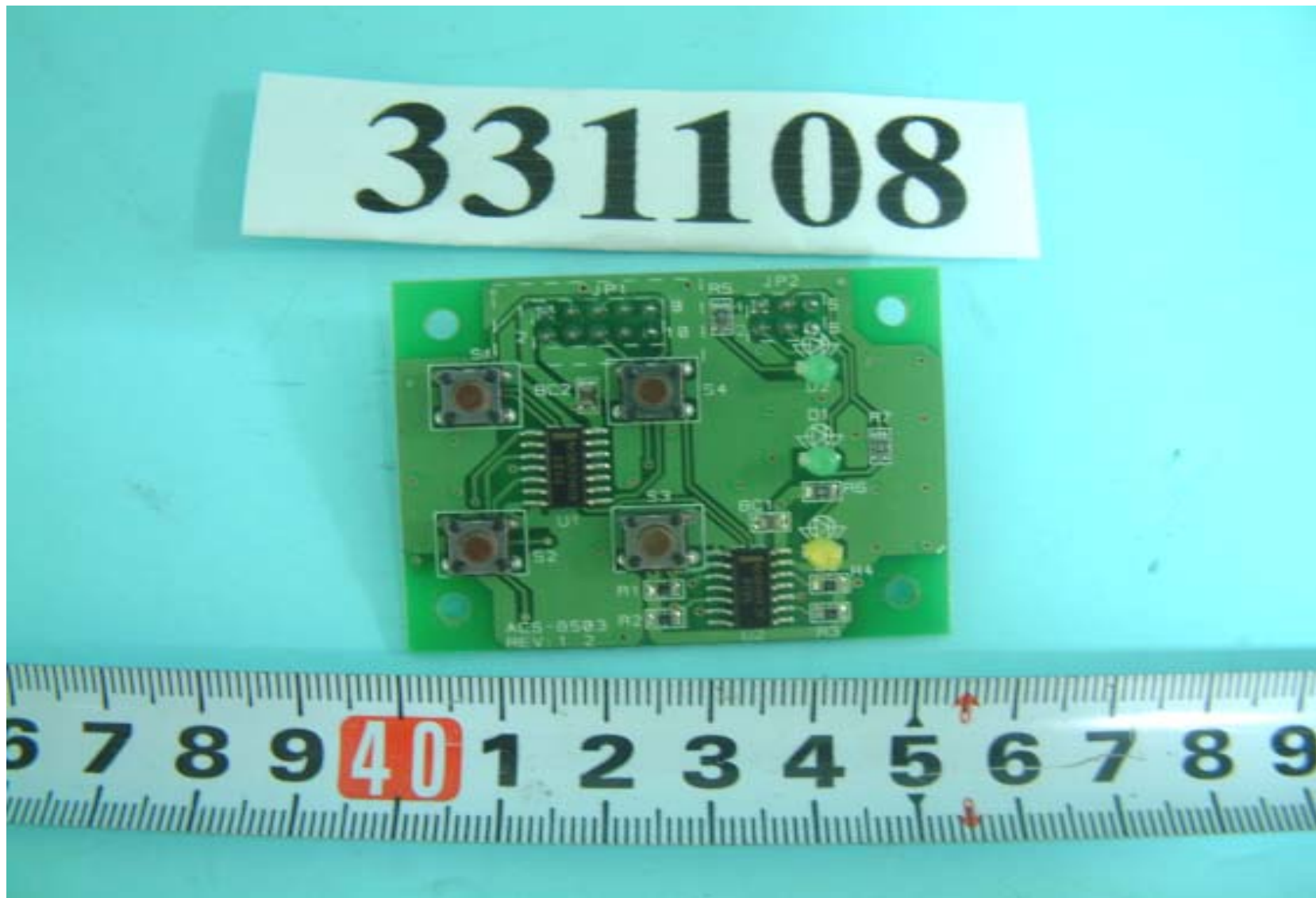
Front side of module board
