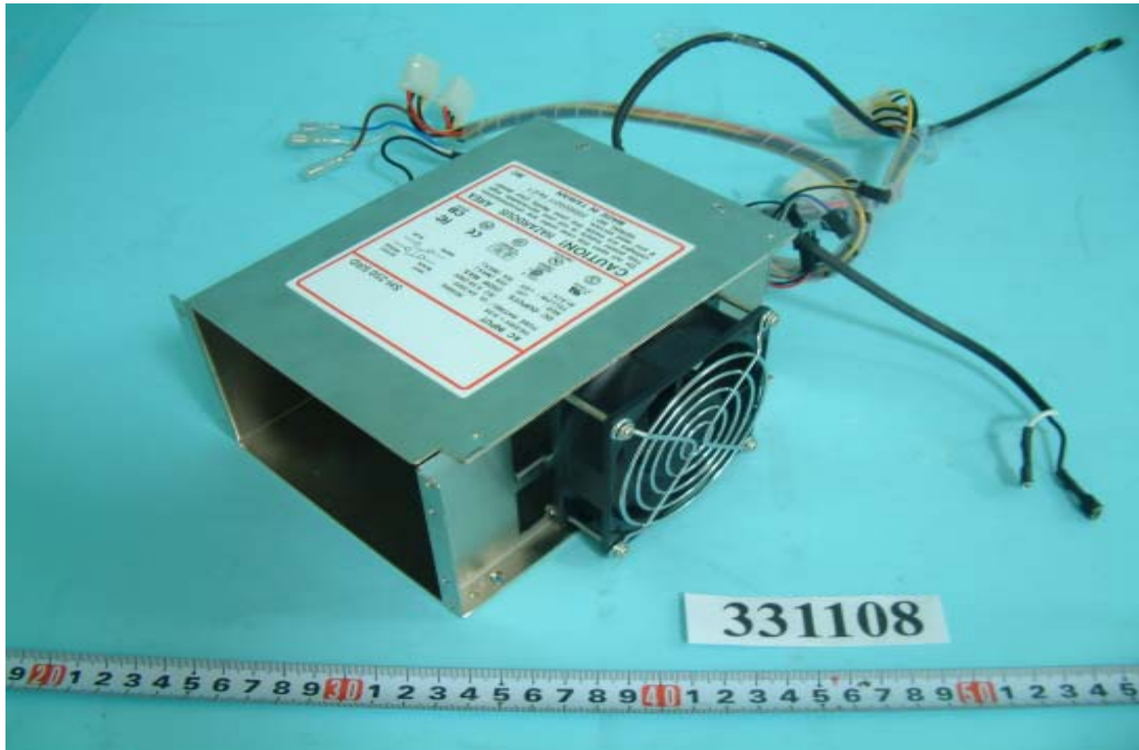
Front side of power
