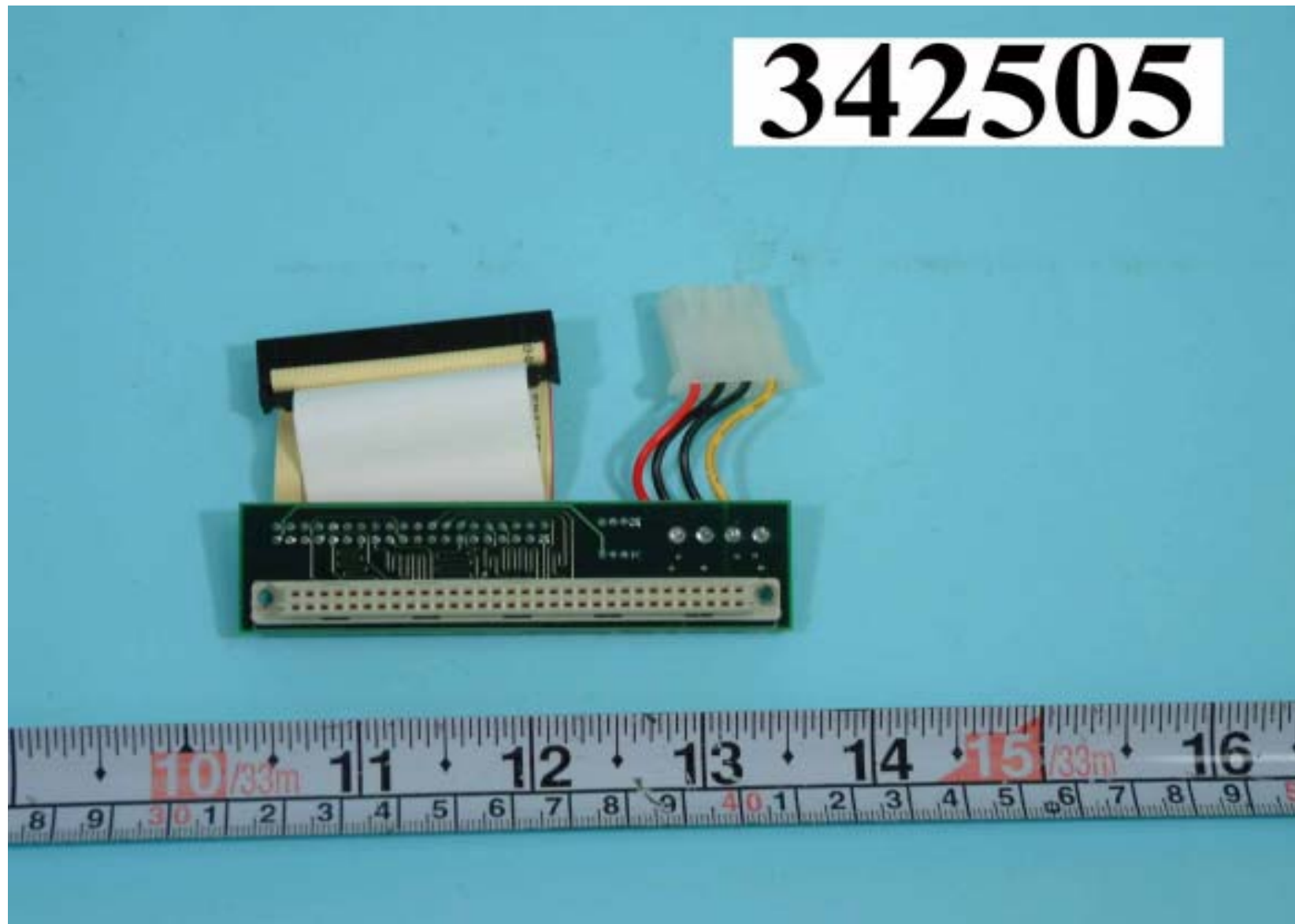
Rear side of module board
