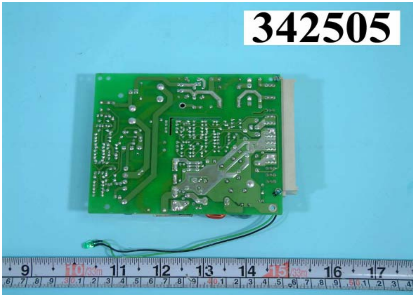
Rear side of main board of module power
