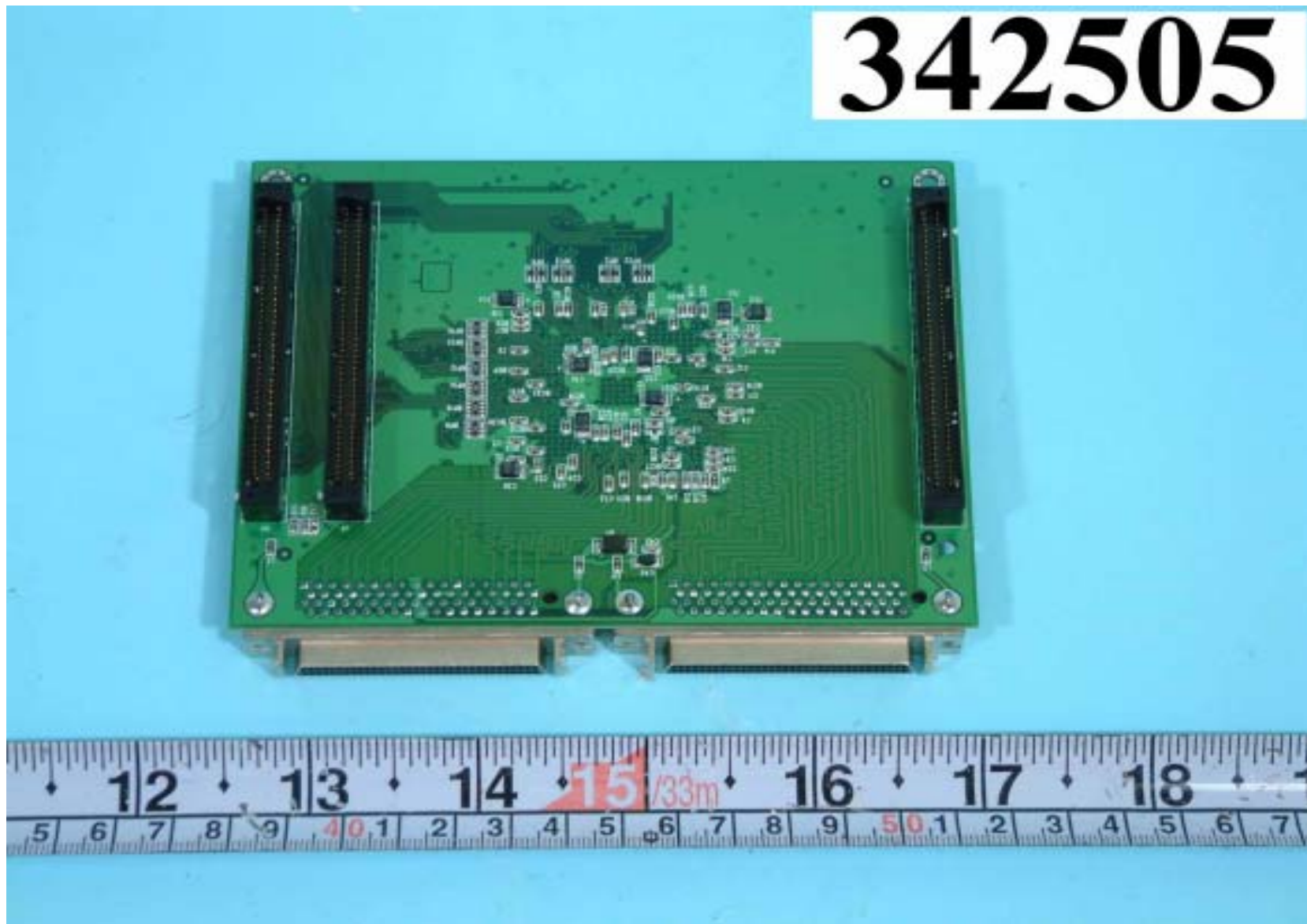
Rear side of SCSI daughter board
