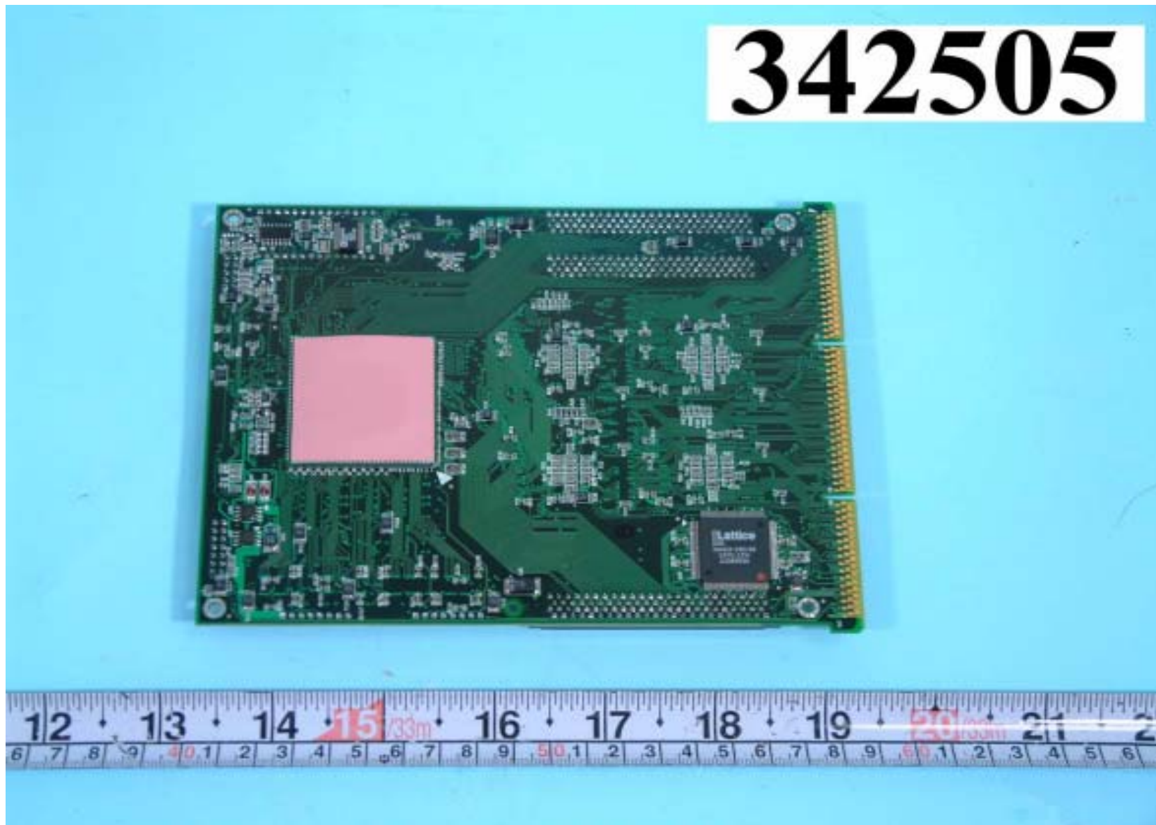
Rear side of controller
