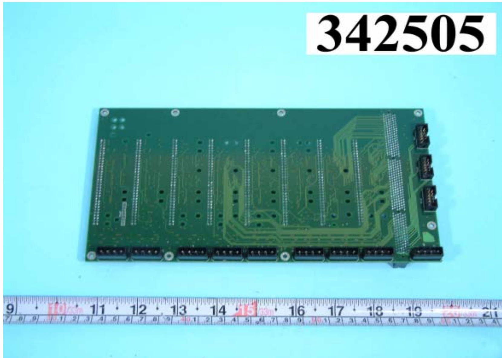
Rear side of back plane
