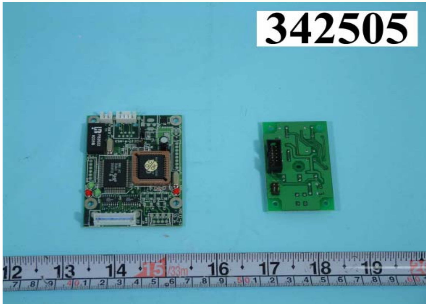
Front side of RS-232 to RJ-45 convertor and button board
