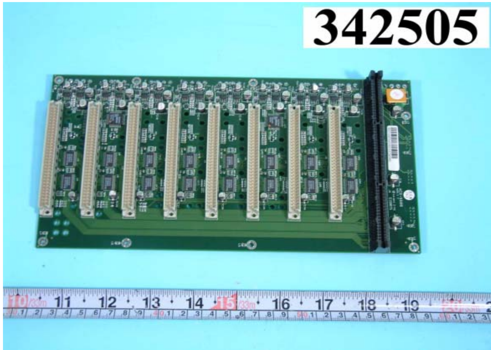
Front side of back plane
