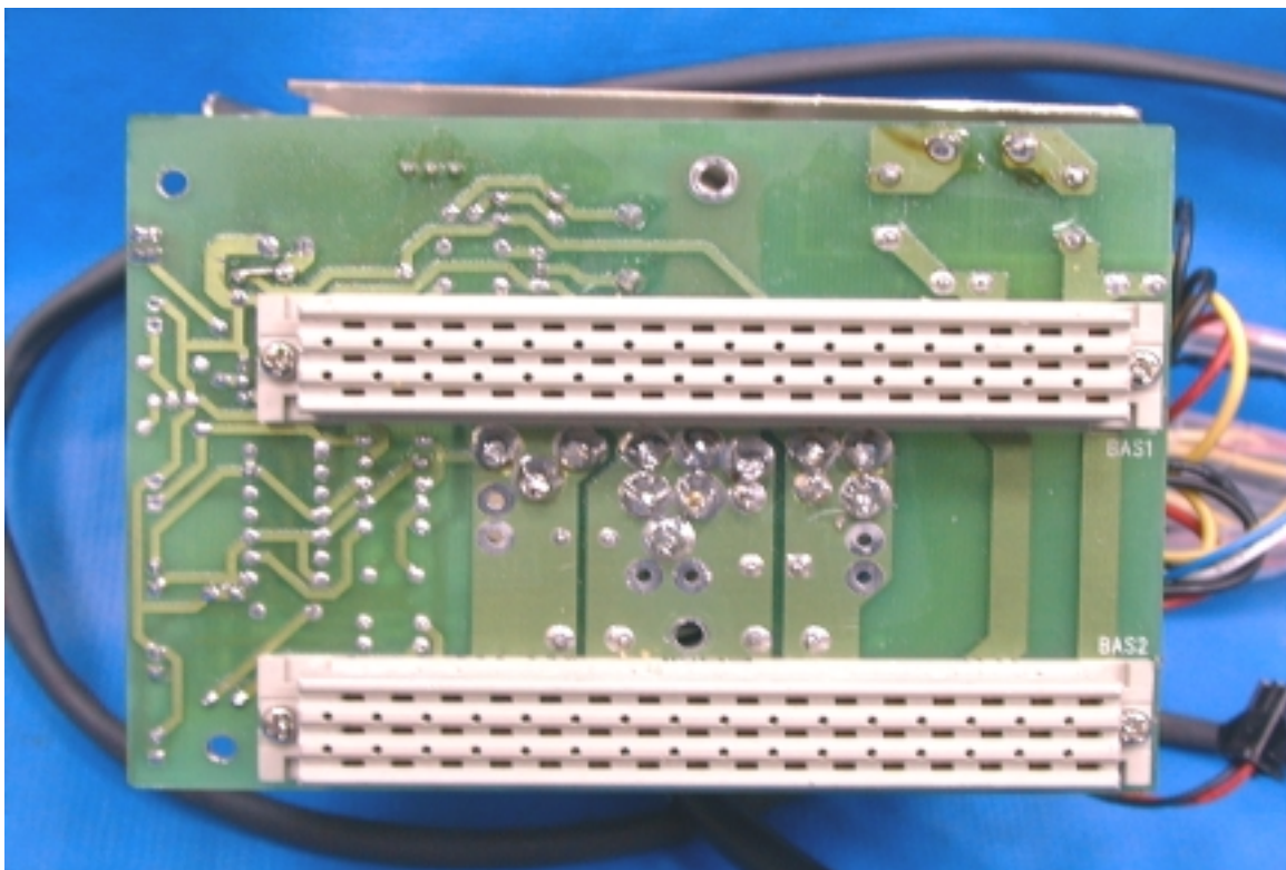
PHOTO. 16. POWER SUPPLY SOLDERING SIDE VIEW
