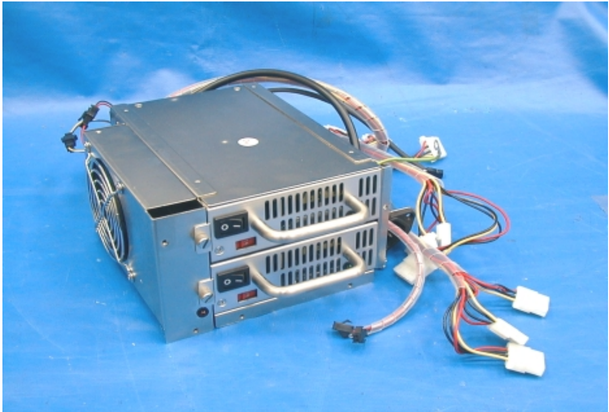
PHOTO. 14. POWER SUPPLY REAR VIEW
