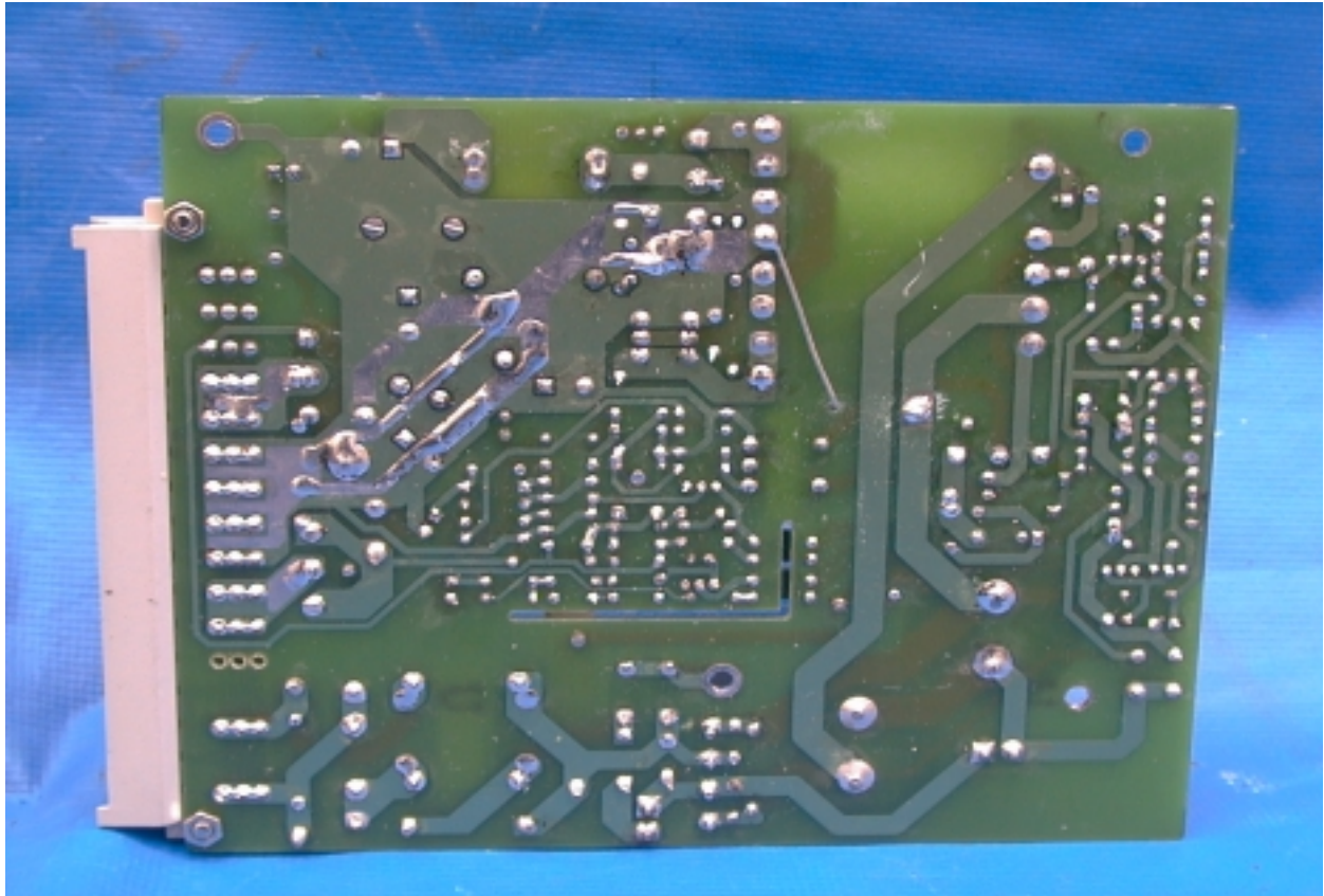
PHOTO. 23. POWER SUPPLY SOLDERING SIDE VIEW
