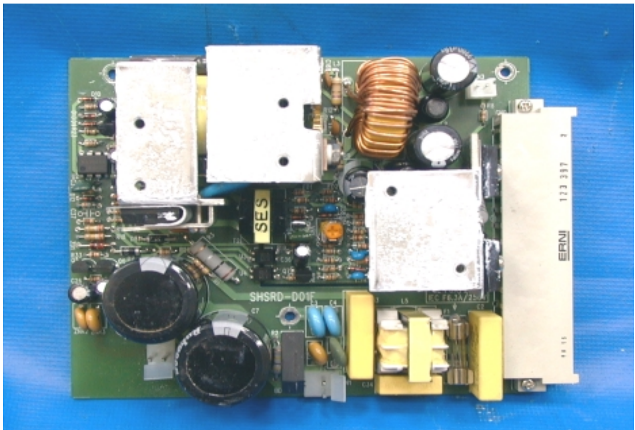
PHOTO. 22. POWER SUPPLY COMPONENT SIDE VIEW
