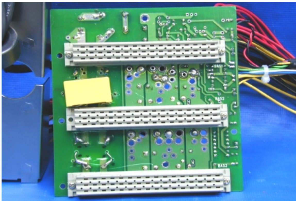
PHOTO. 5. EUT SOLDERING SIDE VIEW
