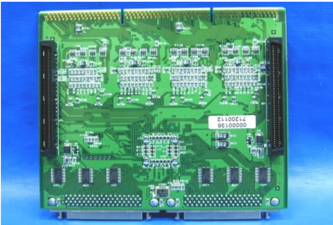
PHOTO. 14. EUT SOLDERING SIDE VIEW
