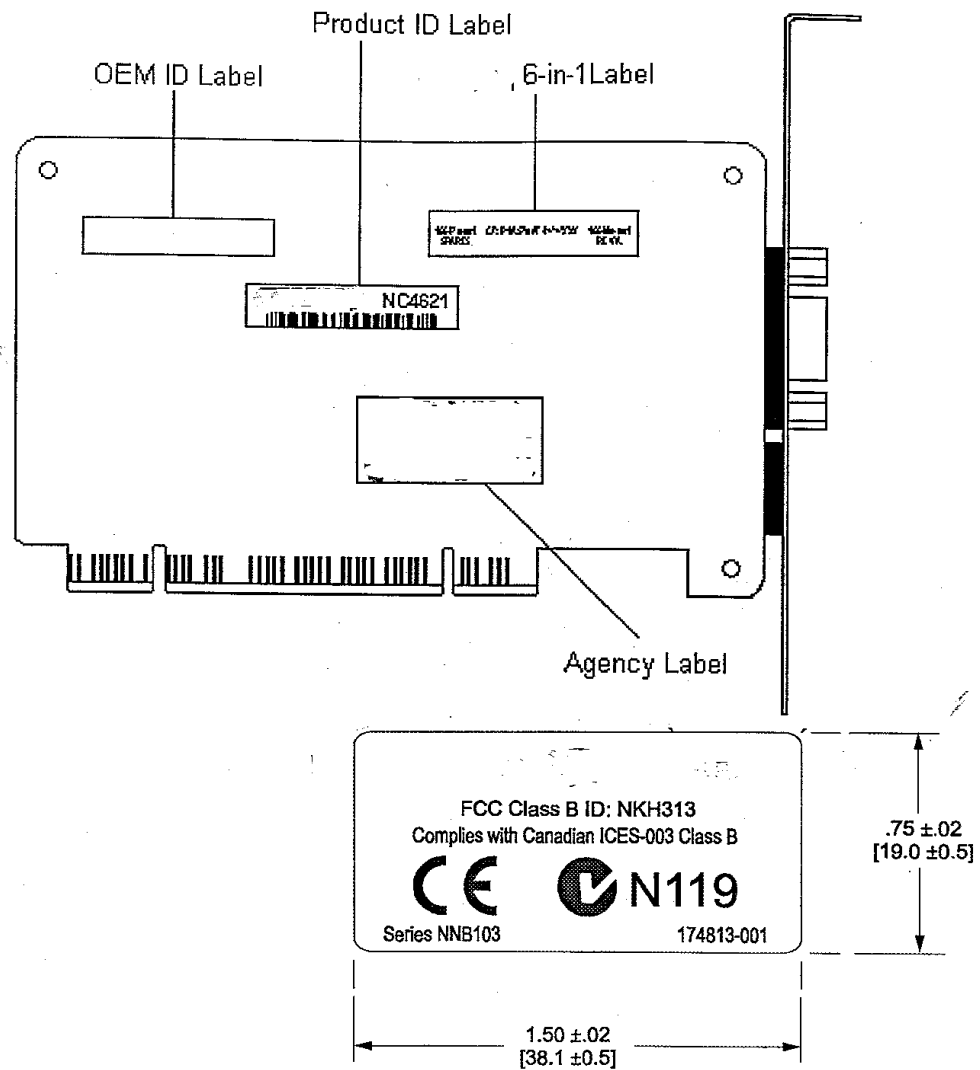
Figure 4 Board Label Placement Bottom Side View
