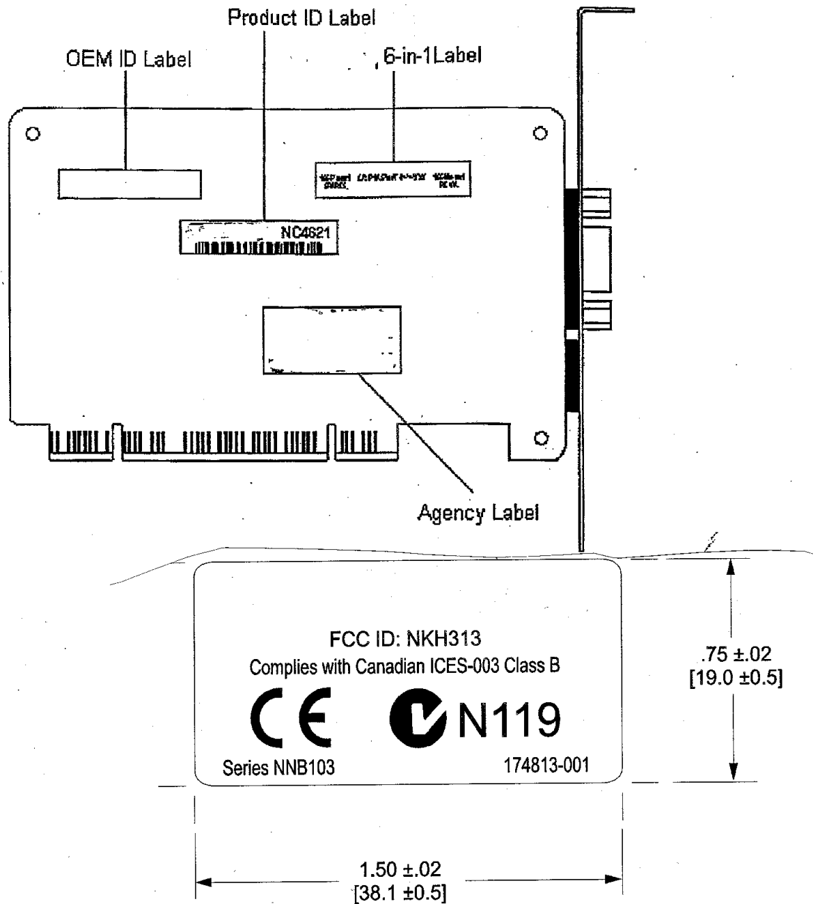
Figure 4 Board Label Placement Bottom Side View
