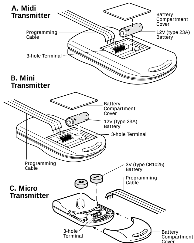
Figure 1. Battery Compartment
