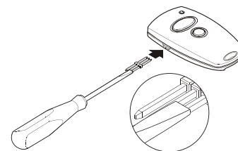
Figure 4. Code Changing
