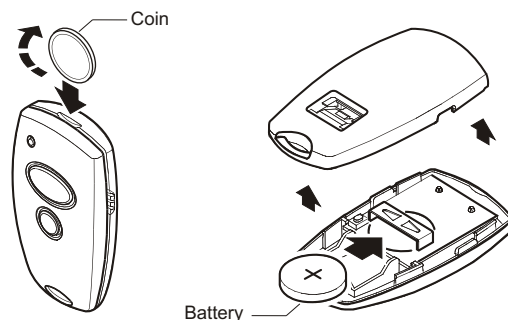
Figure 2. Battery Compartment
