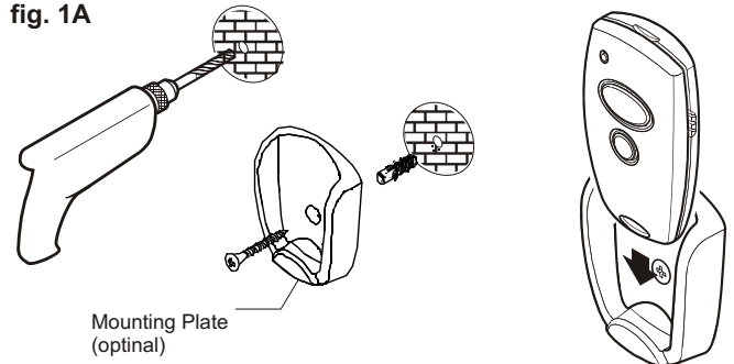
Figure 1. Mounting Plate & Visor Clip
