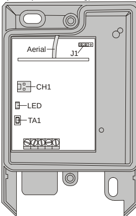
RCL04 (waterproof housing)
