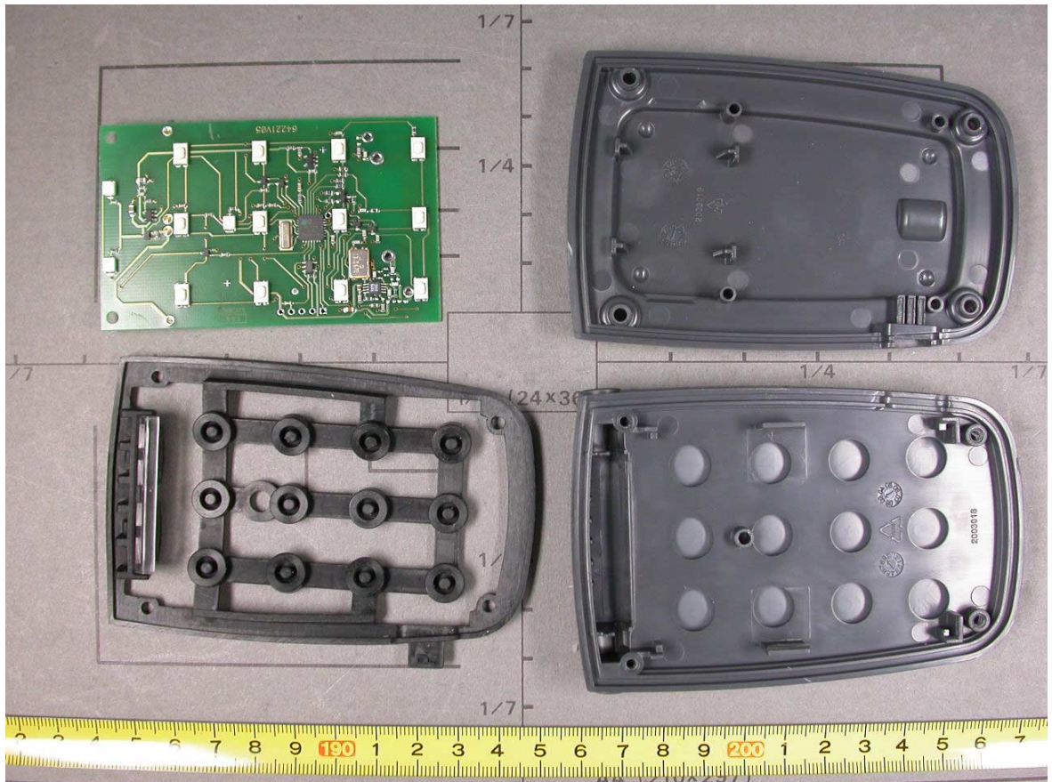
Unit disassembled
