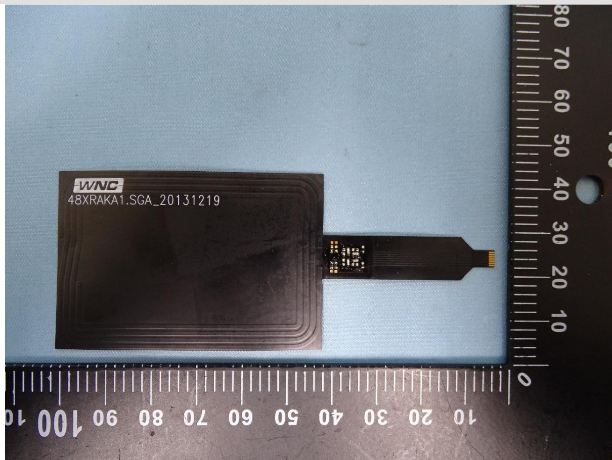
NFC Antenna Front view
