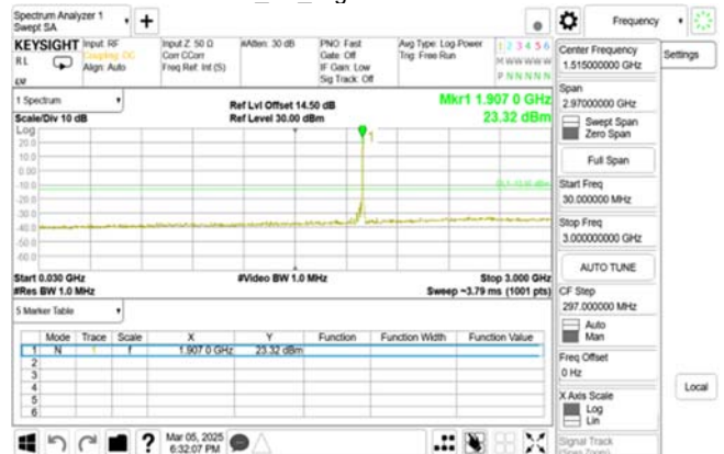
HSDPA_B2_HighCH9538-1907.6
