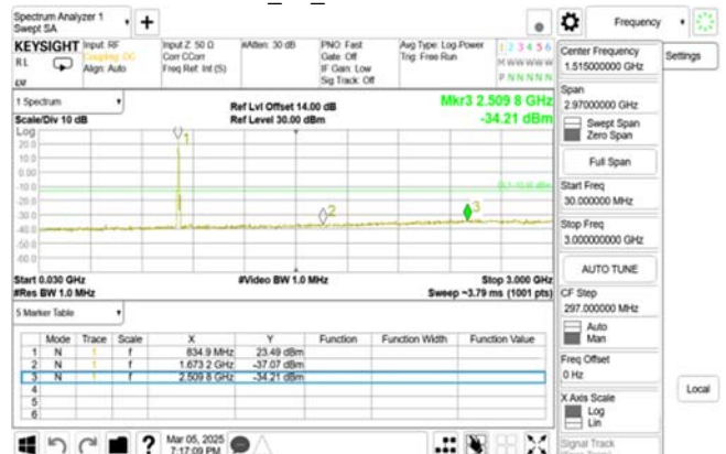
HSDPA_B5_MidCH4183-836.6
