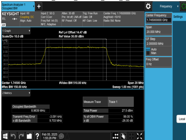
Band66_10MHz_256QAM_RB50_0_CH132322
