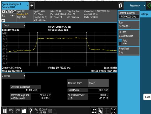
Band66_15MHz_16QAM_RB75_0_CH132047
