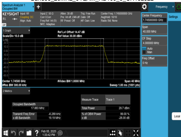
Band66_20MHz_256QAM_RB100_0_CH132322
