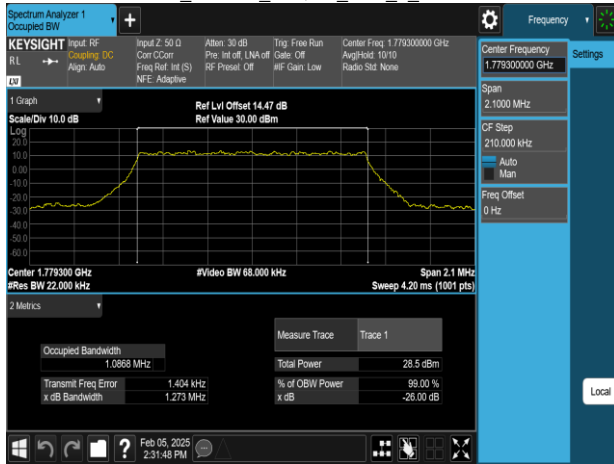
Band66 1.4MHz_256QAM_RB6_0_CH132665
