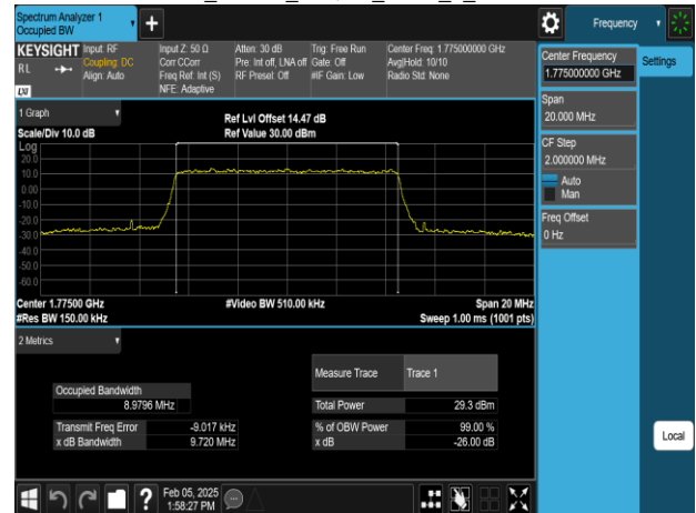
Band66_10MHz_64QAM_RB50_0_CH132622
