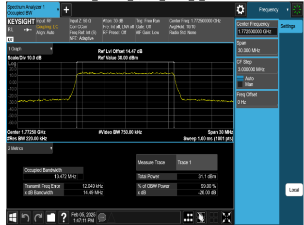
Band66_15MHz_16QAM_RB75_0_CH132597
