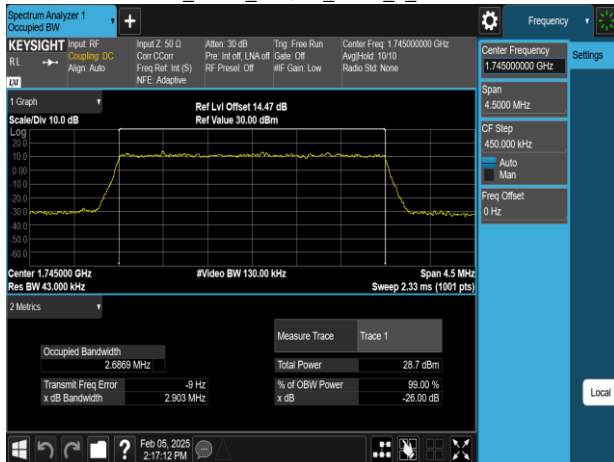
Band66 3MHz 64QAM RB15_0_CH132322
