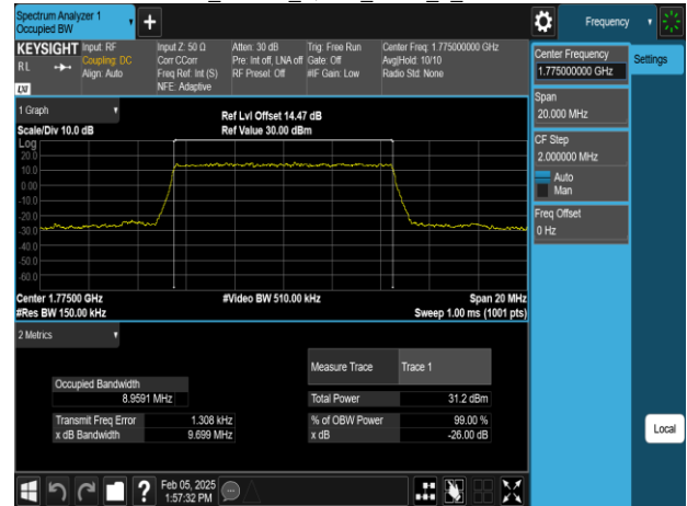
Band66_10MHz_16QAM_RB50_0_CH132622
