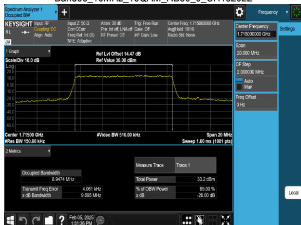
Band66_10MHz_16QAM_RB50_0_CH132022
