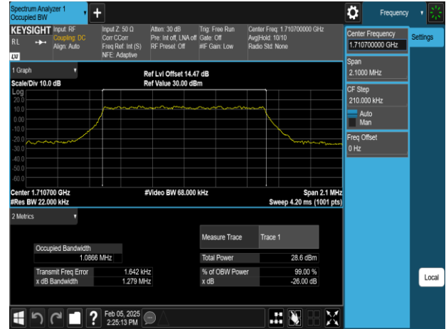
Band66_1.4MHz_256QAM_RB6_0_CH131979
