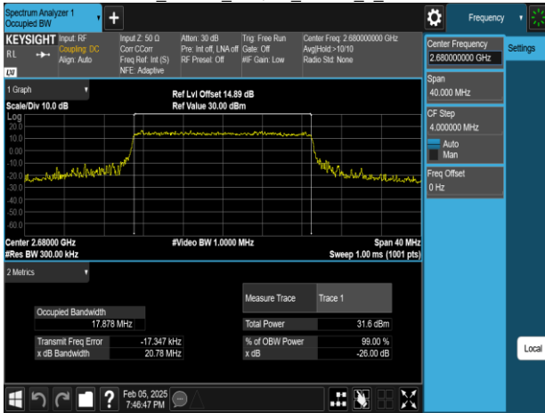
Band41_20MHz_256QAM_RB100_0_CH41490
