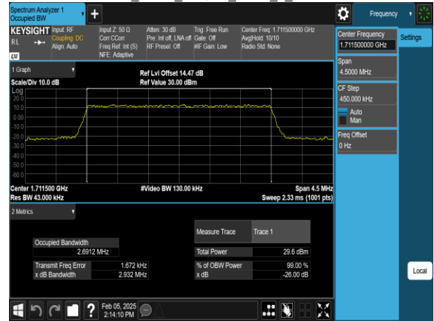
Band66 3MHz_64QAM_RB15_0_CH131987
