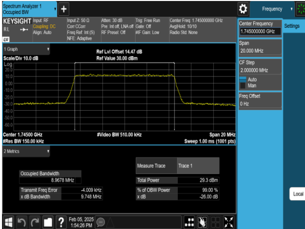
Band66_10MHz_256QAM_RB50_0_CH132322
