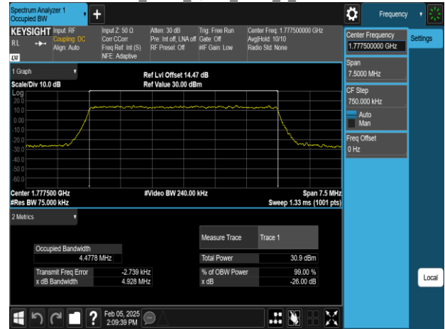
Band66_5MHz_16QAM_RB25_0_CH132647
