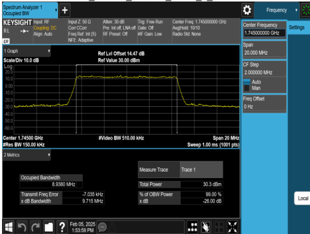
Band66_10MHz_64QAM_RB50_0_CH132322
