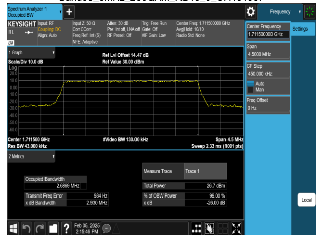
Band66 3MHz_256QAM_RB15_0_CH131987
