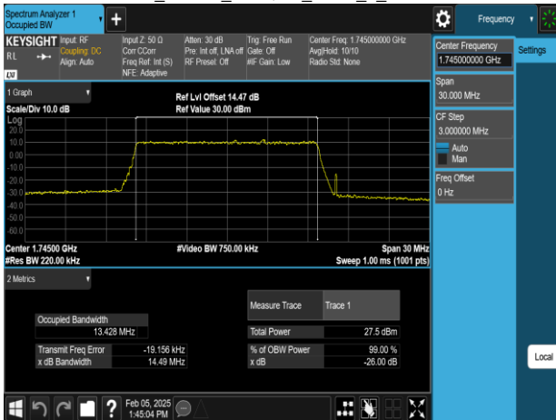
Band66_15MHz_256QAM_RB75_0_CH132322
