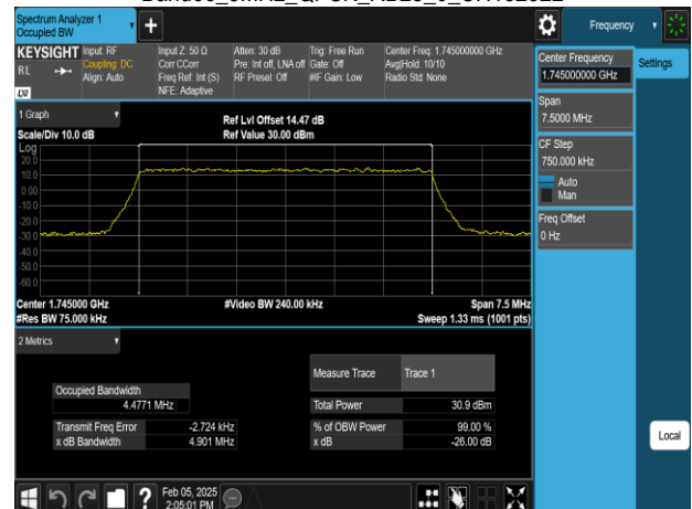
Band66_5MHz_QPSK_RB25_0_CH132322
