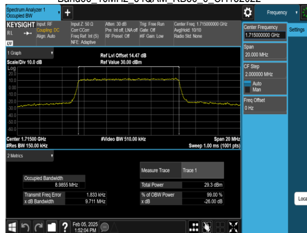
Band66_10MHz_256QAM_RB50_0_CH132022
