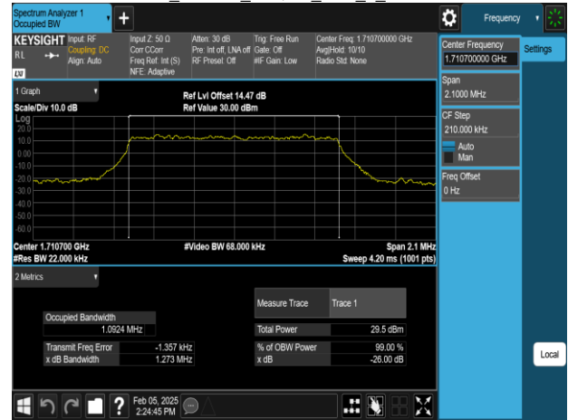
Band66_1.4MHz_64QAM_RB6_0_CH131979
