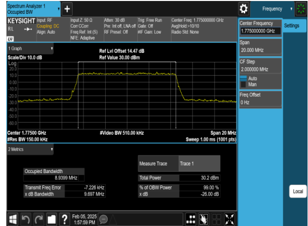
Band66_10MHz_64QAM_RB50_0_CH132622
