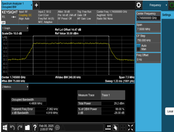
Band66_5MHz_256QAM_RB25_0_CH132322
