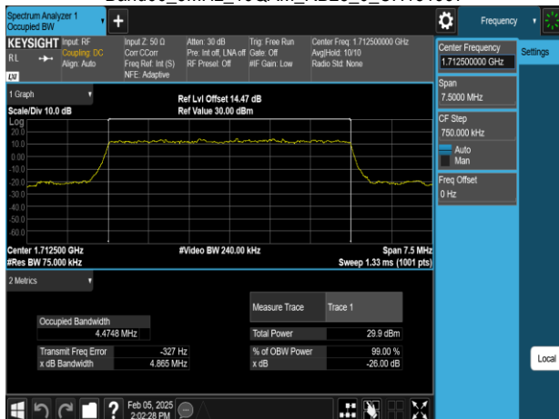
Band66_5MHz_16QAM_RB25_0_CH131997
