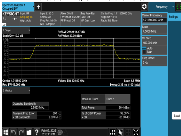
Band66 3MHz_QPSK_RB15_0_CH131987
