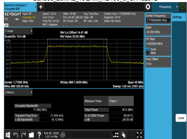
Band66_20MHz_64QAM_RB100_0_CH132572
