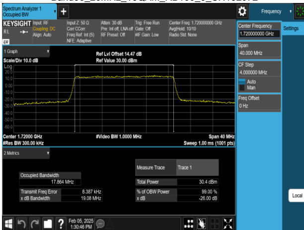
Band66 20MHz_16QAM_RB100_0_CH132072
