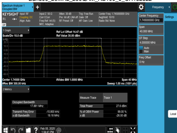
Band66_20MHz_256QAM_RB100_0_CH132322
