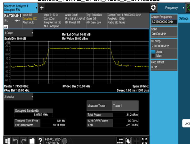
Band66_10MHz_QPSK_RB50_0_CH132322
