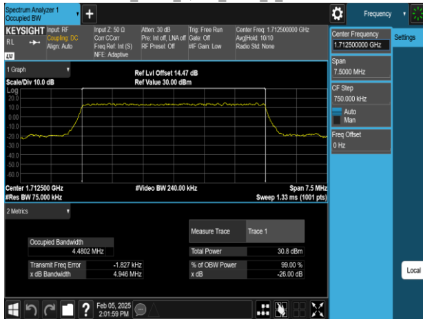
Band66_5MHz_16QAM_RB25_0_CH131997
