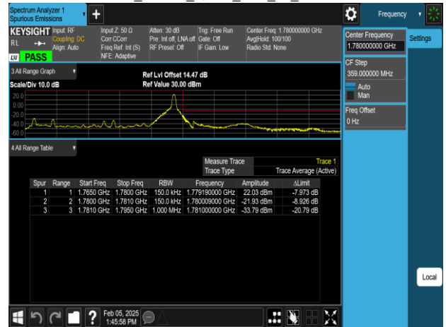
Band66_15MHz_QPSK_RB75_0_CH132597
