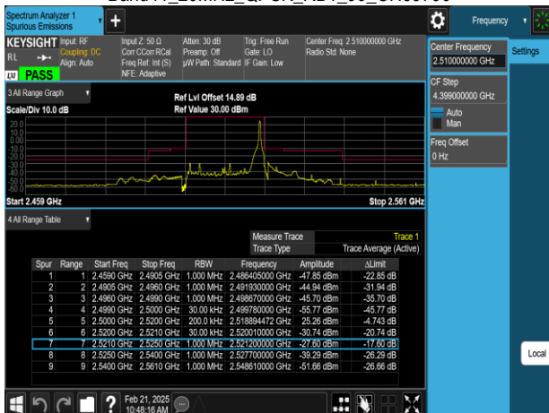
Band41_20MHz_QPSK_RB1_99_CH39790
