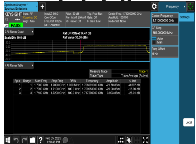
Band66_10MHz_QPSK_RB50_0_CH132022
