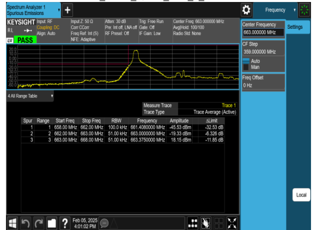
Band71 5MHz_QPSK_RB25_0_CH133147
