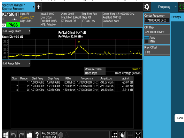
Band66_15MHz_QPSK_RB1_0_CH132047
