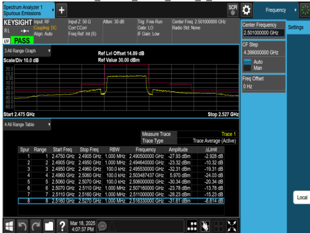
Band41_10MHz_QPSK_RB1_0_CH39740
