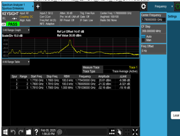
Band66_10MHz_QPSK_RB50_0_CH132622
