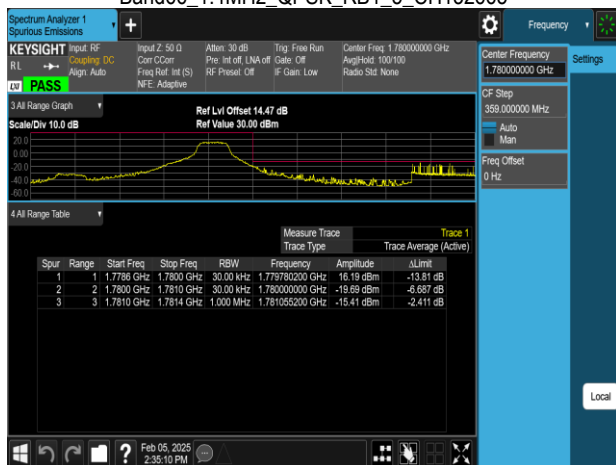
Band66_1.4MHz_QPSK_RB6_0_CH132665
