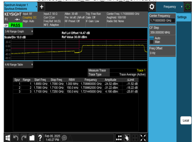
Band66_15MHz_QPSK_RB1_74_CH132597
