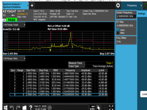
Band41_20MHz_QPSK_RB1_99_CH39750
