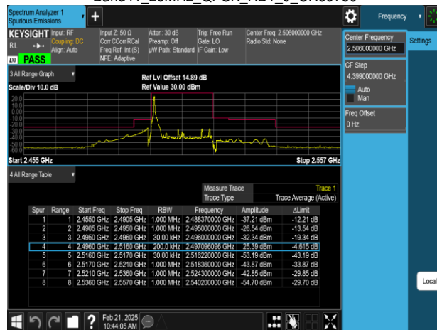
Band41_20MHz_QPSK_RB1_99_CH39750
