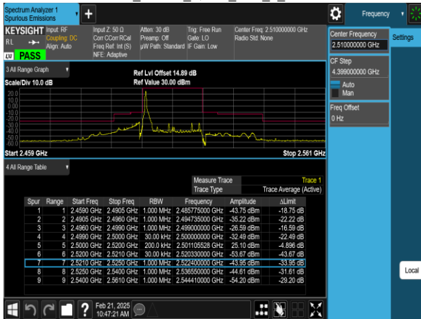
Band41_20MHz_QPSK_RB1_99_CH39790
