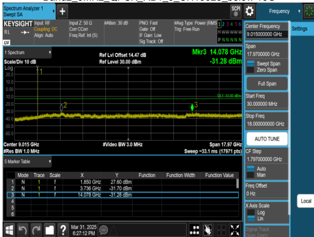
Band2_5MHz_QPSK_RB1_0_CH18625_upper 18G
