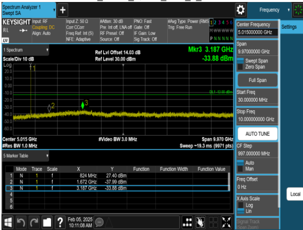
Band26_5MHz_QPSK_RB1_0_CH26915
