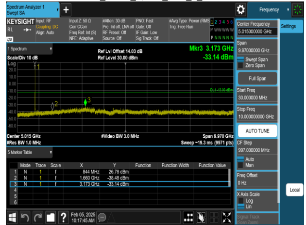
Band26_5MHz_QPSK_RB1_0_CH27685 below 18G
