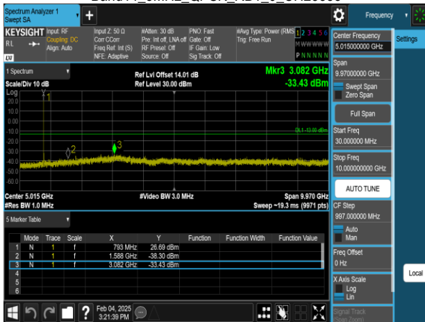
Band17_5MHz_QPSK_RB1_0_CH23755
