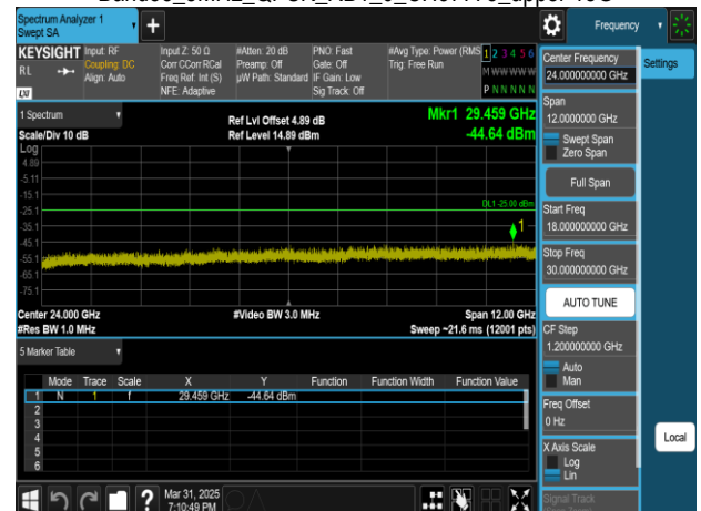
Band38_5MHz_QPSK_RB1_0_CH37775_upper 18G
