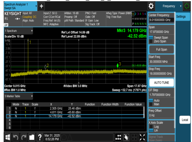
Band30_5MHz_QPSK_RB1_0_CH27685_upper 18G
