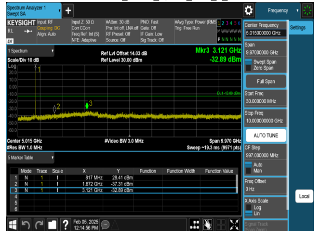
Band26-Part90s_5MHz_QPSK_RB1_0_CH26740
