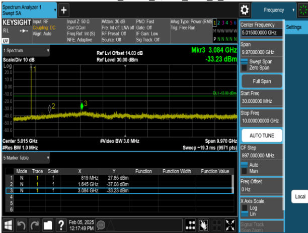
Band26_5MHz_QPSK_RB1_0_CH26815
