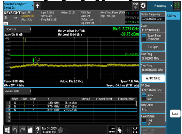
Band25_5MHz_QPSK_RB1_0_CH26065_upper 18G
