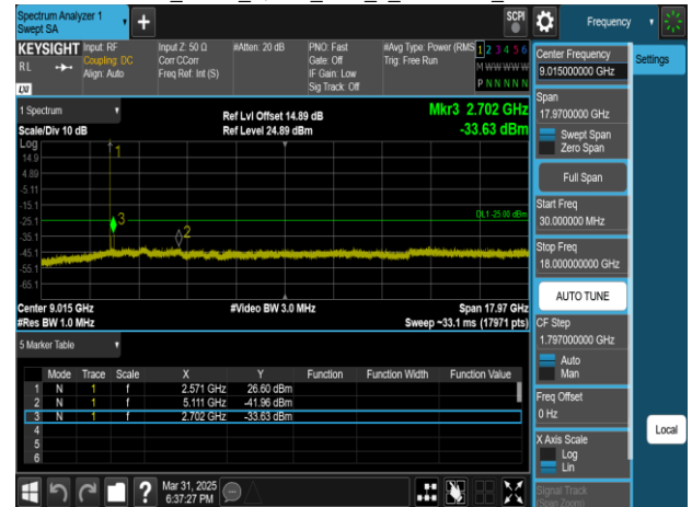
Band38_5MHz_QPSK_RB1_0_CH37775_upper 18G
