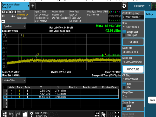
Band30_5MHz_QPSK_RB1_0_CH27735_below 18G
