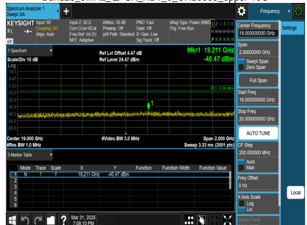
Band25_5MHz_QPSK_RB1_0_CH26065_upper 18G
