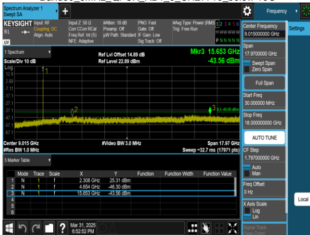
Band30_5MHz_QPSK_RB1_0_CH27710_upper 18G
