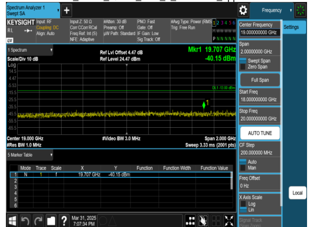
Band2_5MHz_QPSK_RB1_0_CH19175_upper 18G
