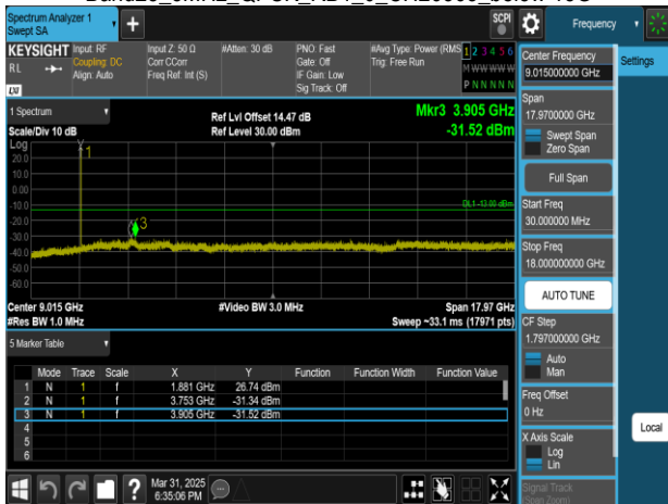
Band25_5MHz_QPSK_RB1_0_CH26365_upper 18G
