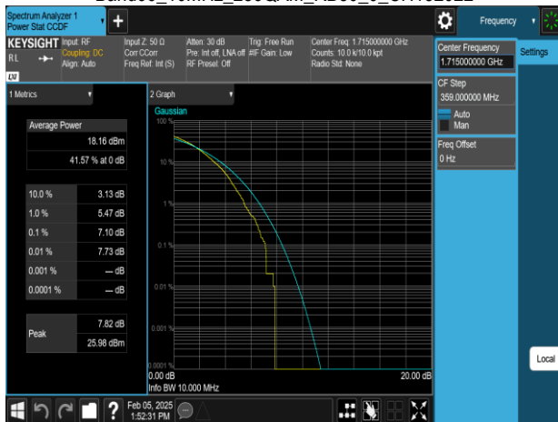
Band66_10MHz_256QAM_RB50_0_CH132022
