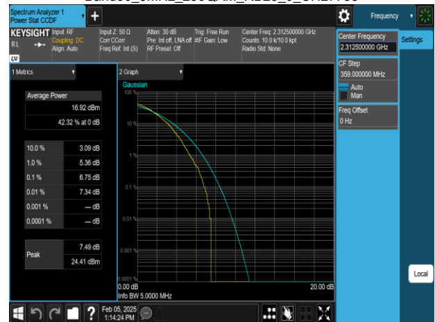
Band30_5MHz_256QAM_RB25_0_CH27735
