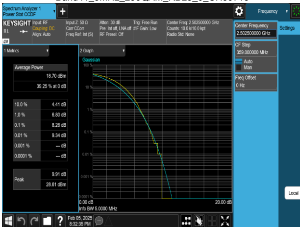
Band41 5MHz_256QAM_RB25_0_CH39715
