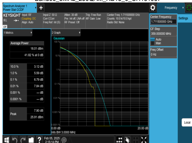
Band66 3MHz_256QAM_RB15_0_CH131987
