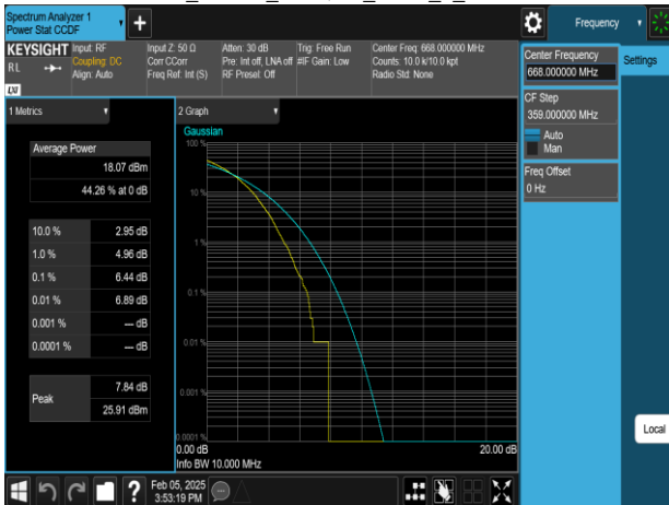
Band71_10MHz_256QAM_RB50_0_CH133172
