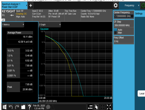
Band66 20MHz_256QAM_RB100_0_CH132072
