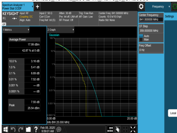
Band26_15MHz_256QAM_RB75_0_CH26965
