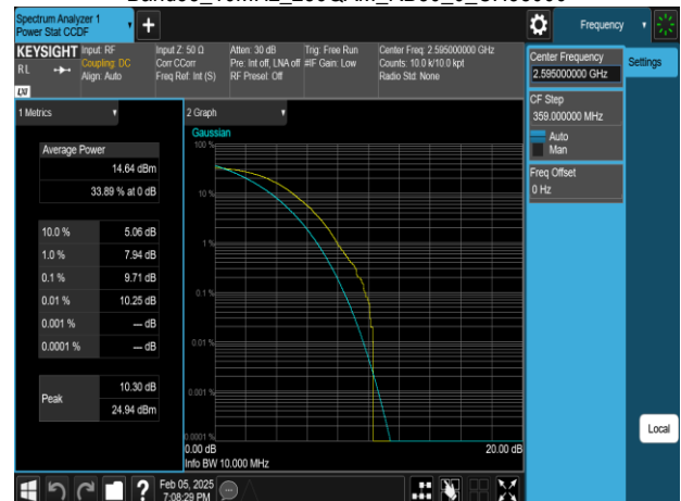
Band38_10MHz_256QAM_RB50_0_CH38000
