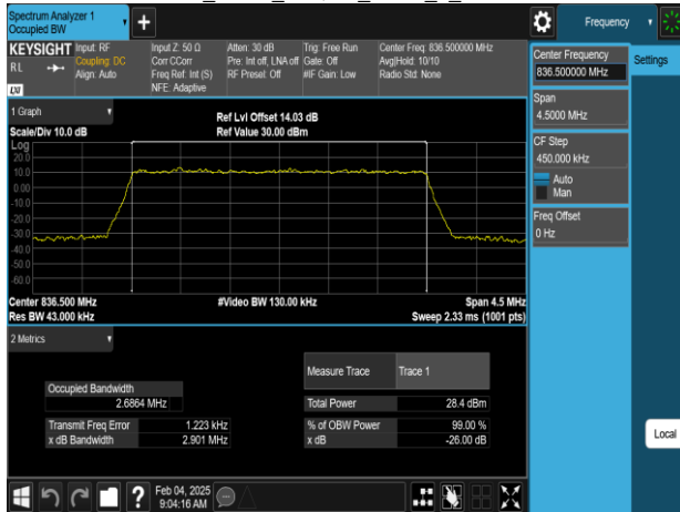
Band5_3MHz_256QAM_RB15_0_CH20525
