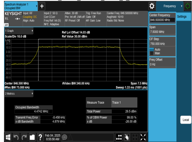
Band5_5MHz_64QAM_RB25_0_CH20625
