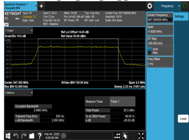
Band5_3MHz_256QAM_RB15_0_CH20635
