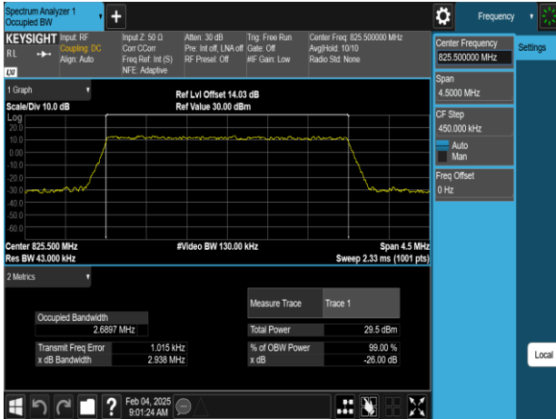
Band5_3MHz_64QAM_RB15_0_CH20415
