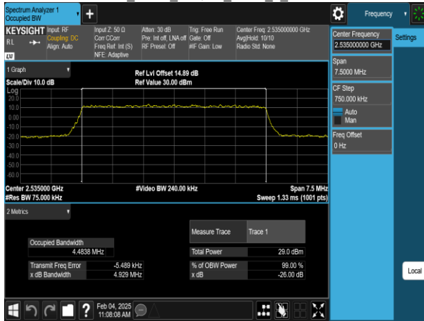
Band7_5MHz_256QAM_RB25_0_CH21100
