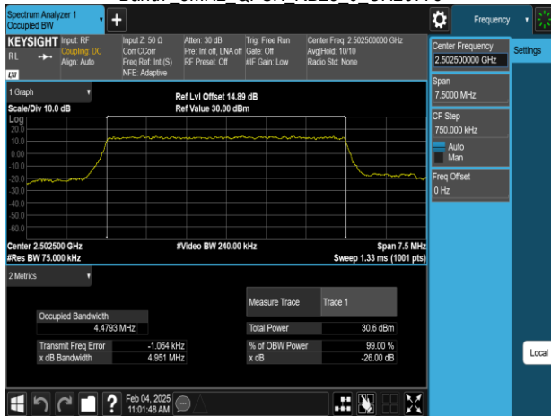
Band7_5MHz_16QAM_RB25_0_CH20775
