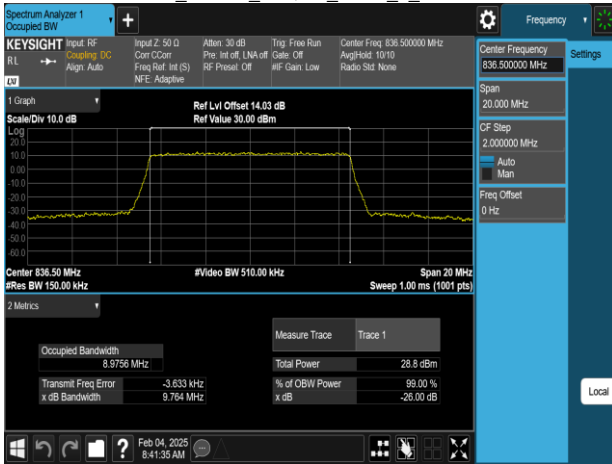
Band5_10MHz_256QAM_RB50_0_CH20525
