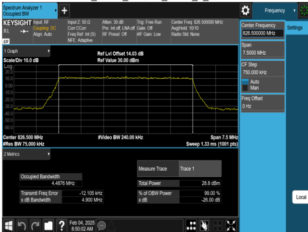
Band5_5MHz_64QAM_RB25_0_CH20425
