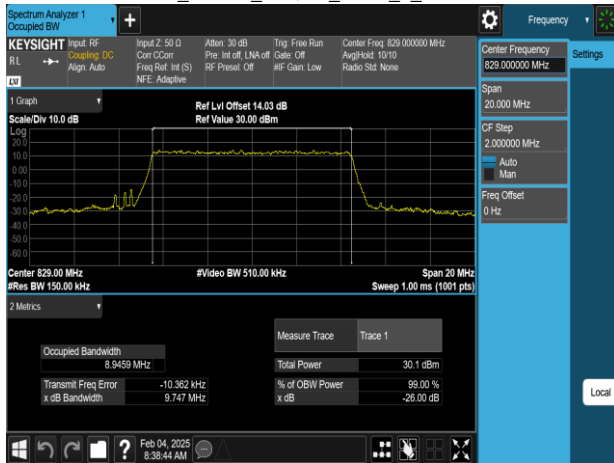
Band5_10MHz_64QAM_RB50_0_CH20450
