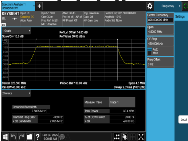
Band5_3MHz_16QAM_RB15_0_CH20415
