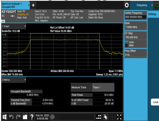
Band5_5MHz_16QAM_RB25_0_CH20425
