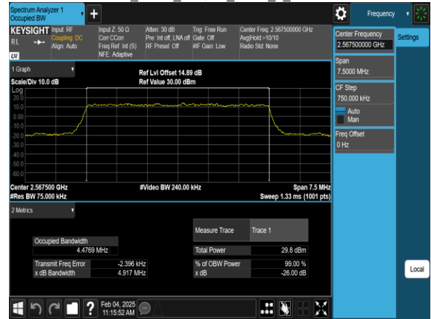
Band7_5MHz_64QAM_RB25_0_CH21425
