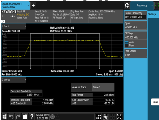
Band5_3MHz_64QAM_RB15_0_CH20415
