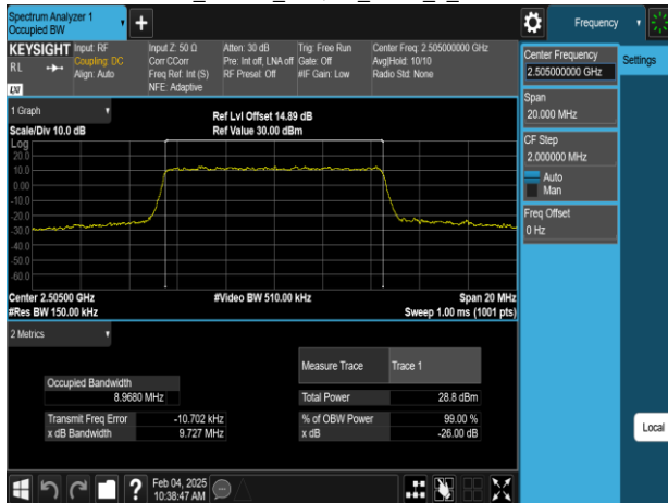
Band7_10MHz_64QAM_RB50_0_CH20800
