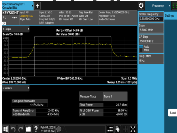
Band7_5MHz_64QAM_RB25_0_CH20775
