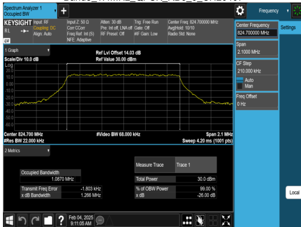
Band5 1.4MHz_16QAM_RB6_0_CH20407
