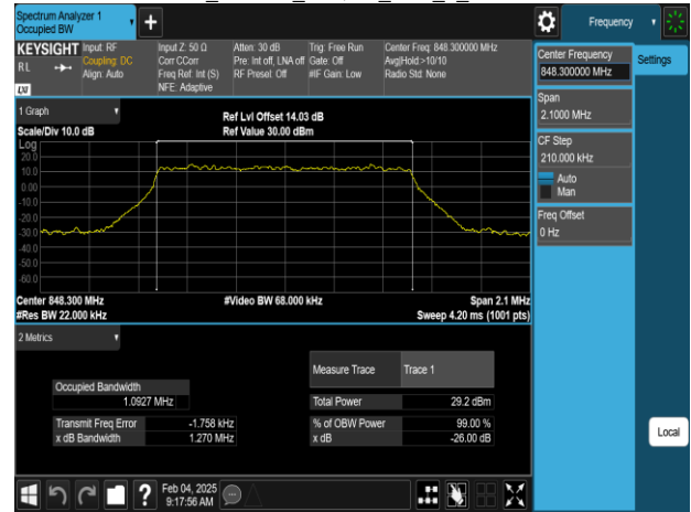
Band5_1.4MHz_64QAM_RB6_0_CH20643
