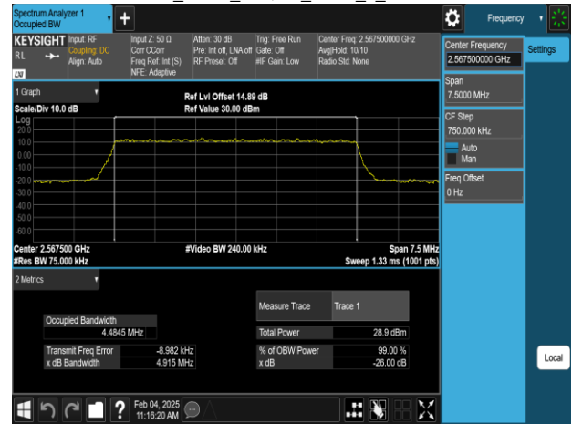
Band7_5MHz_256QAM_RB25_0_CH21425
