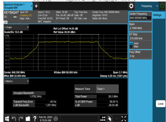
Band5_1.4MHz_256QAM_RB6_0_CH20643
