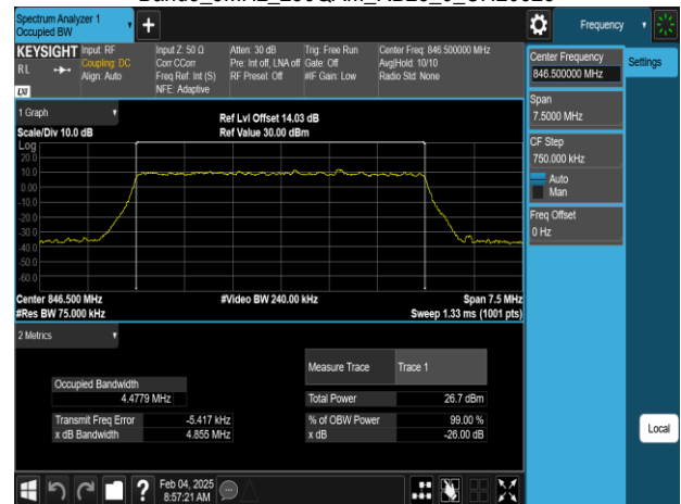
Band5_5MHz_256QAM_RB25_0_CH20625
