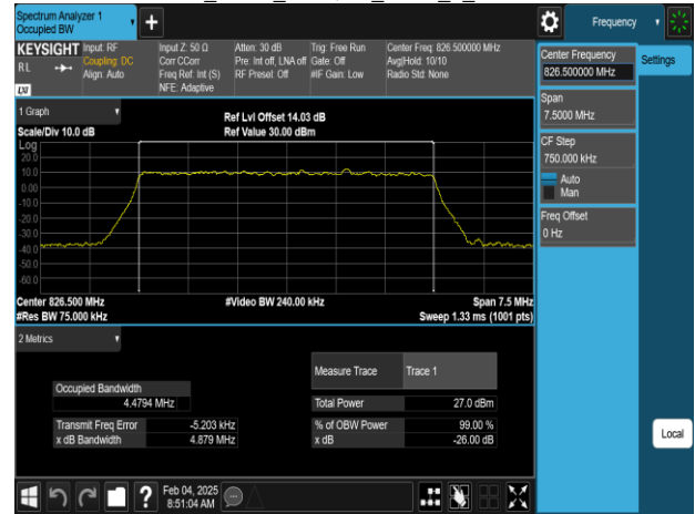
Band5_5MHz_QPSK_RB25_0_CH20525
