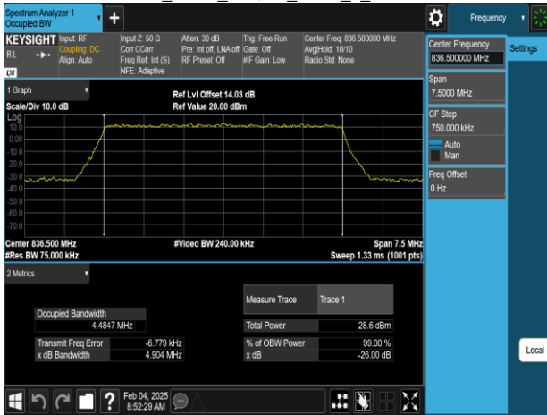
Band5_5MHz_256QAM_RB25_0_CH20525
