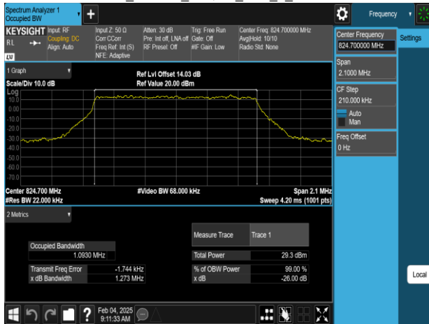
Band5 1.4MHz_64QAM_RB6_0_CH20407
