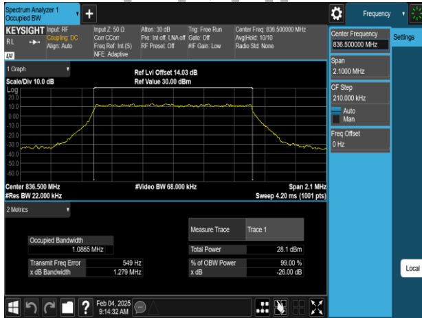
Band5_1.4MHz_256QAM_RB6_0_CH20525
