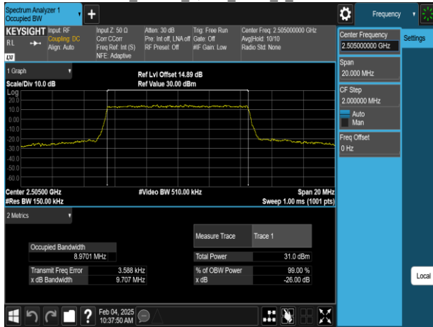
Band7_10MHz_16QAM_RB50_0_CH20800
