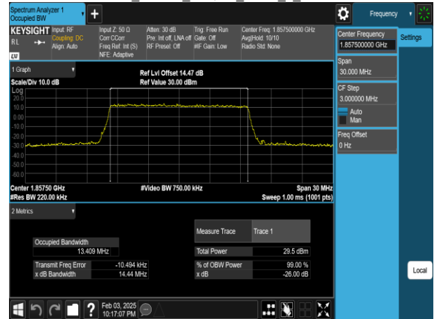
Band25_15MHz_64QAM_RB75_0_CH26115
