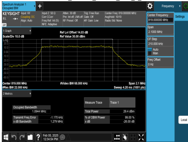
Band26-Part90s_1.4MHz_64QAM_RB6_0_CH26740
