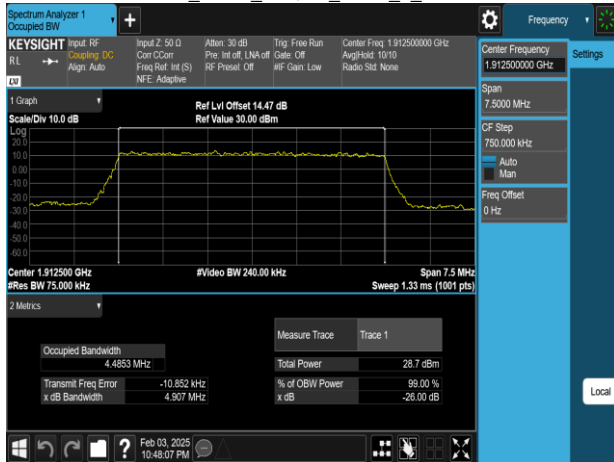
Band25_5MHz_256QAM_RB25_0_CH26665
