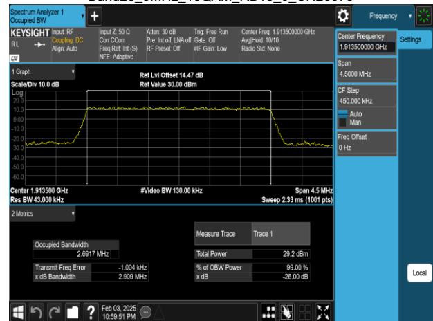
Band25_3MHz_16QAM_RB15_0_CH26675
