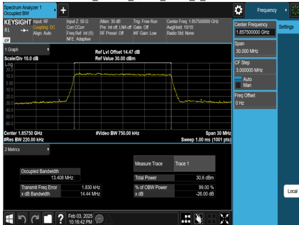
Band25_15MHz_QPSK_RB75_0_CH26115
