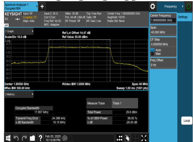
Band25_20MHz_16QAM_RB100_0_CH26590
