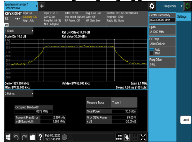
Band26-Part90s_1.4MHz_16QAM_RB6_0_CH26783
