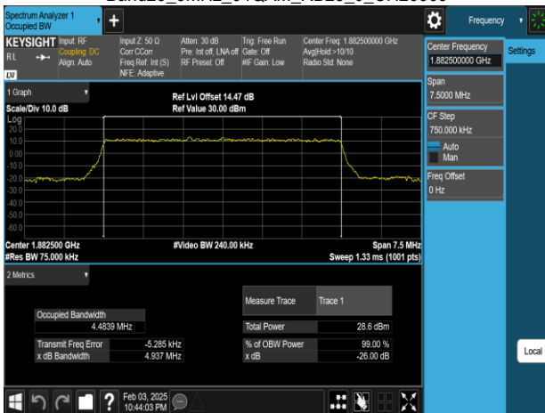
Band25_5MHz_64QAM_RB25_0_CH26365
