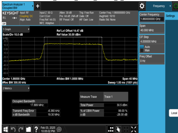
Band25_20MHz_QPSK_RB100_0_CH26140
