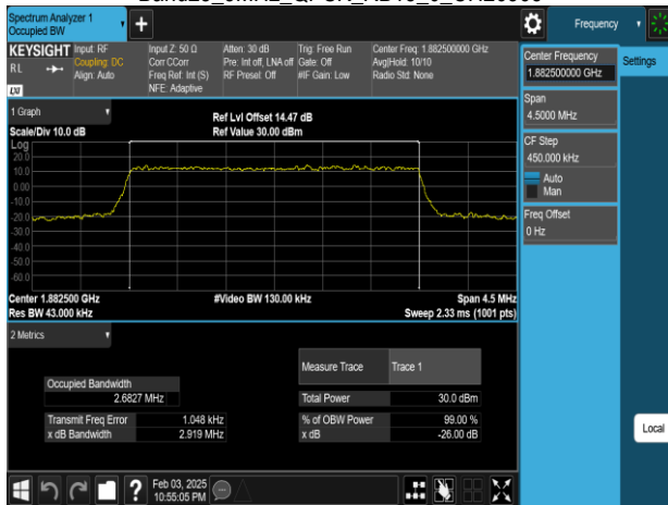
Band25_3MHz_16QAM_RB15_0_CH26365
