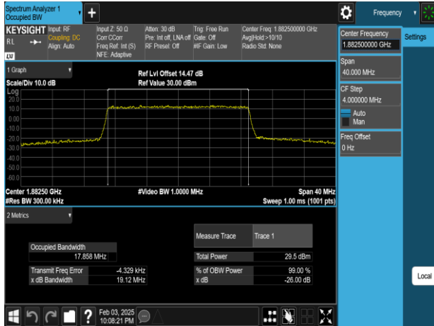
Band25_20MHz_64QAM_RB100_0_CH26365
