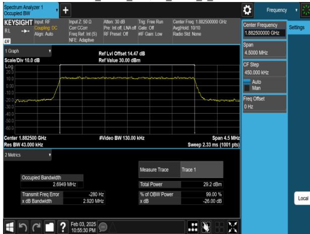
Band25_3MHz_64QAM_RB15_0_CH26365
