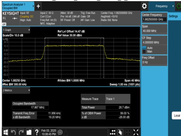
Band25_20MHz_64QAM_RB100_0_CH26365
