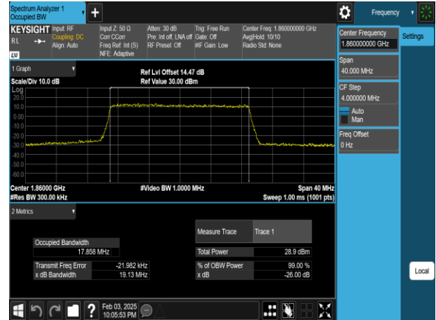
Band25_20MHz_256QAM_RB100_0_CH26140
