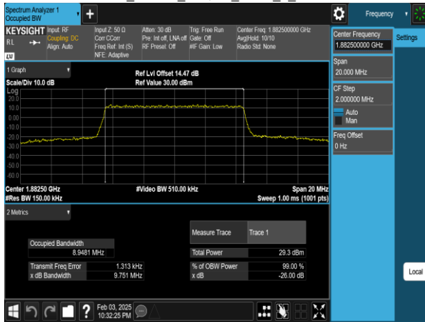
Band25_10MHz_64QAM_RB50_0_CH26365
