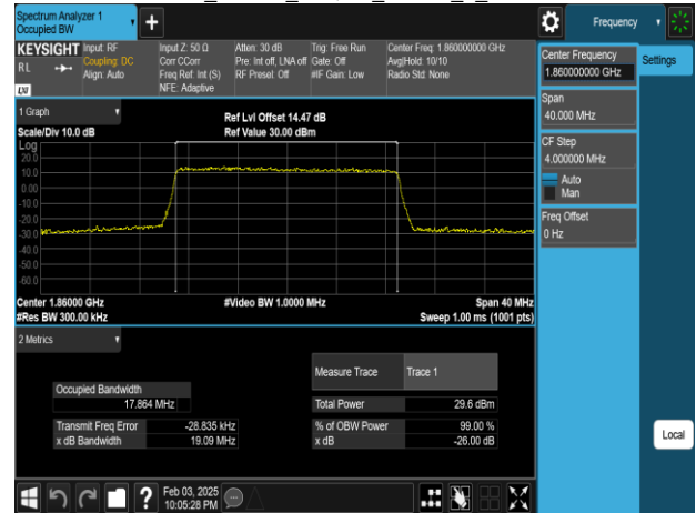
Band25_20MHz_64QAM_RB100_0_CH26140
