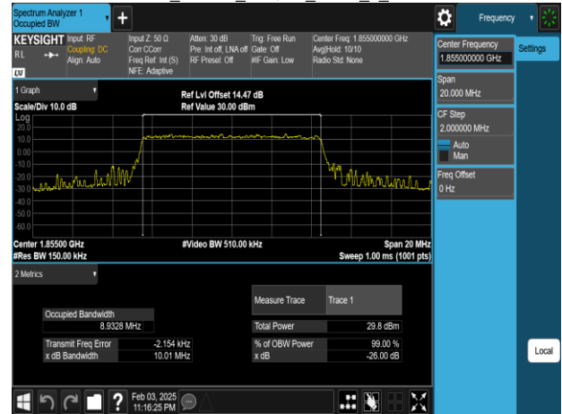
Band25_10MHz_64QAM_RB50_0_CH26090
