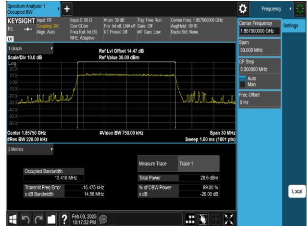
Band25_15MHz_256QAM_RB75_0_CH26115
