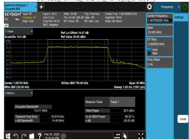
Band25_15MHz_16QAM_RB75_0_CH26615
