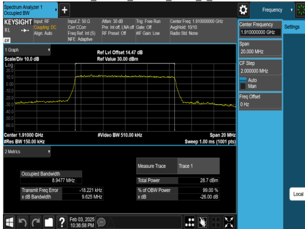
Band25_10MHz_256QAM_RB50_0_CH26640
