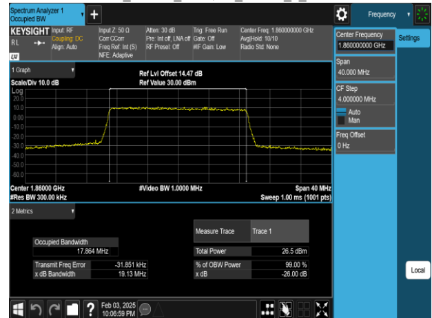
Band25_20MHz_256QAM_RB100_0_CH26140
