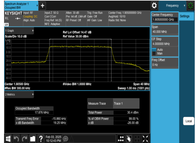
Band25_20MHz_16QAM_RB100_0_CH26590
