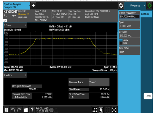
Band26-Part90s_1.4MHz_256QAM_RB6_0_CH26697
