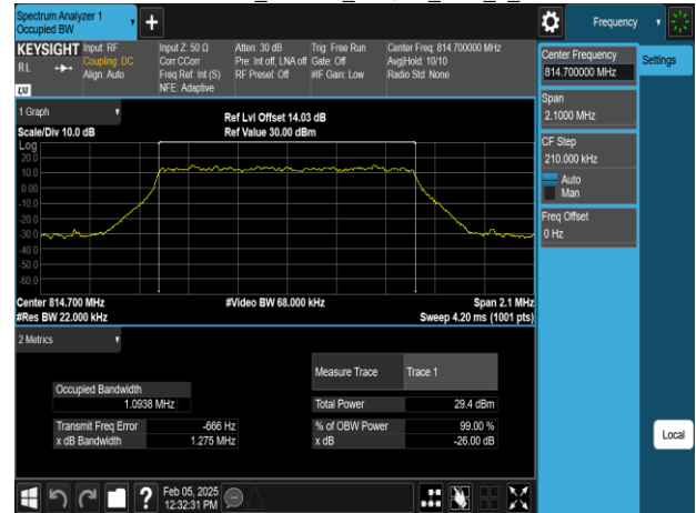
Band26-Part90s_1.4MHz_64QAM_RB6_0_CH26697
