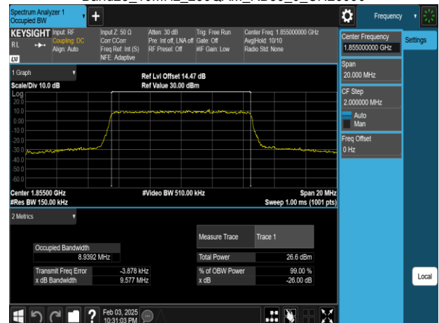
Band25_10MHz_256QAM_RB50_0_CH26090
