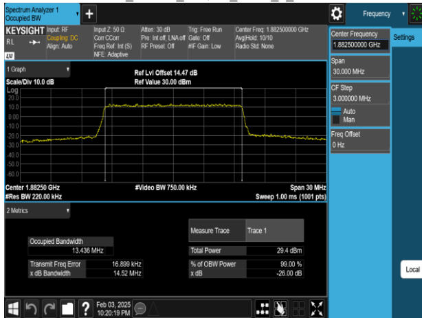
Band25_15MHz_64QAM_RB75_0_CH26365
