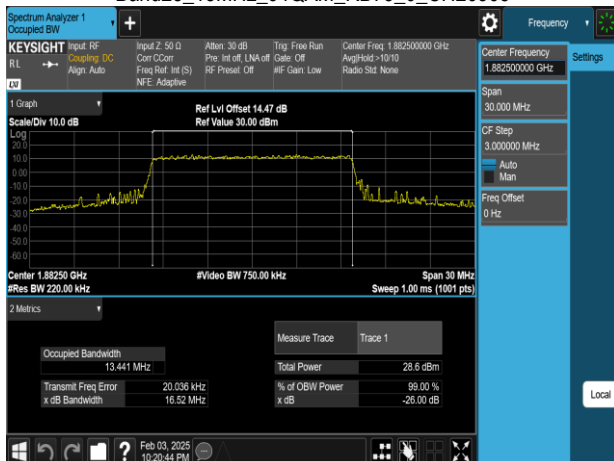
Band25_15MHz_64QAM_RB75_0_CH26365
