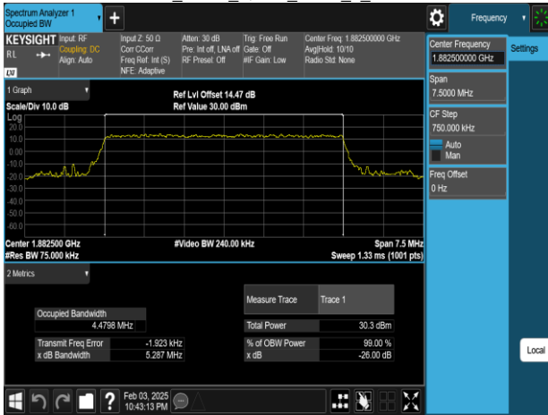
Band25_5MHz_16QAM_RB25_0_CH26365
