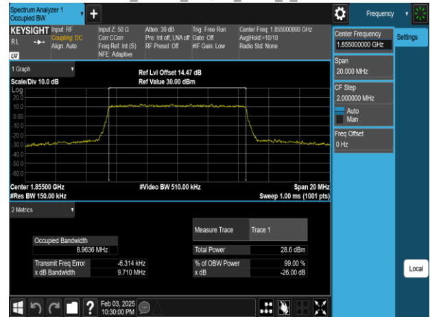
Band25_10MHz_256QAM_RB50_0_CH26090
