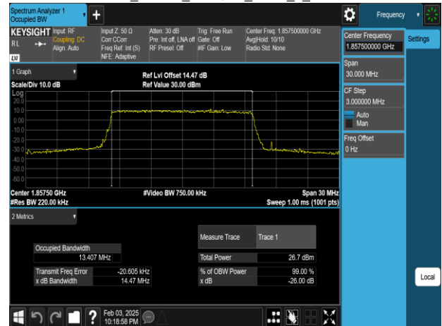
Band25_15MHz_256QAM_RB75_0_CH26115
