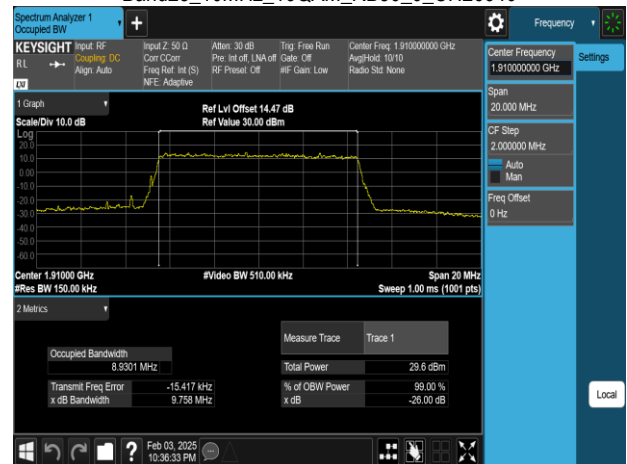
Band25_10MHz_16QAM_RB50_0_CH26640
