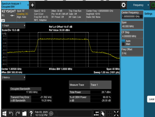
Band25_20MHz_256QAM_RB100_0_CH26590
