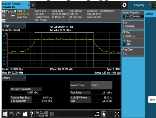
Band25 1.4MHz 256QAM_RB6_0_CH26683
