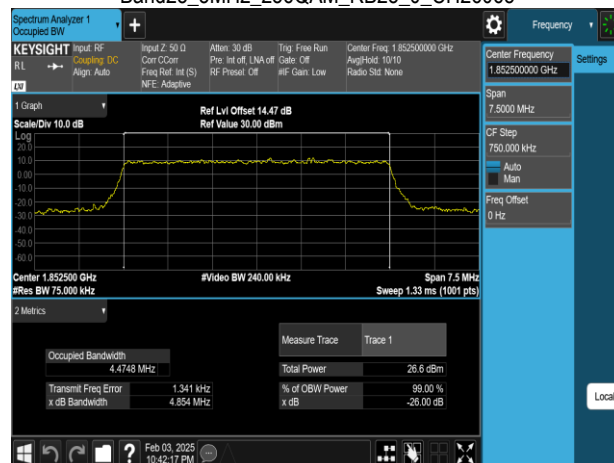
Band25_5MHz_256QAM_RB25_0_CH26065
