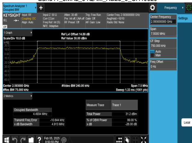
Band41_5MHz_64QAM_RB25_0_CH40620
