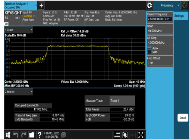
Band38_20MHz_256QAM_RB100_0_CH38000
