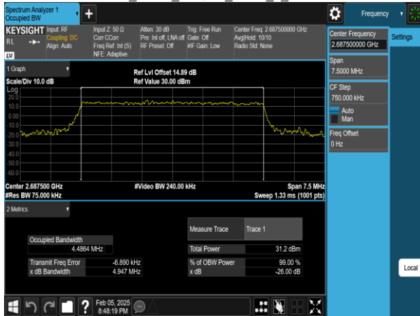
Band41_5MHz_256QAM_RB25_0_CH41565
