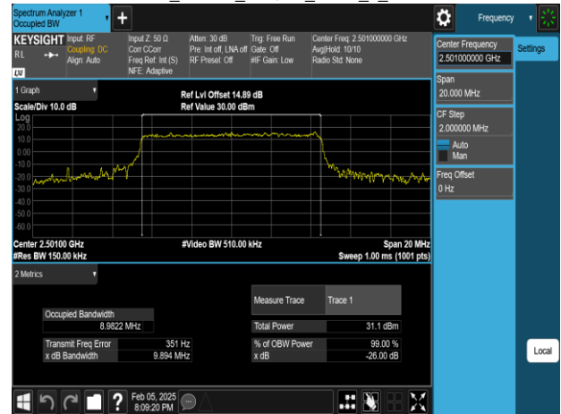
Band41_10MHz_256QAM_RB50_0_CH39700
