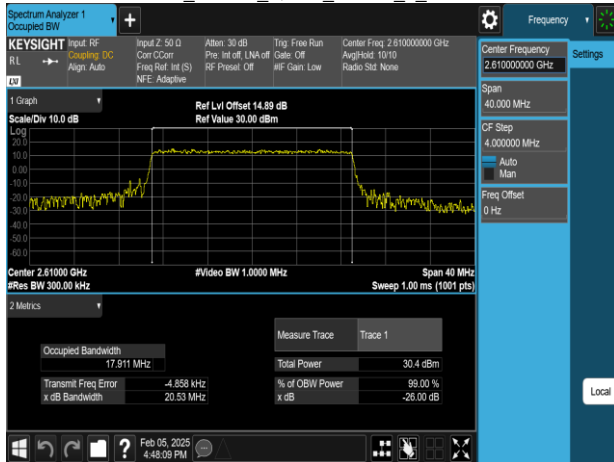
Band38_20MHz_16QAM_RB100_0_CH38150
