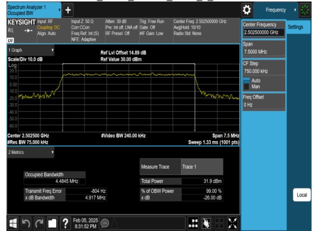
Band41_5MHz_64QAM_RB25_0_CH39715
