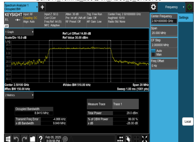
Band41_10MHz_256QAM_RB50_0_CH39700
