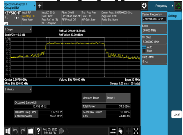
Band41_15MHz_16QAM_RB75_0_CH39765
