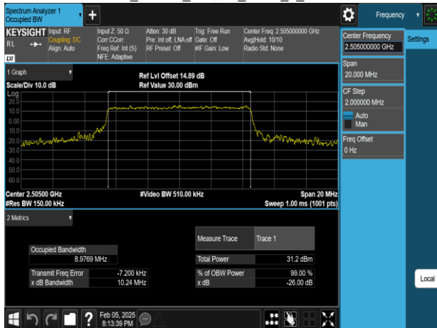
Band41_10MHz_64QAM_RB50_0_CH39740
