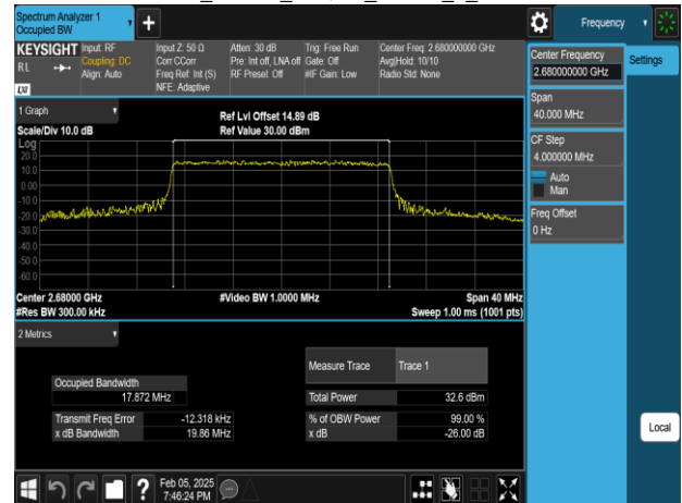
Band41_20MHz_16QAM_RB100_0_CH41490
