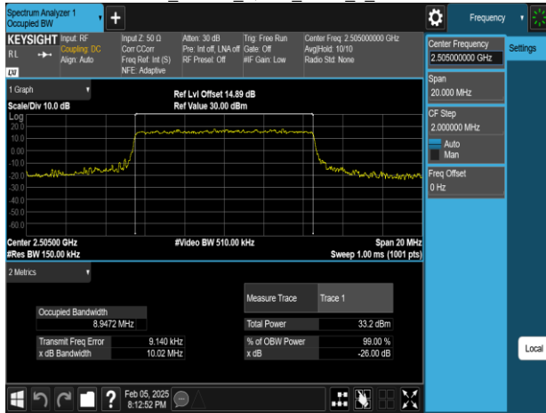
Band41_10MHz_16QAM_RB50_0_CH39740
