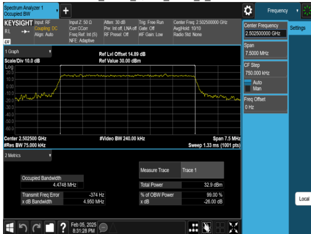
Band41_5MHz_QPSK_RB25_0_CH39715
