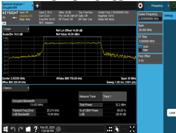
Band41_15MHz_64QAM_RB75_0_CH39725
