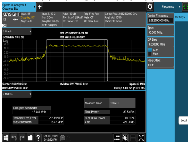
Band41 15MHz 16QAM_RB75_0_CH41515
