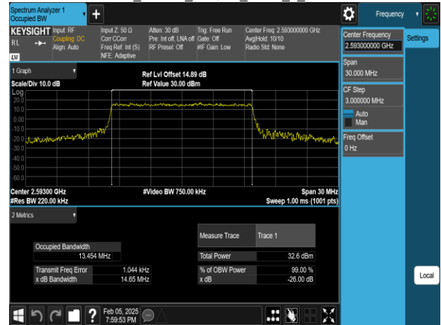
Band41_15MHz_64QAM_RB75_0_CH40620
