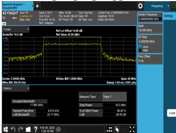
Band38_20MHz_QPSK_RB100_0_CH38000
