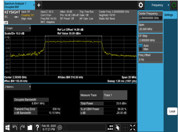
Band41_10MHz_16QAM_RB50_0_CH40620
