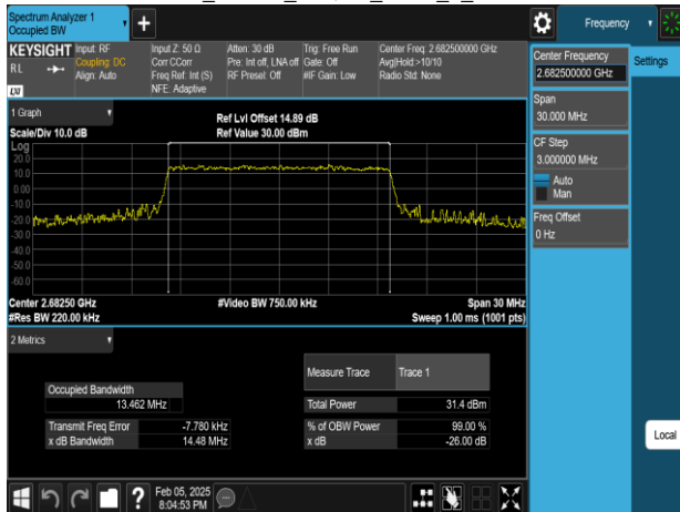
Band41 15MHz 64QAM_RB75_0_CH41515
