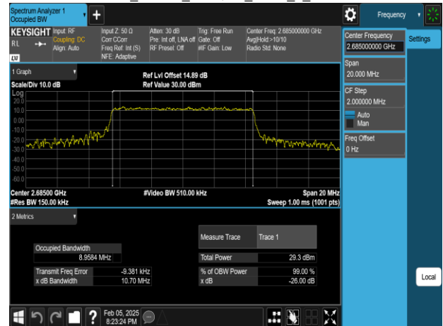
Band41_10MHz_256QAM_RB50_0_CH41540
