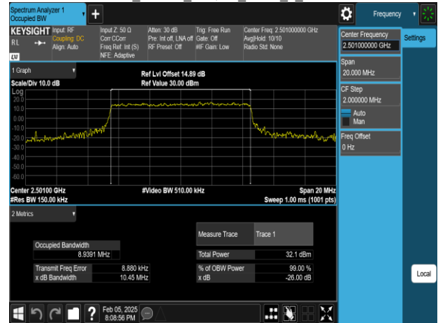
Band41_10MHz_64QAM_RB50_0_CH39700
