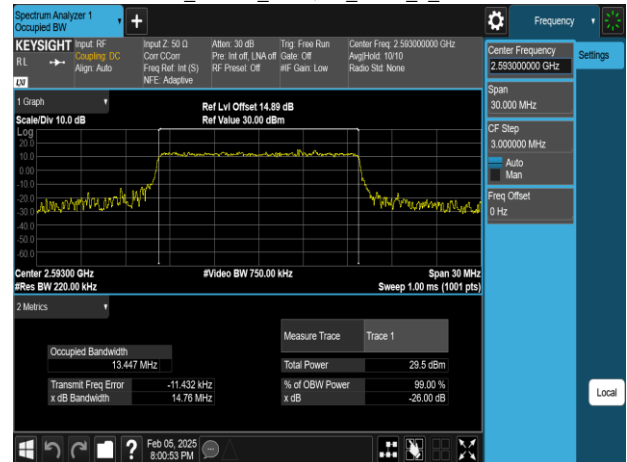
Band41_15MHz_256QAM_RB75_0_CH40620
