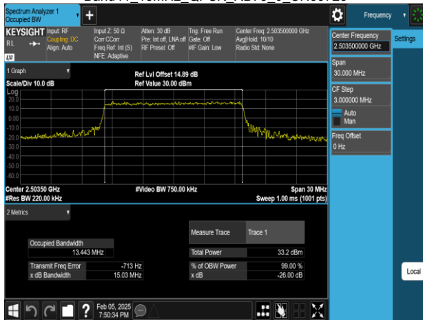
Band41_15MHz_16QAM_RB75_0_CH39725
