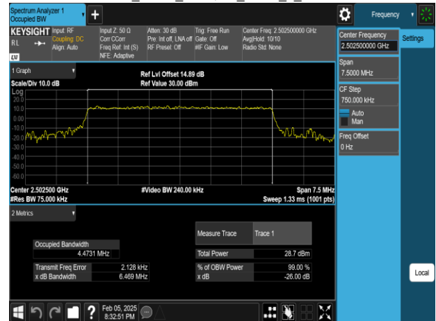
Band41_5MHz_256QAM_RB25_0_CH39715
