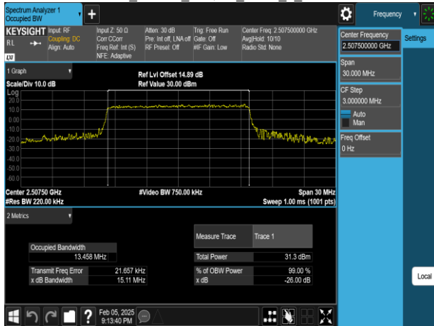
Band41_15MHz_256QAM_RB75_0_CH39765
