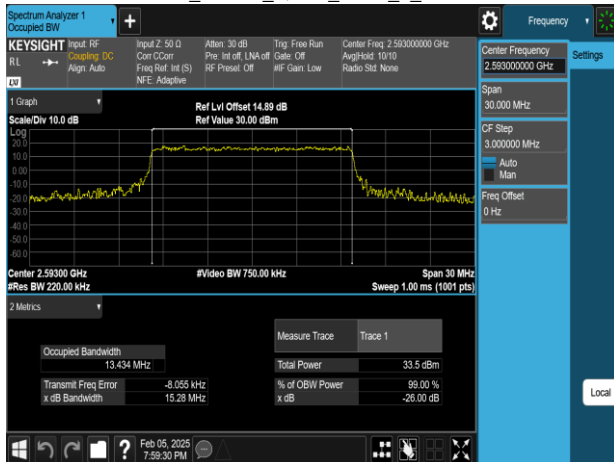
Band41_15MHz_QPSK_RB75_0_CH40620
