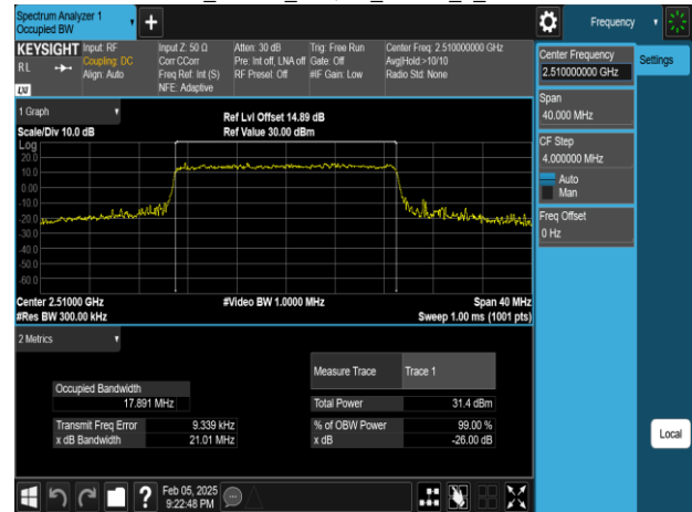
Band41_20MHz_256QAM_RB100_0_CH39790
