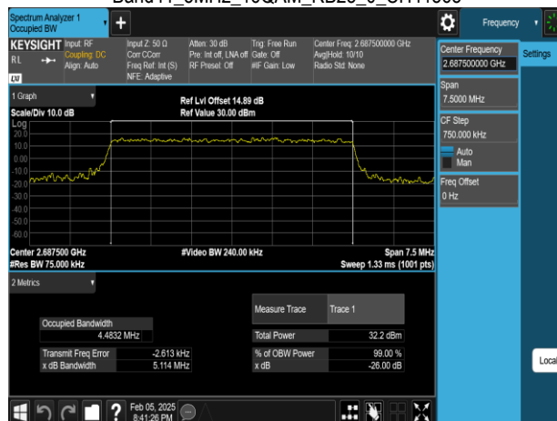
Band41_5MHz_16QAM_RB25_0_CH41565
