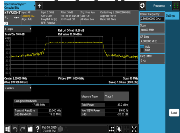
Band41 20MHz 16QAM_RB100_0_CH39750
