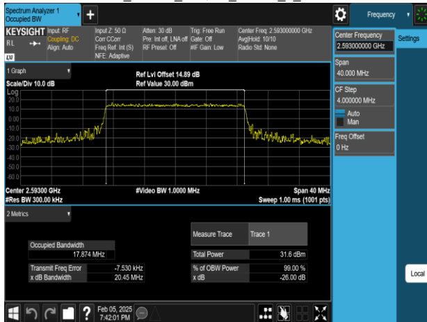
Band41_20MHz_64QAM_RB100_0_CH40620
