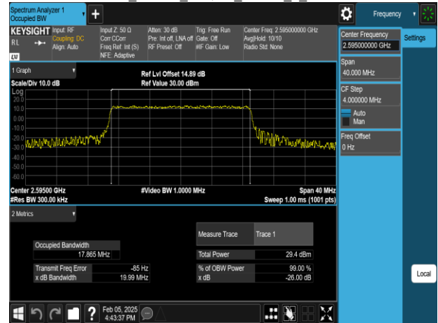
Band38_20MHz_64QAM_RB100_0_CH38000
