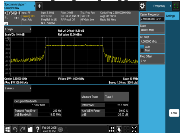
Band38_20MHz_256QAM_RB100_0_CH38000
