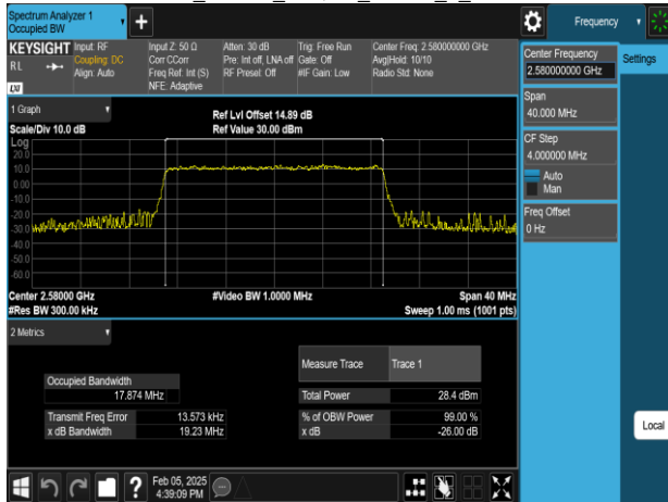
Band38_20MHz_256QAM_RB100_0_CH37850
