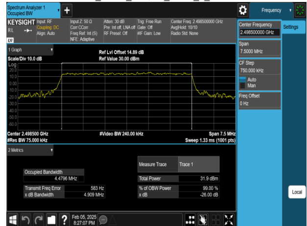
Band41_5MHz_16QAM_RB25_0_CH39675
