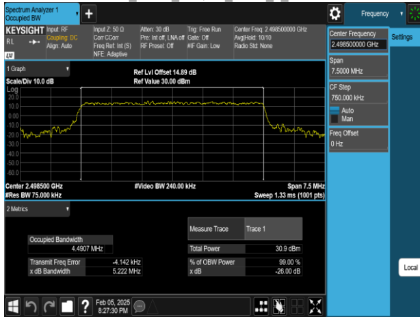
Band41_5MHz_256QAM_RB25_0_CH39675
