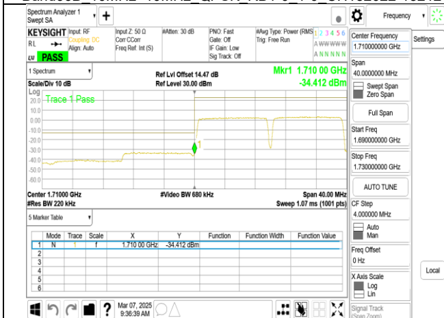
Band66B 10MHz+10MHz QPSK RB50-0 50-0 CH132022-132121
