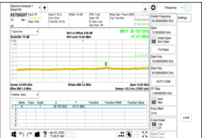
Band38_15MHz+15MHz_QPSK_RB1-74_1-0_CH37825-37975_up-per 18G
