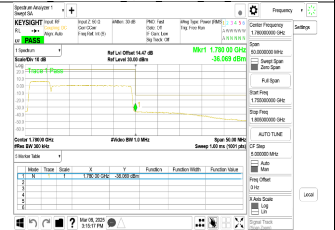
Band66 5MHz+20MHz QPSK RB25-0 100-0 CH132455-132572
