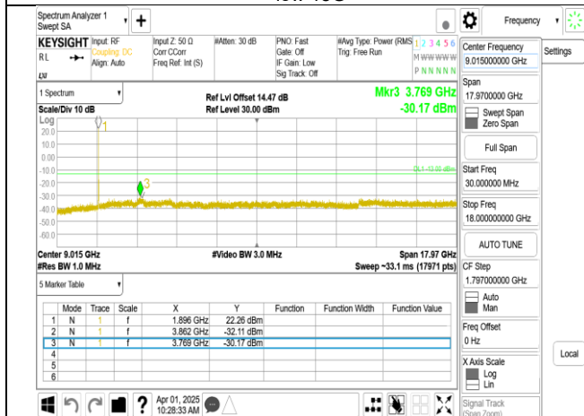
Band2_15MHz+15MHz_QPSK_RB1-74_1-0_CH18975-19125_low 18G
