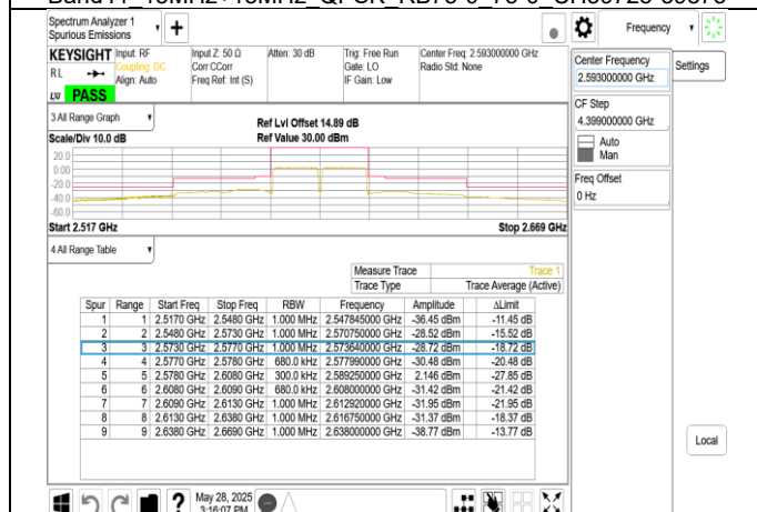
Band41 15MHz+15MHz QPSK RB75-0 75-0 CH40545-40695
