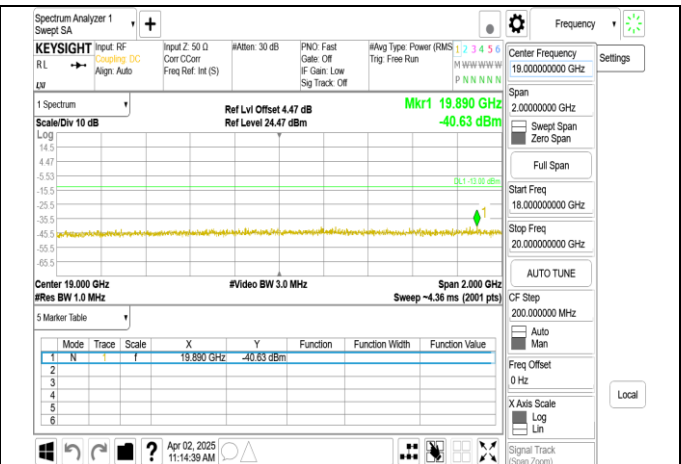
Band2_15MHz+15MHz_QPSK_RB1-74_1-0_CH18675-18825_up per 18G
