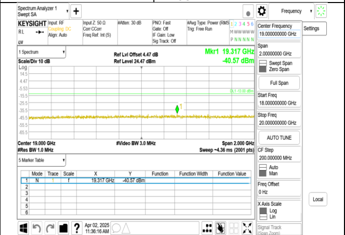
Band2_15MHz+15MHz_QPSK_RB1-74_1-0_CH18825-18975_up per 18G
