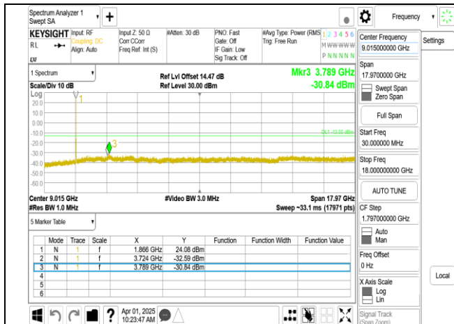
Band2_15MHz+15MHz_QPSK_RB1-74_1-0_CH18675-18825_low 18G
