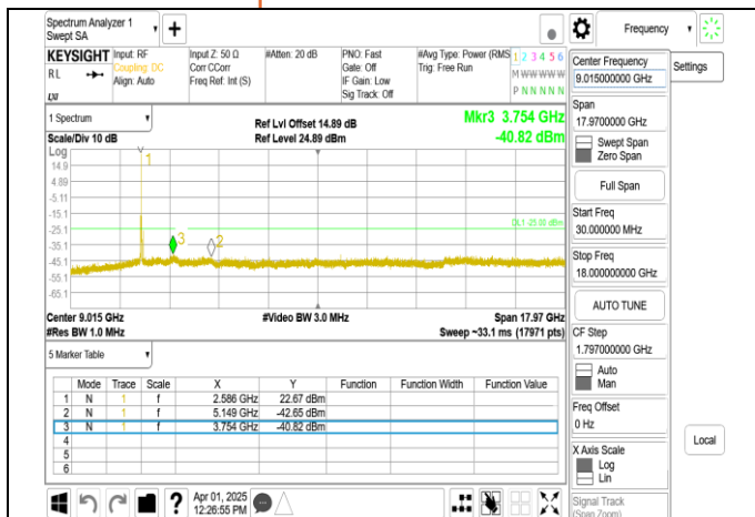
Band38_15MHz+15MHz_QPSK_RB1-74_1-0_CH37825-37975_be-low 18G
