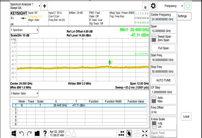
Band38_15MHz+15MHz_QPSK_RB1-74_1-0_CH38025-38175_up-per 18G
