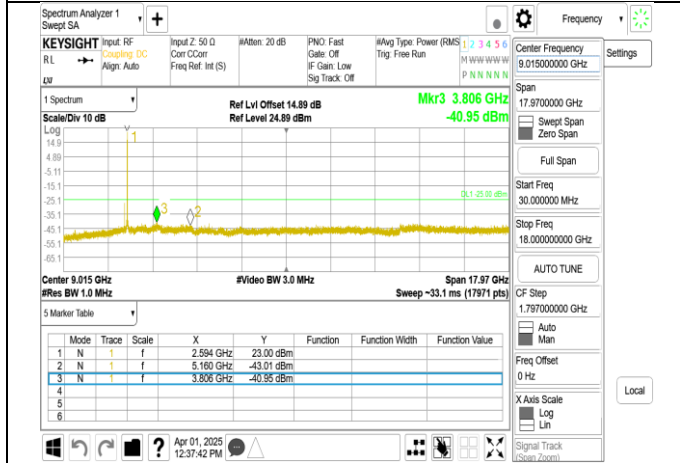
Band38_15MHz+15MHz_QPSK_RB1-74_1-0_CH37925-38075_be-low 18G
