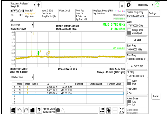
Band38_15MHz+15MHz_QPSK_RB1-74_1-0_CH38025-38175_be-low 18G
