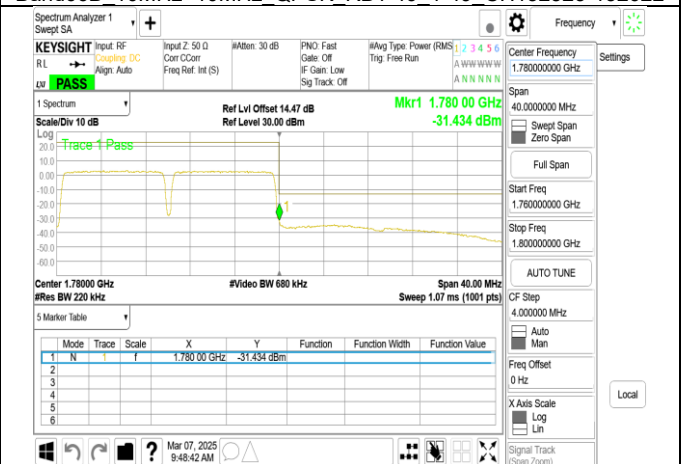
Band66B 10MHz+10MHz QPSK RB50-0 50-0 CH132523-132622
