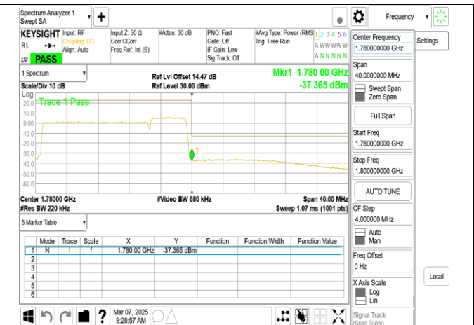
Band66B 15MHz+5MHz QPSK RB75-0 25-0 CH132549-132642
