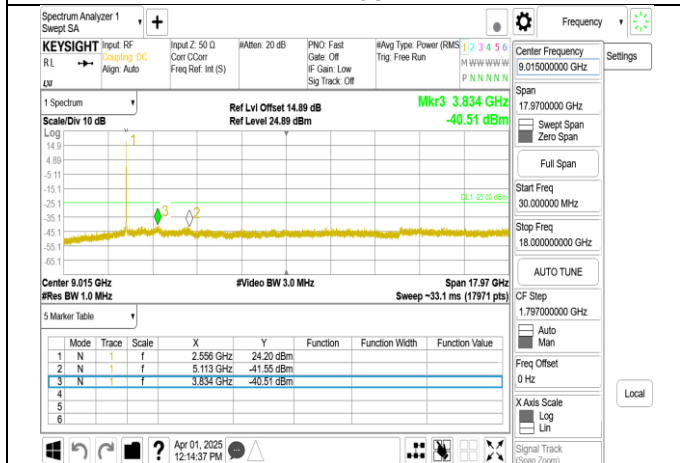
Band7_15MHz+15MHz_QPSK_RB1-74_1-0_CH21225-21375_low 18G
