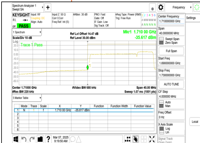
Band66B 15MHz+5MHz QPSK RB75-0 25-0 CH132047-132140
