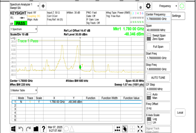
Band66B 15MHz+5MHz QPSK RB1-74 1-24 CH132549-132642
