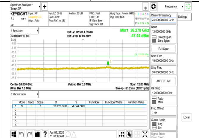
Band7_15MHz+15MHz_QPSK_RB1-74_1-0_CH21225-21375_up per 18G
