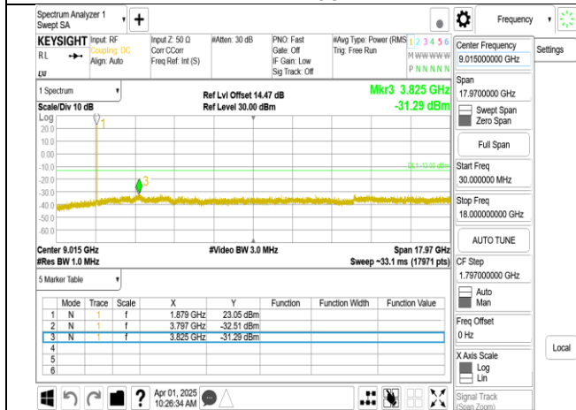
Band2_15MHz+15MHz_QPSK_RB1-74_1-0_CH18825-18975_low 18G
