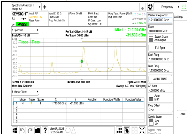
Band66B 10MHz+10MHz QPSK RB1-0 1-0 CH132022-132121
