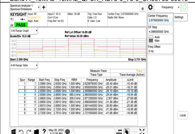
Band41 15MHz+15MHz QPSK RB75-0 75-0 CH41365-41515
