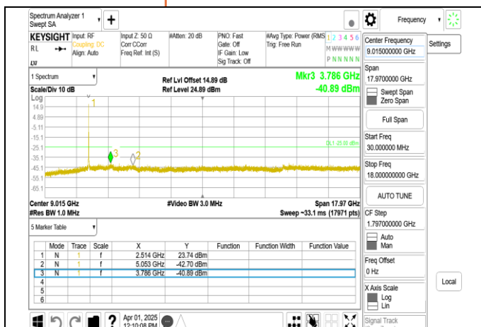
Band7_15MHz+15MHz_QPSK_RB1-74_1-0_CH20825-20975_low 18G
