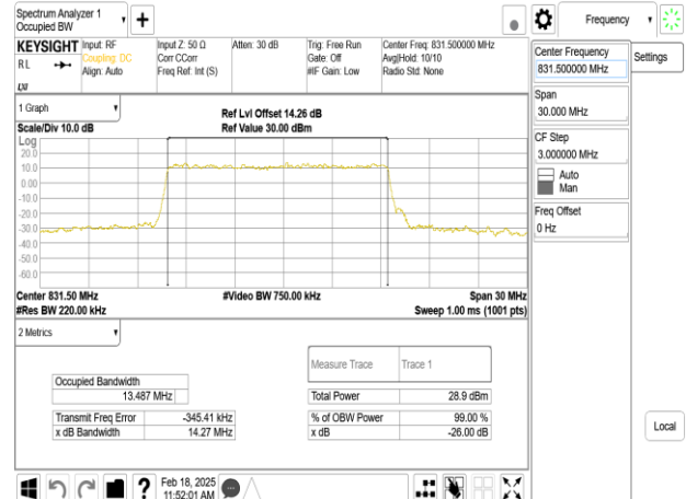
Band26_15MHz_DFT_s_OFDM_SCS15kHz_64QAM_RB75_0_CH166300
