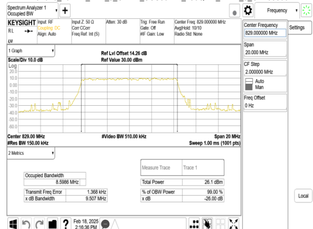
Band26_10MHz_DFT_s_OFDM_SCS30kHz_256QAM_RB24_0_CH165800
