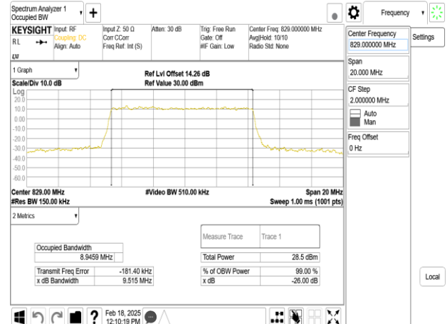
Band26_10MHz_DFT_s_OFDM_SCS15kHz_64QAM_RB50_0_CH165800
