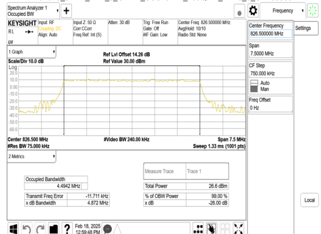
Band26_5MHz_DFT_s_OFDM_SCS15kHz_256QAM_RB25_0_CH165300
