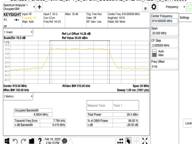
Band26-Part90s_10MHz_DFT_s_OFDM_SCS30kHz_256QAM_RB24_0_CH163800
