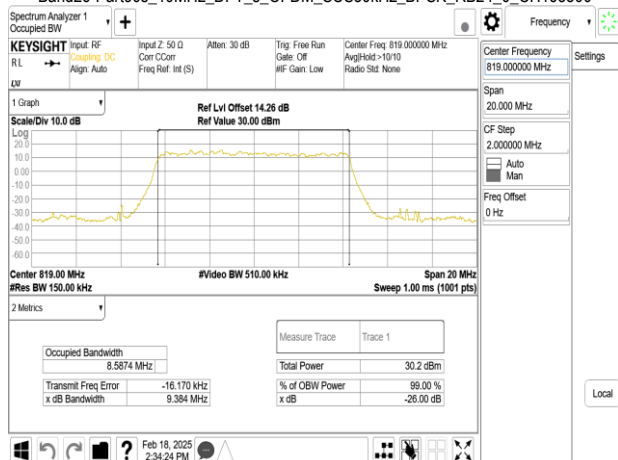
Band26-Part90s_10MHz_DFT_s_OFDM_SCS30kHz_QPSK_RB24_0_CH163800
