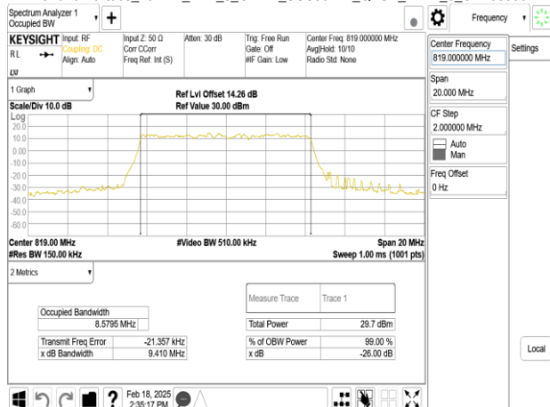
Band26-Part90s_10MHz_DFT_s_OFDM_SCS30kHz_16QAM_RB24_0_CH163800
