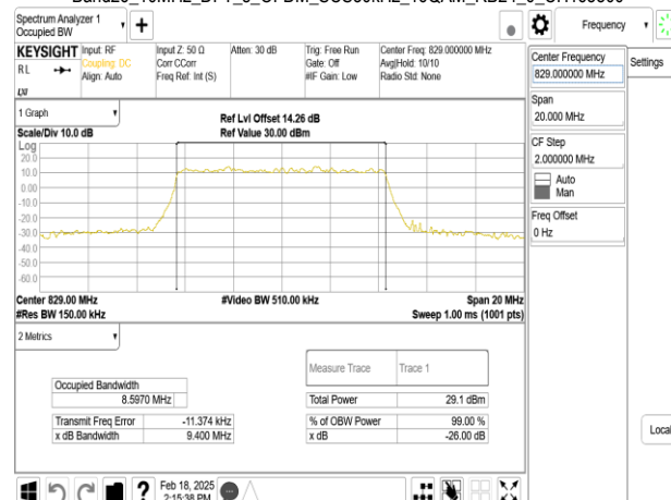
Band26_10MHz_DFT_s_OFDM_SCS30kHz_16QAM_RB24_0_CH165800
