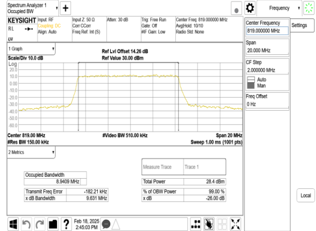
Band26-Part90s_10MHz_DFT_s_OFDM_SCS15kHz_256QAM_RB50_0_CH163800
