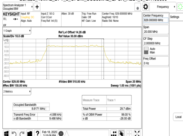
Band26_10MHz_DFT_s_OFDM_SCS30kHz_QPSK_RB24_0_CH165800
