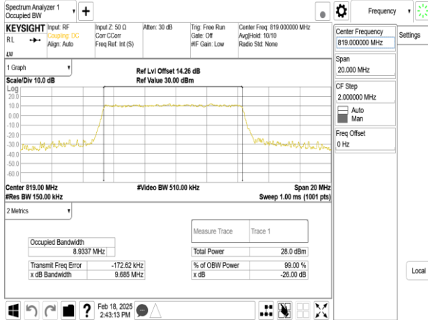
Band26-Part90s_10MHz_DFT_s_OFDM_SCS15kHz_QPSK_RB50_0_CH163800
