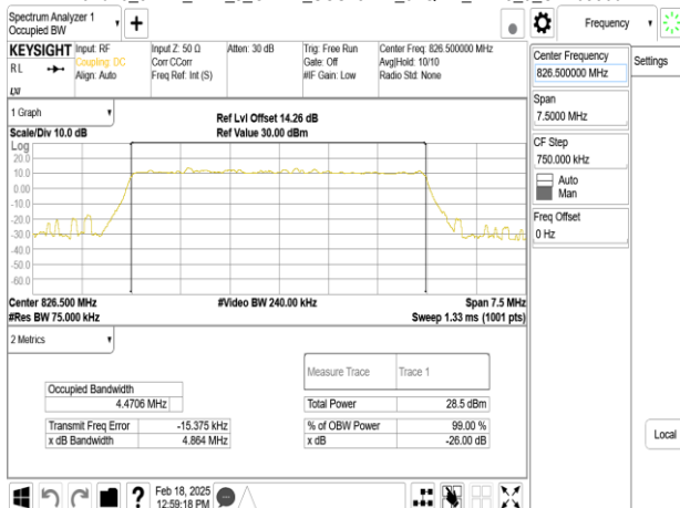
Band26_5MHz_DFT_s_OFDM_SCS15kHz_64QAM_RB25_0_CH165300
