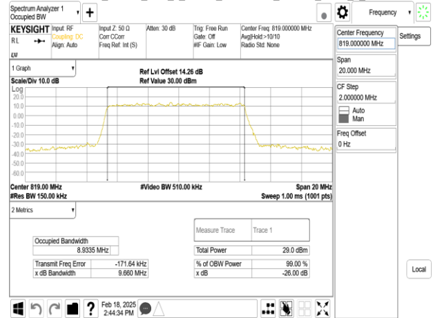
Band26-Part90s_10MHz_DFT_s_OFDM_SCS15kHz_64QAM_RB50_0_CH163800
