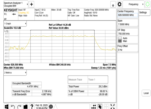
Band26_5MHz_DFT_s_OFDM_SCS15kHz_16QAM_RB25_0_CH165300
