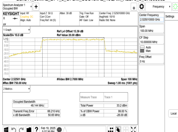
Band41_50MHz_DFT_s_OFDM_SCS15kHz_16QAM_RB270_0_CH505002
