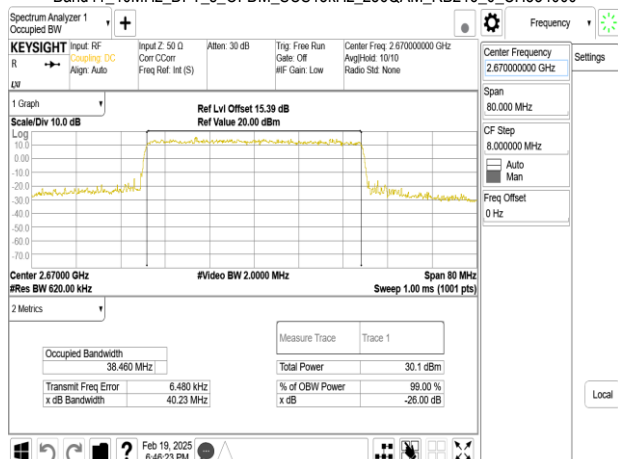
Band41_40MHz_DFT_s_OFDM_SCS15kHz_256QAM_RB216_0_CH534000
