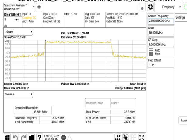
Band41_40MHz_DFT_s_OFDM_SCS15kHz_16QAM_RB216_0_CH518604
