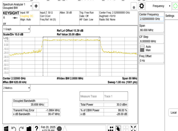
Band41_40MHz_DFT_s_OFDM_SCS30kHz_256QAM_RB100_0_CH504000
