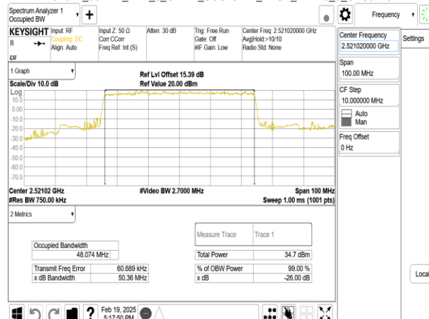
Band41_50MHz_DFT_s_OFDM_SCS15kHz_BPSK_RB270_0_CH504204
