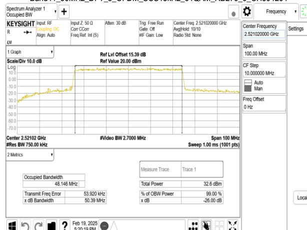
Band41_50MHz_DFT_s_OFDM_SCS15kHz_64QAM_RB270_0_CH504204
