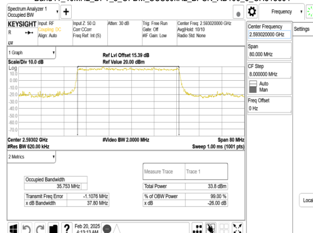
Band41_40MHz_DFT_s_OFDM_SCS30kHz_BPSK_RB100_0_CH518604
