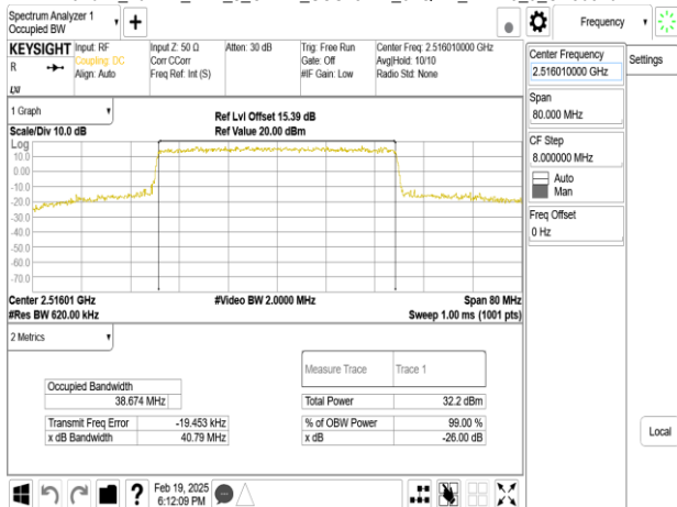
Band41_40MHz_DFT_s_OFDM_SCS15kHz_64QAM_RB216_0_CH504000
