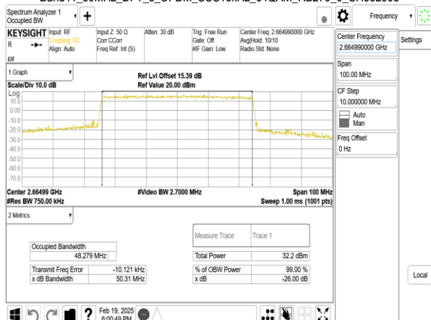
Band41_50MHz_DFT_s_OFDM_SCS15kHz_64QAM_RB270_0_CH532998
