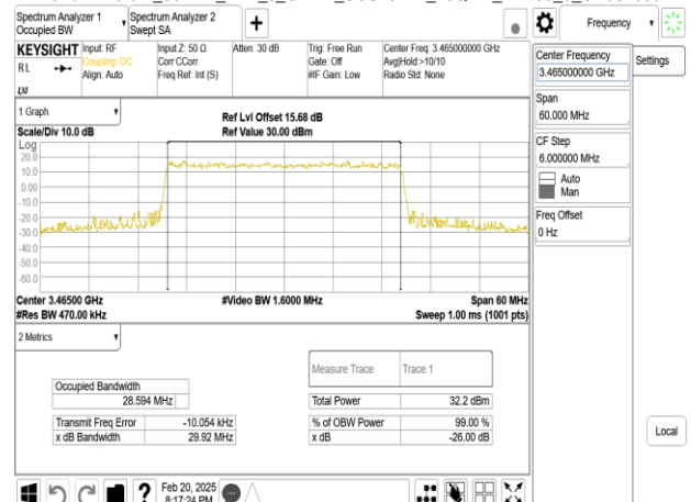
Band77-Part27_30MHz_DFT_s_OFDM_SCS15kHz_16QAM_RB160_0_CH631000
