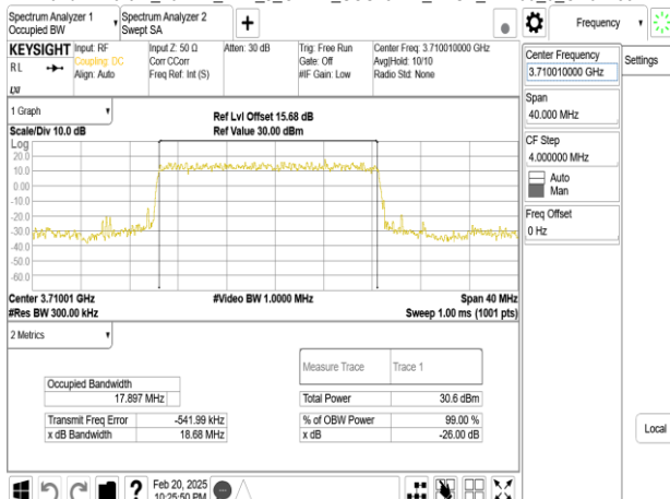
Band77-Part27_20MHz_DFT_s_OFDM_SCS15kHz_BPSK_RB100_0_CH647334
