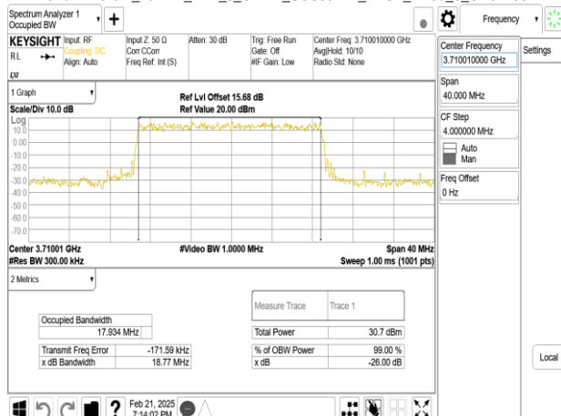
Band77-Part27_20MHz_DFT_s_OFDM_SCS30kHz_BPSK_RB50_0_CH647334
