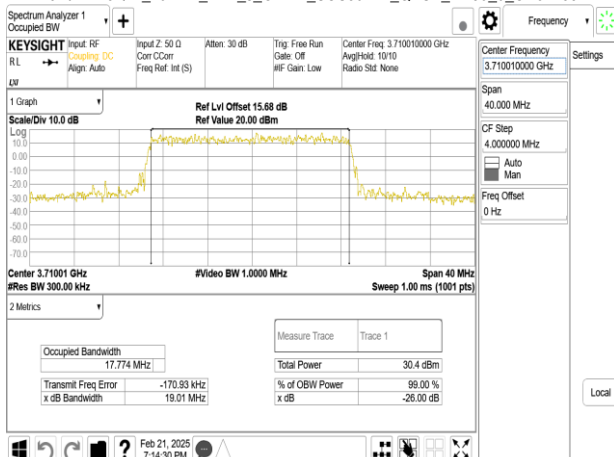
Band77-Part27_20MHz_DFT_s_OFDM_SCS30kHz_QPSK_RB50_0_CH647334
