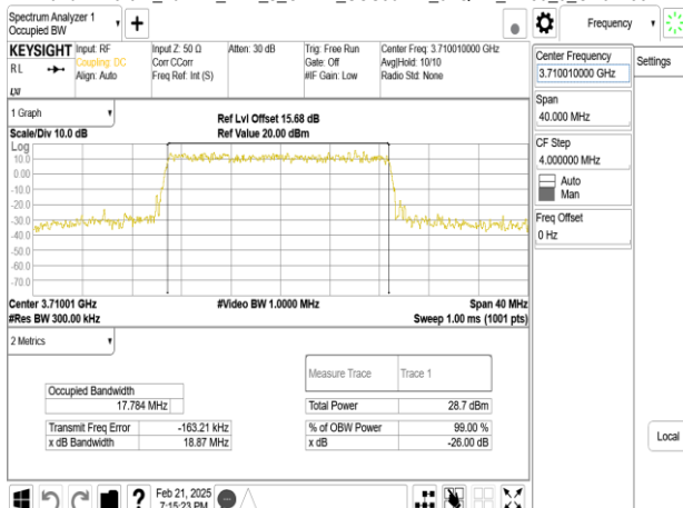
Band77-Part27_20MHz_DFT_s_OFDM_SCS30kHz_64QAM_RB50_0_CH647334
