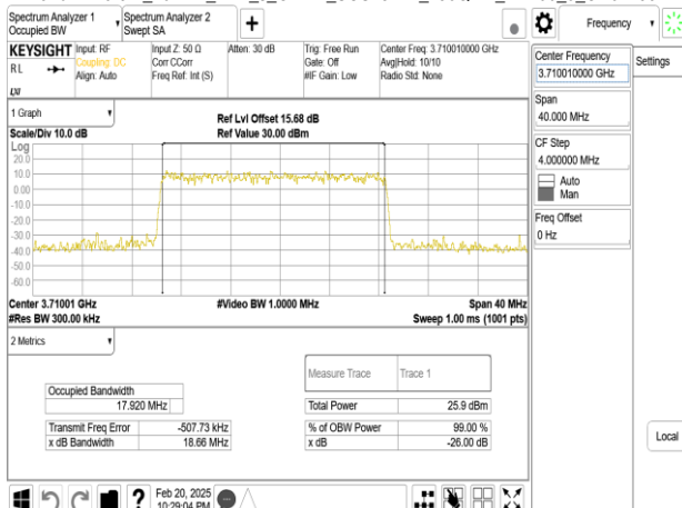
Band77-Part27_20MHz_DFT_s_OFDM_SCS15kHz_256QAM_RB100_0_CH647334
