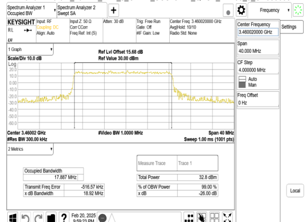
Band77-Part27_20MHz_DFT_s_OFDM_SCS15kHz_QPSK_RB100_0_CH630668
