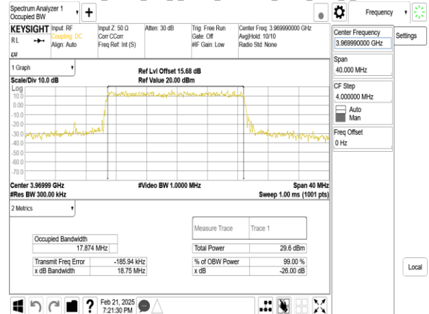
Band77-Part27_20MHz_DFT_s_OFDM_SCS30kHz_16QAM_RB50_0_CH630668
