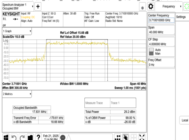
Band77-Part27_20MHz_DFT_s_OFDM_SCS30kHz_16QAM_RB50_0_CH647334
