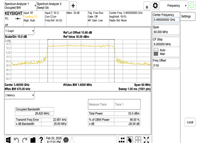
Band77-Part27_30MHz_DFT_s_OFDM_SCS15kHz_QPSK_RB160_0_CH631000
