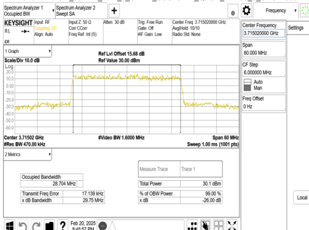
Band77-Part27_30MHz_DFT_s_OFDM_SCS15kHz_QPSK_RB160_0_CH647668
