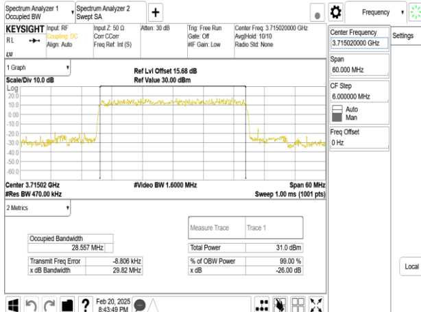
Band77-Part27_30MHz_DFT_s_OFDM_SCS15kHz_BPSK_RB160_0_CH647668
