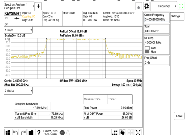
Band77-Part27_20MHz_DFT_s_OFDM_SCS30kHz_BPSK_RB50_0_CH630668
