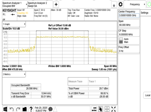
Band77-Part27_30MHz_DFT_s_OFDM_SCS15kHz_256QAM_RB160_0_CH635666
