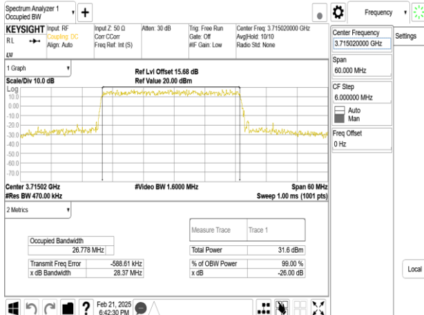
Band77-Part27_30MHz_DFT_s_OFDM_SCS30kHz_QPSK_RB75_0_CH647668
