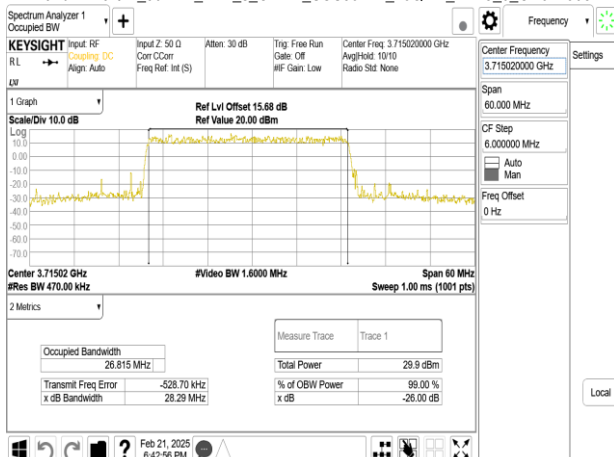
Band77-Part27_30MHz_DFT_s_OFDM_SCS30kHz_16QAM_RB75_0_CH647668
