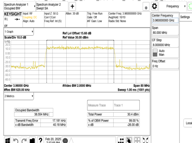
Band77-Part27_40MHz_DFT_s_OFDM_SCS15kHz_QPSK_RB216_0_CH631334
