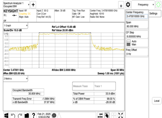
Band77-Part27_40MHz_DFT_s_OFDM_SCS30kHz_BPSK_RB100_0_CH631334
