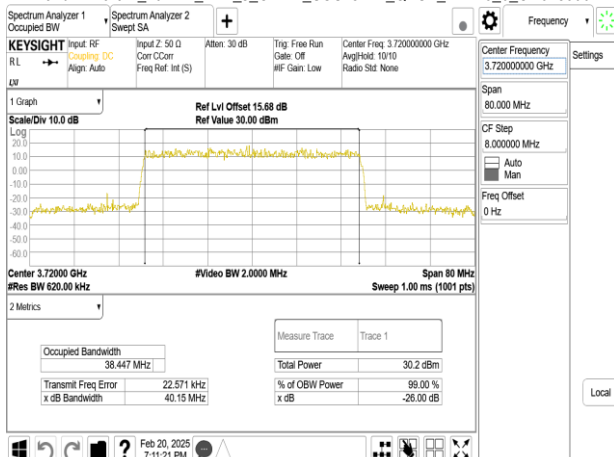
Band77-Part27_40MHz_DFT_s_OFDM_SCS15kHz_QPSK_RB216_0_CH648000
