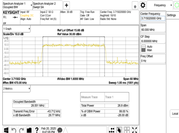
Band77-Part27_30MHz_DFT_s_OFDM_SCS15kHz_256QAM_RB160_0_CH647668
