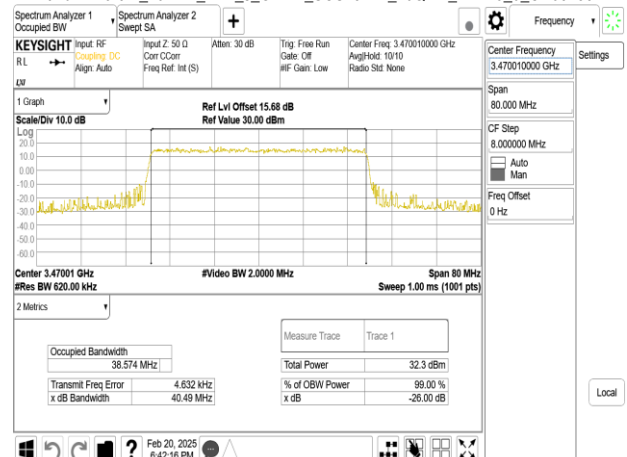
Band77-Part27_40MHz_DFT_s_OFDM_SCS15kHz_16QAM_RB216_0_CH631334
