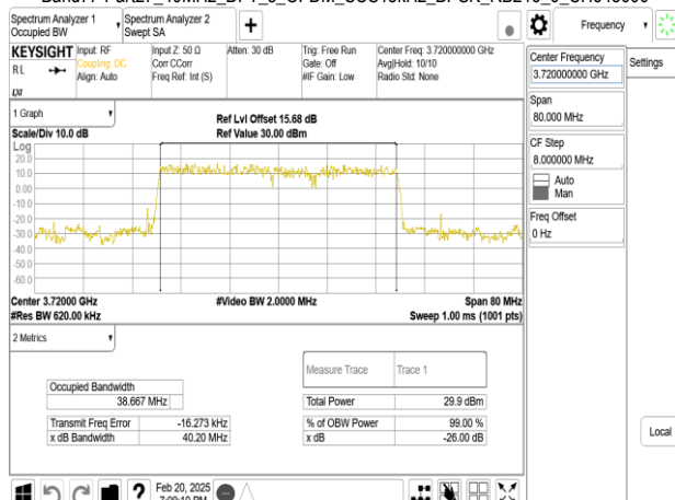
Band77-Part27_40MHz_DFT_s_OFDM_SCS15kHz_BPSK_RB216_0_CH648000
