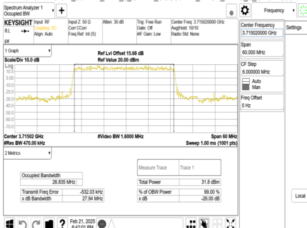
Band77-Part27_30MHz_DFT_s_OFDM_SCS30kHz_BPSK_RB75_0_CH647668
