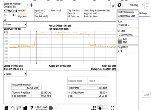
Band77-Part27_60MHz_DFT_s_OFDM_SCS30kHz_16QAM_RB162_0_CH632000
