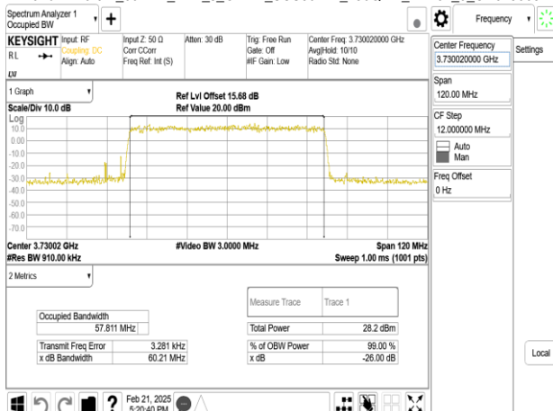
Band77-Part27_60MHz_DFT_s_OFDM_SCS30kHz_256QAM_RB162_0_CH648668
