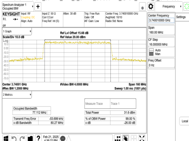
Band77-Part27_80MHz_DFT_s_OFDM_SCS30kHz_QPSK_RB216_0_CH649334
