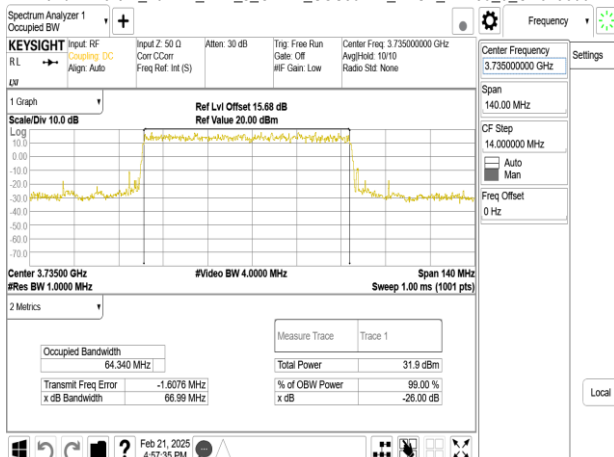
Band77-Part27_70MHz_DFT_s_OFDM_SCS30kHz_BPSK_RB180_0_CH649000
