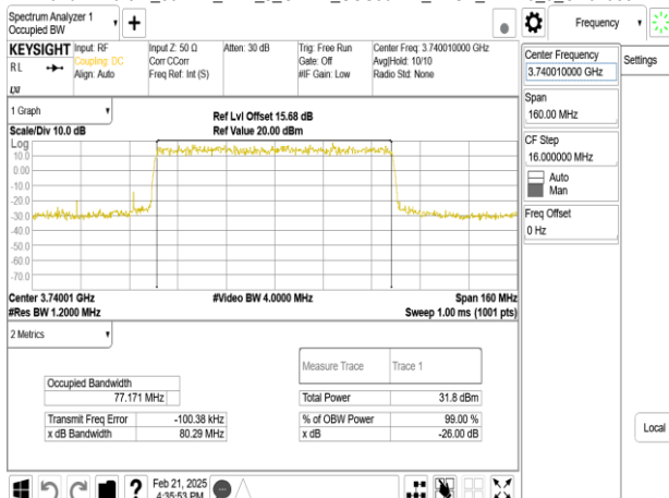
Band77-Part27_80MHz_DFT_s_OFDM_SCS30kHz_BPSK_RB216_0_CH649334
