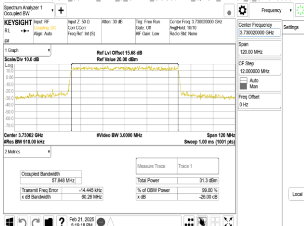
Band77-Part27_60MHz_DFT_s_OFDM_SCS30kHz_QPSK_RB162_0_CH648668
