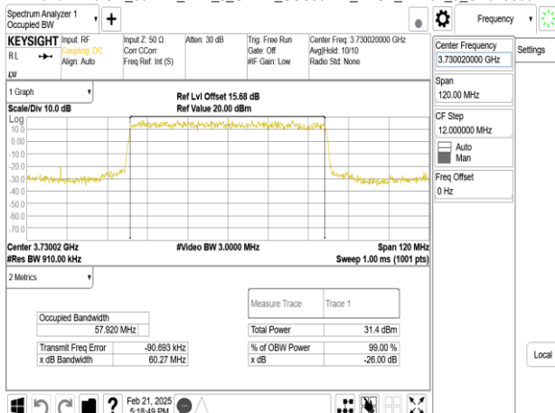
Band77-Part27_60MHz_DFT_s_OFDM_SCS30kHz_BPSK_RB162_0_CH648668
